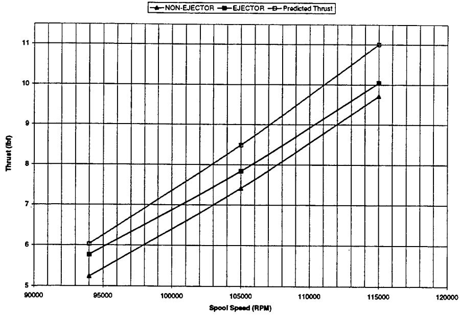
Figure 14 Ejector Performance
