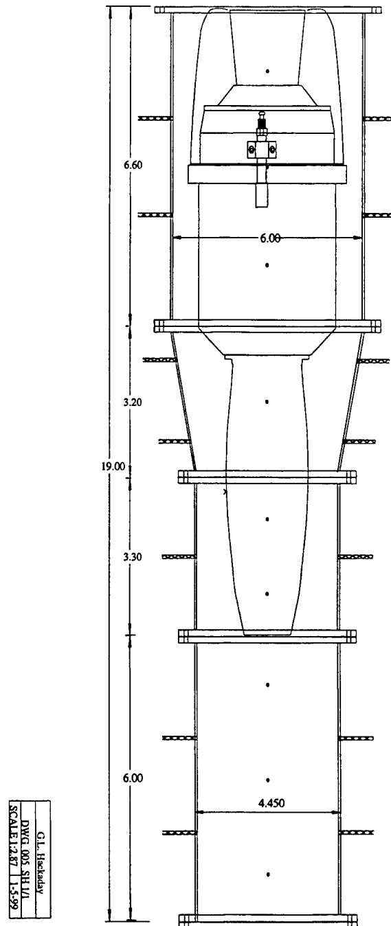
Figure 16 Shroud with Sophia J450 Installed
