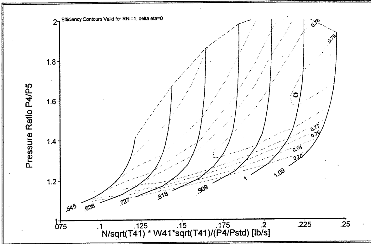
Figure E3. GASTURB Default Turbine Performance Map.
