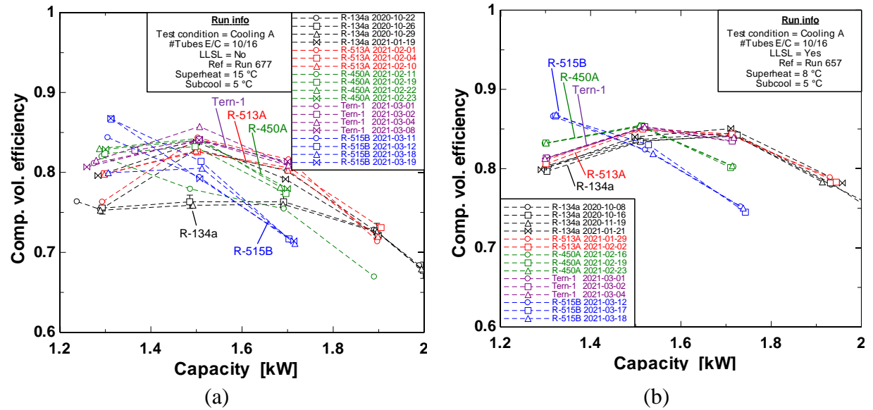
Figure 4.3-7. Compressor volumetric efficiency (a) without LLSL-HX and (b) with LLSL-HX
