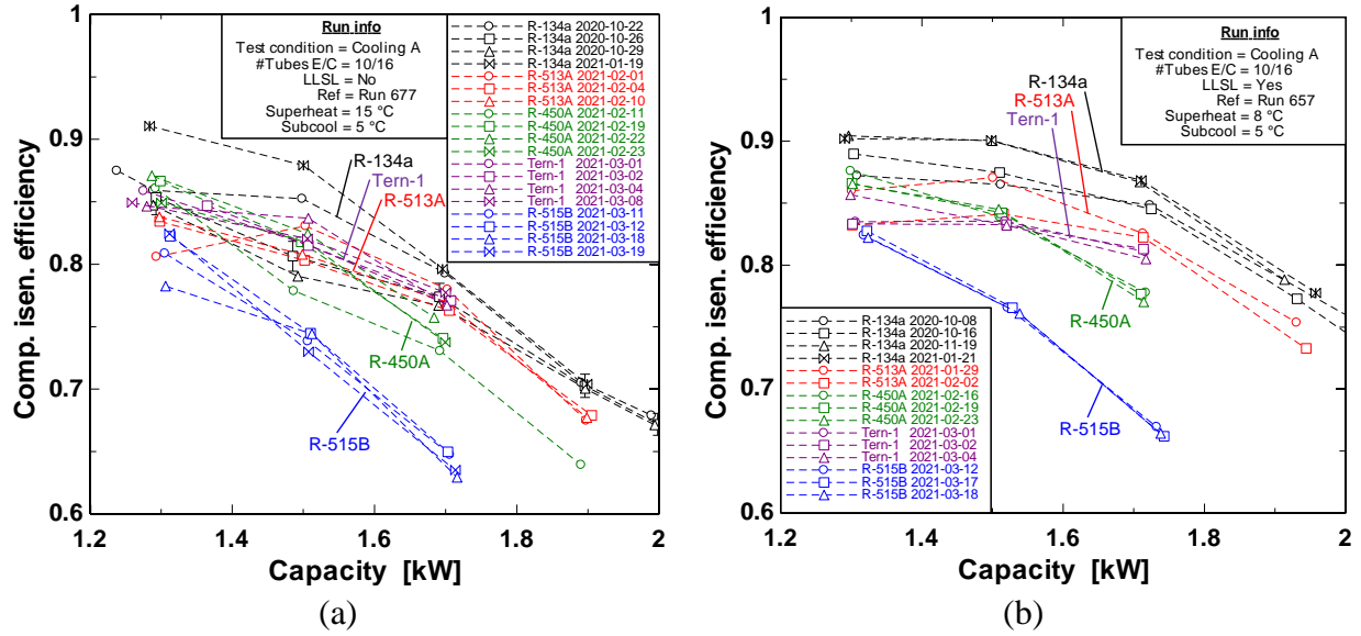
Figure 4.3-6. Compressor isentropic efficiency (a) without LLSL-HX and (b) with LLSL-HX.
