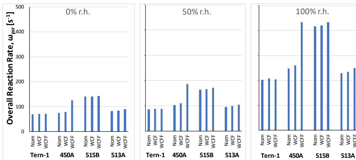
Figure 4.2-12. Peak (over all \phi for each blend) chemical reaction \omega_{psr} for R-513A, R-450A, R-515B and the NIST blend. Data are shown for the Nominal, WCF, and WCFF compositions in air ( T = 296 K) and 0 %, 50 %, and 100 % r.h.
