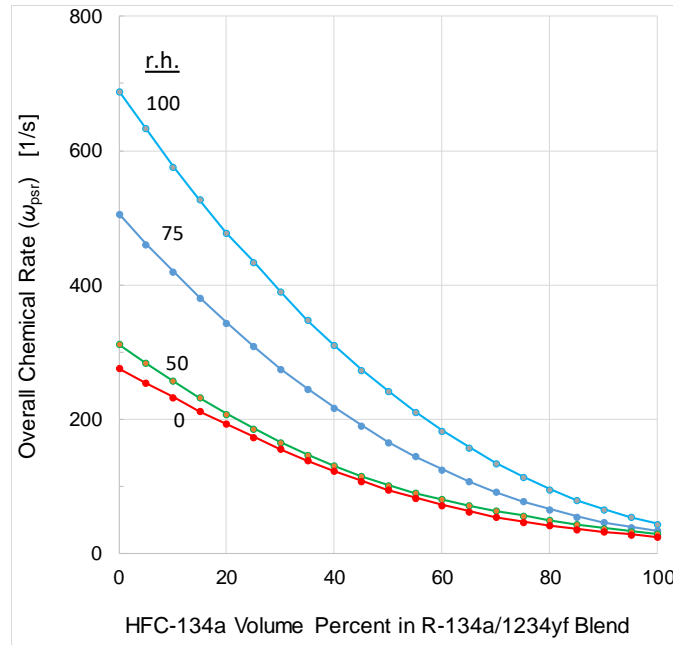
Figure 4.2-10. Peak (over all \phi for each blend) chemical reaction \omega_{\text{psr}} as a function of volume fraction of HFC-134a in the blend of R-1234yf/134a. Individual curves are shown for varying water vapor in the air (0 %, 50 %, 75 % and 100 % r.h.)
