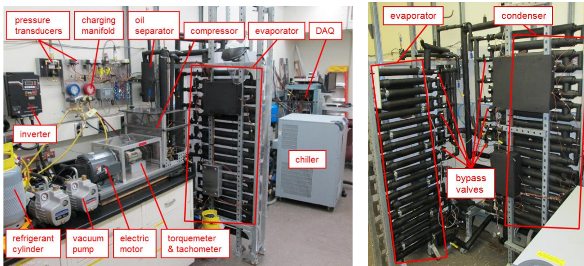
Figure 4.3-1. Photos of the MBHP test apparatus
