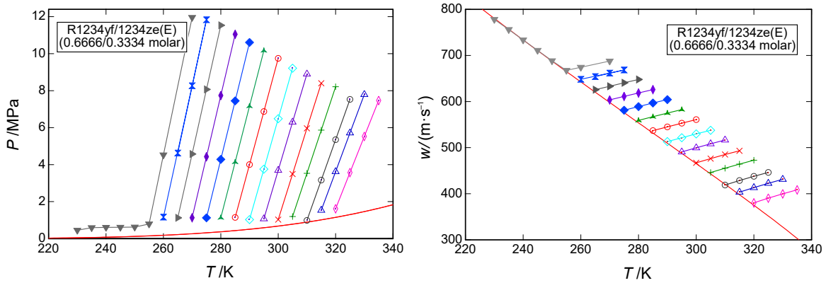
Figure 4.1-2. Measured speed of sound points for the R-1234yf/1234ze(E) blend at a composition of (0.6666/0.3334) mole fraction; left: pressure versus temperature; right: sound speed versus temperature; symbols are measured points and lines connect points along an isochore; red line is phase boundary.
