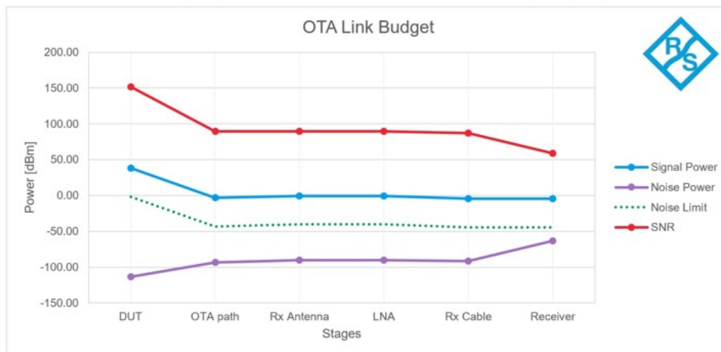
Figure 4.5. Rohde and Schwarz Link Budget Results at 1m
