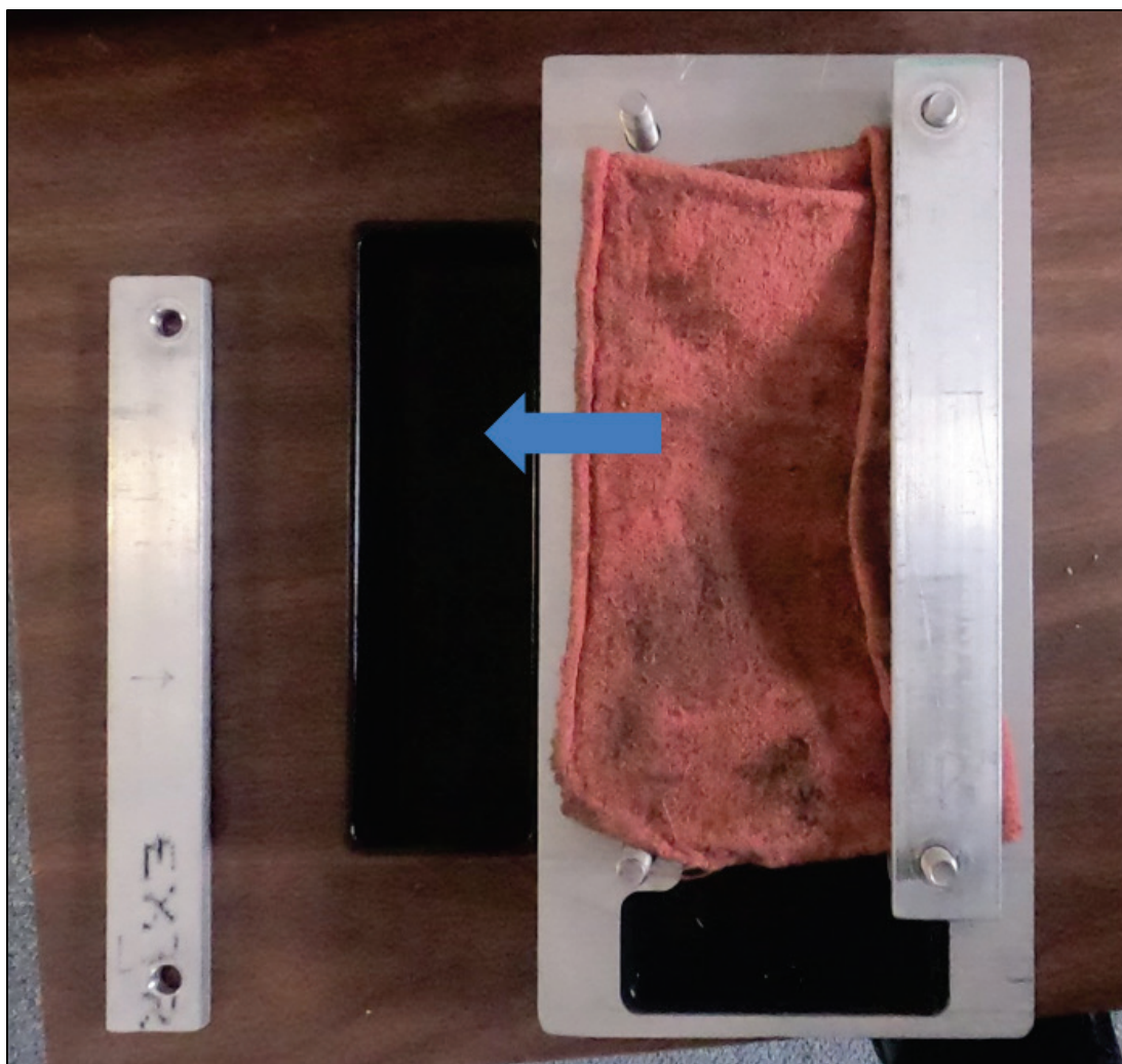
Figure 4. Sampling rig showing a configuration with pig skin for the second stroke with FiberText wipes.
