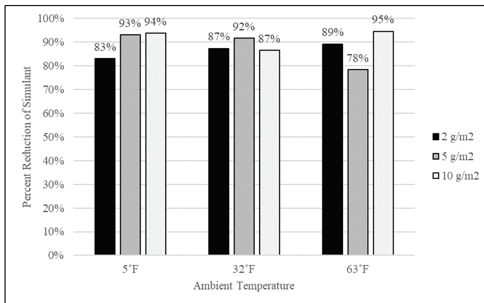
Figure 6. FiberText wipes technology percent reduction of simulant for each ambient testing temperature and starting simulant concentration.
