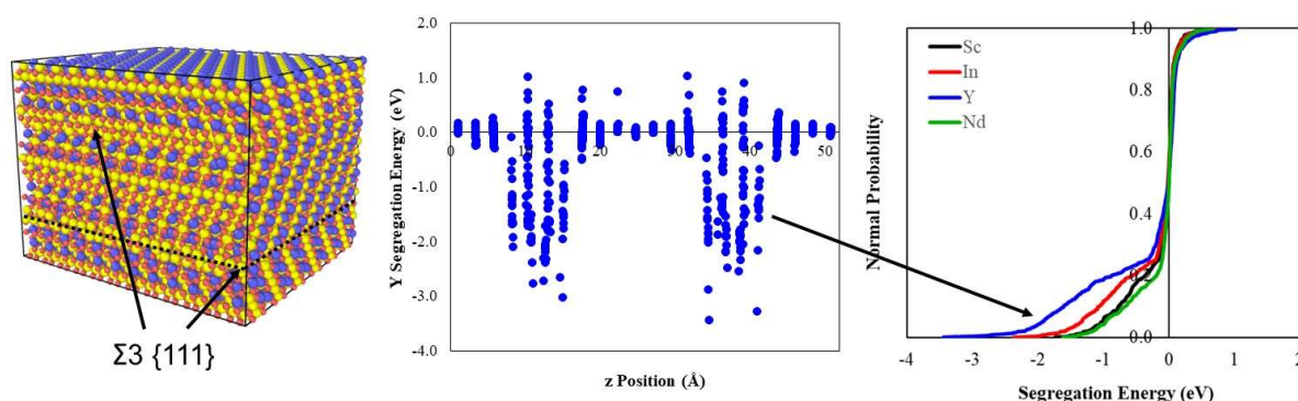
Figure 12. (left) Structure constructed for zinc aluminate with two grain boundaries. (center) Relative potential energy of a zinc aluminate system doped with Y. The dopant was positioned at different locations of the system and the lowest energy positions represent the grain boundary regions created in the modelled system. (right) Four dopants were studied and the segregation energies are shown here.
