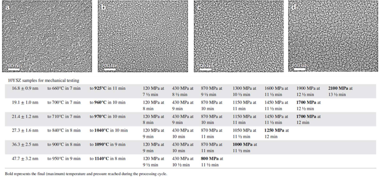
Figure 5. YSZ nanoceramics produced by SPS. SEM images on the top and a table describing the sintering protocols developed after extensive experimental grid design.
