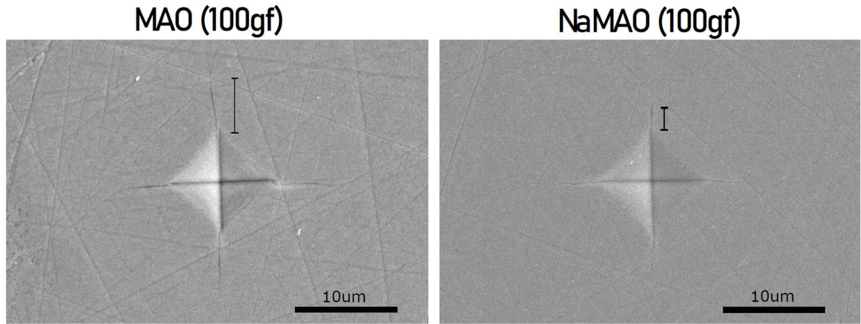
Figure 2. \text{MgAl}_2\text{O}_4 (MAO) and Na-doped \text{MgAl}_2\text{O}_4 (NaMAO) indicating distinct edge cracks supporting Na doped samples show increased toughness. K1C is 3.57 for MAO and 4.45 for NaMAO.
