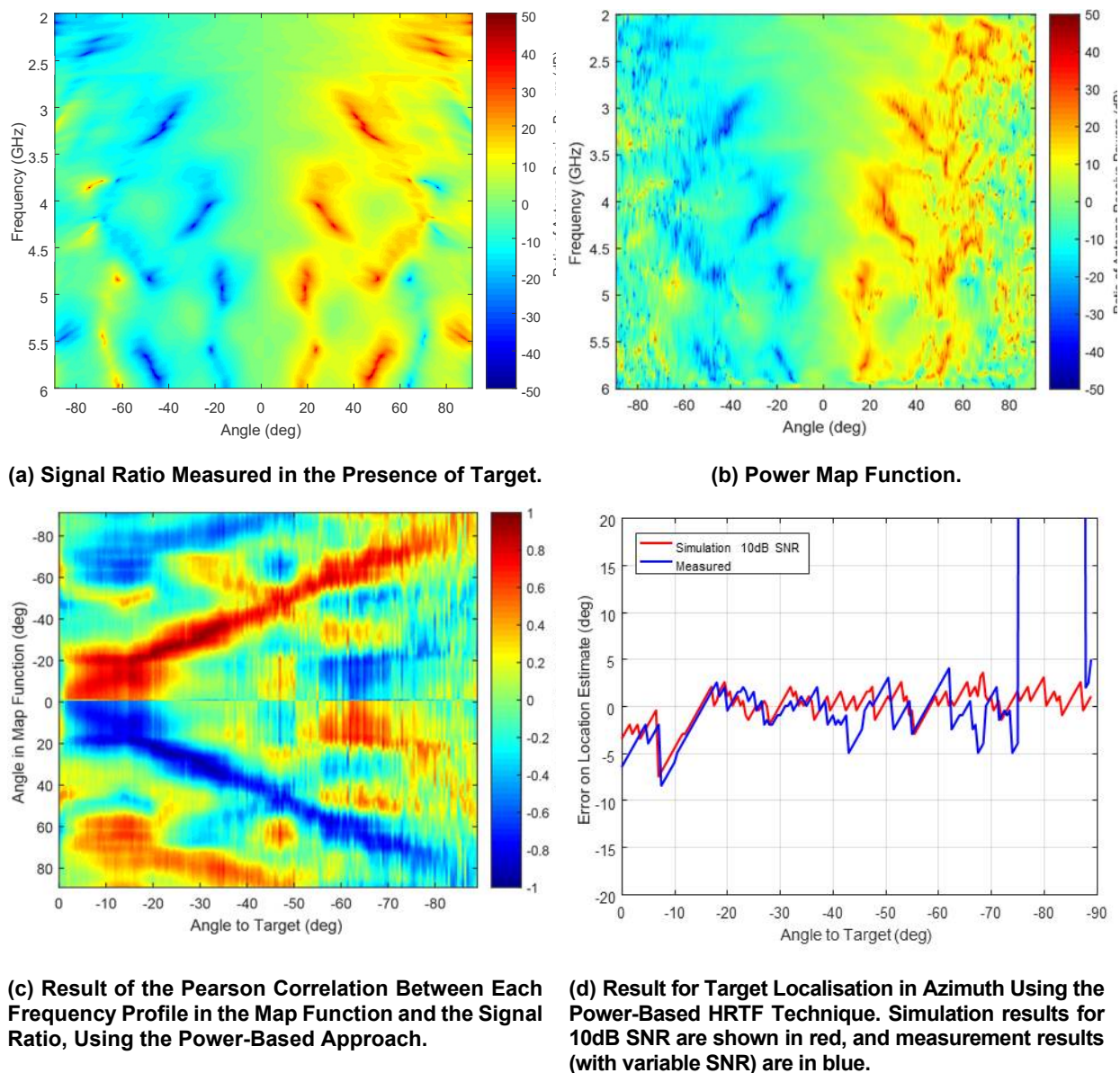
Figure 4-11: Results for the Power-Based Approach.
