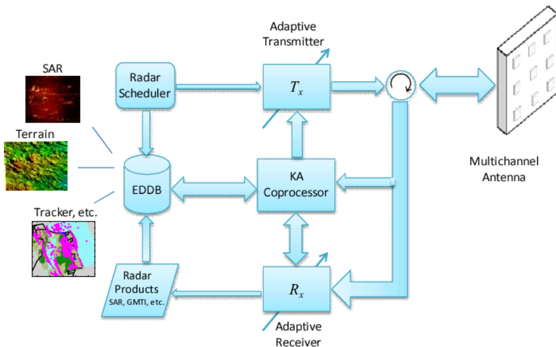
Figure 3-1: Cognitive Radar Architecture Proposed by Guerçi [27].
