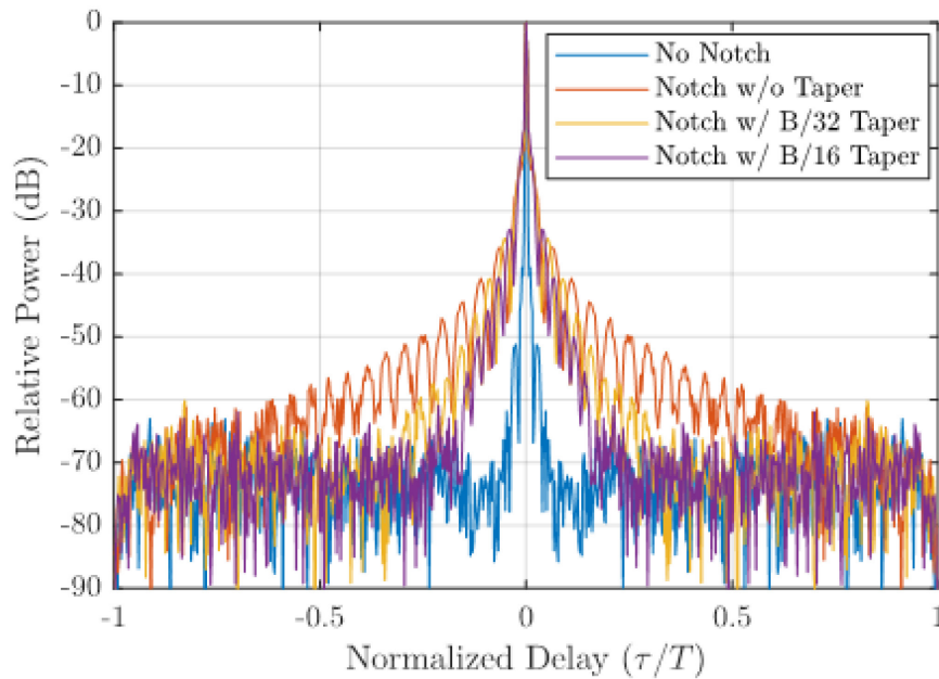
Figure 5-3: Measured Aggregate Autocorrelation (for 2500 Unique FM Noise Waveforms) Comparing Spectral Notch Tapering to the Case Without Tapering and the Absence of a Notch [148].
