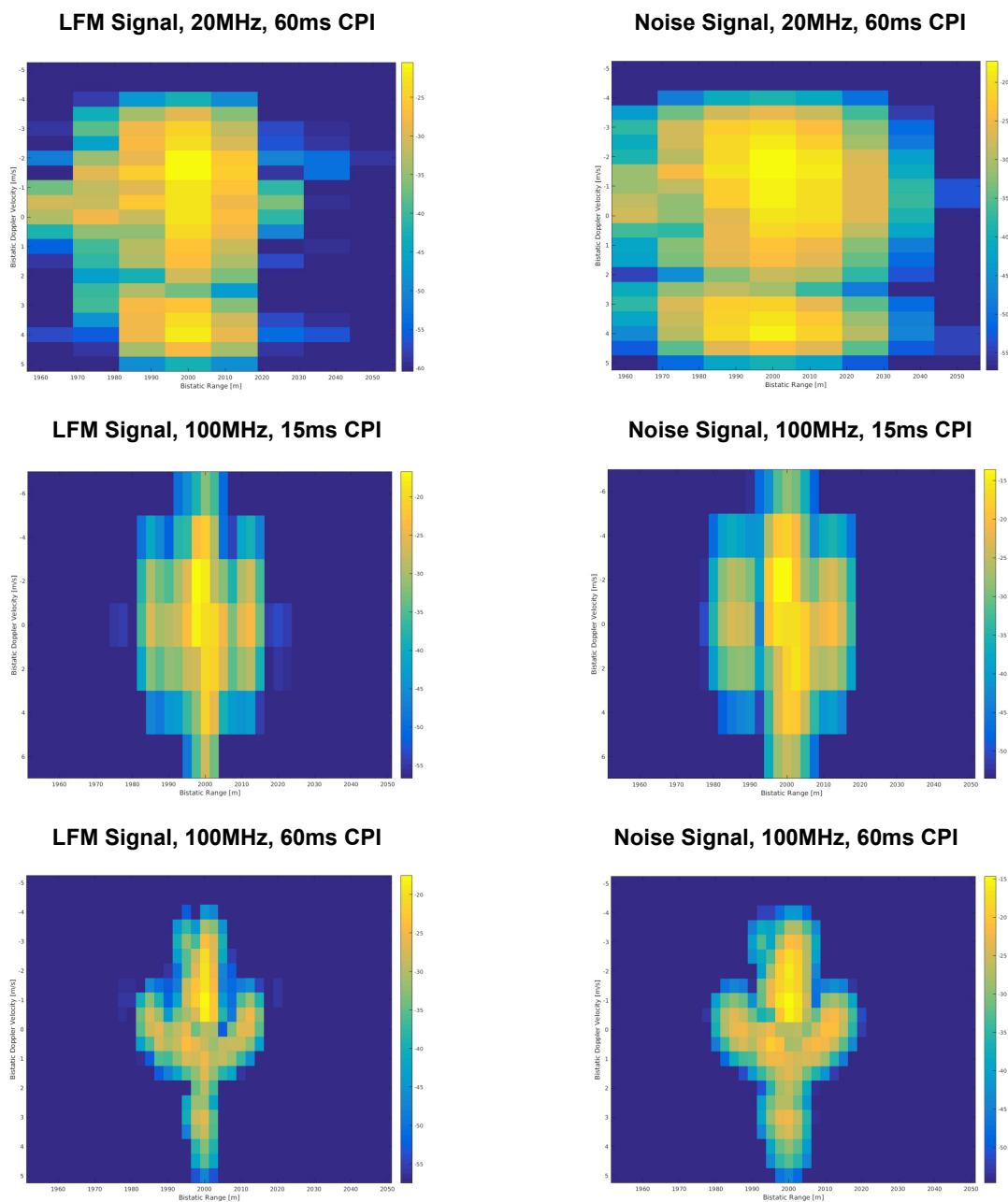
Figure 6-11: Example ISAR Images Depending on Signal Types and their Parameters.
