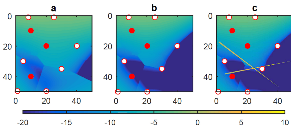
Figure 6-4: Impact of Dynamic and Static Spectrum Map Components [172]. Red and white circles are surveillance and ordinary sensors. (a) Average measurement results with Universal Kriging method. (b) Impact of strong temporal peaks are removed. (c) The scanning radars are modeled based on surveillance sensor parameters estimation.
