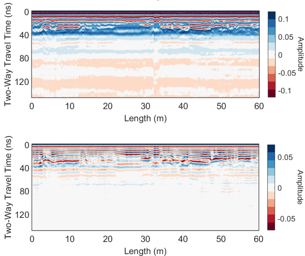
Figure 15. Top , duplicate of profile shown in Fig. 14 b . Bottom , top profile with data filtering applied.
