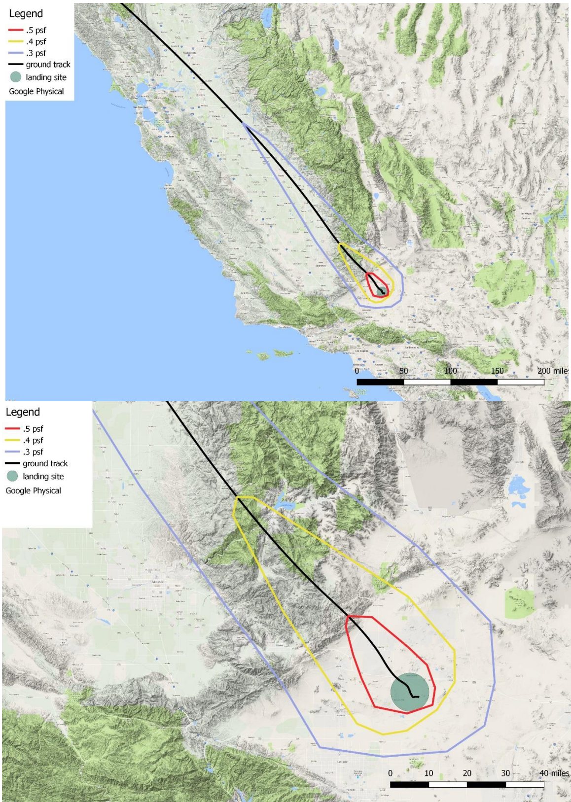
Figure D- 4: EAFB Ascending Node Trajectory Sonic Boom Footprint
