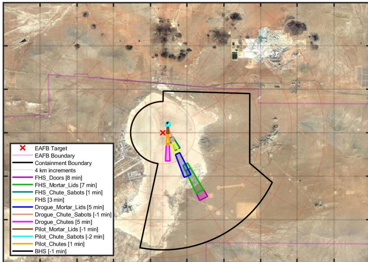
Figure 2-4: Example Output from Jettisoned Parts Landing Area Prediction Model
