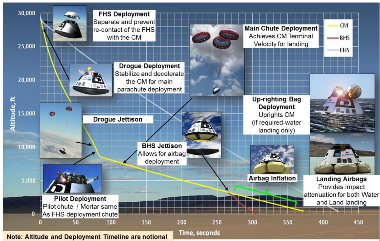
Figure 2-5: Starliner Landing Sequence
