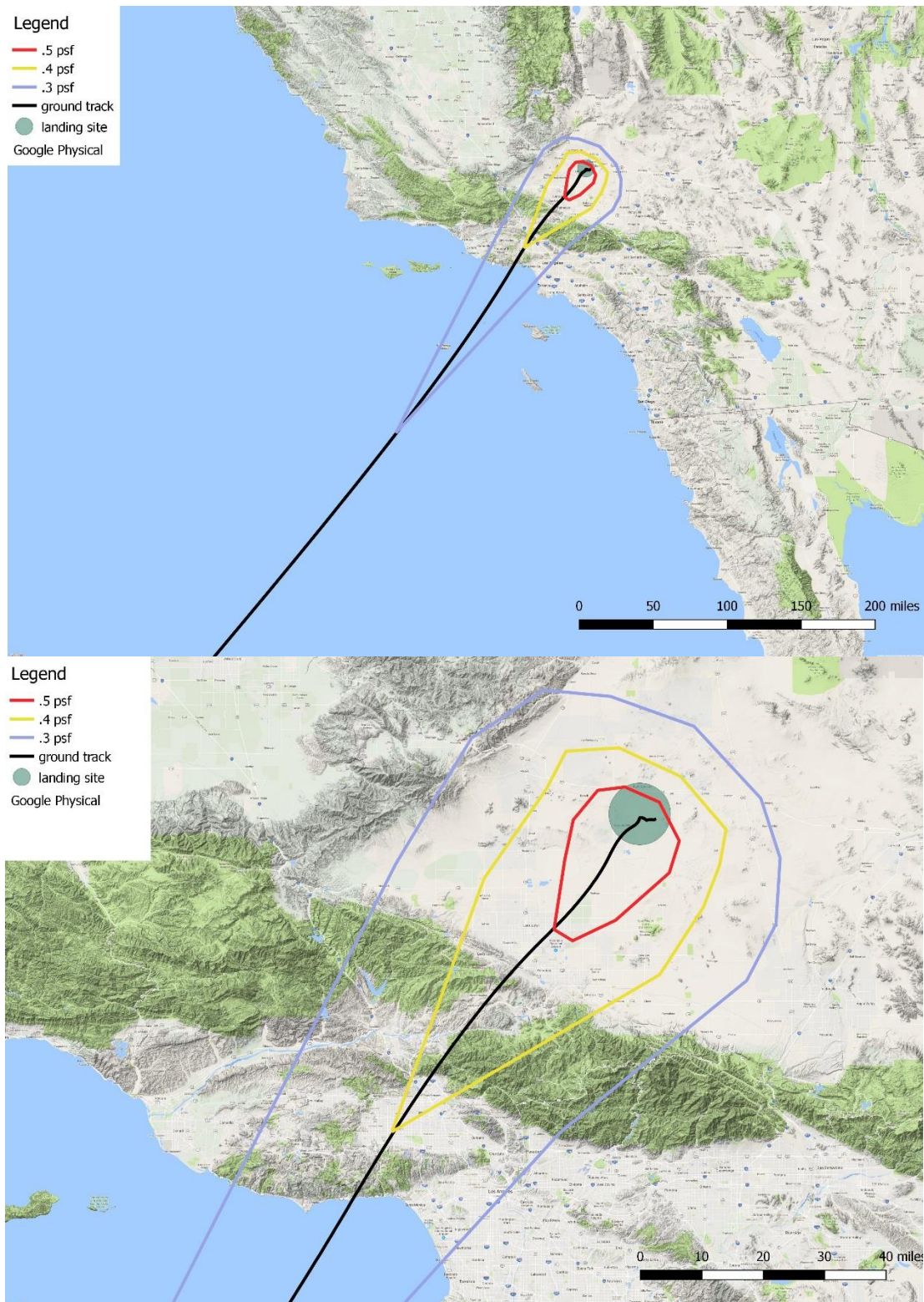
Figure D- 2: EAFB Descending Node Trajectory Sonic Boom Footprint
