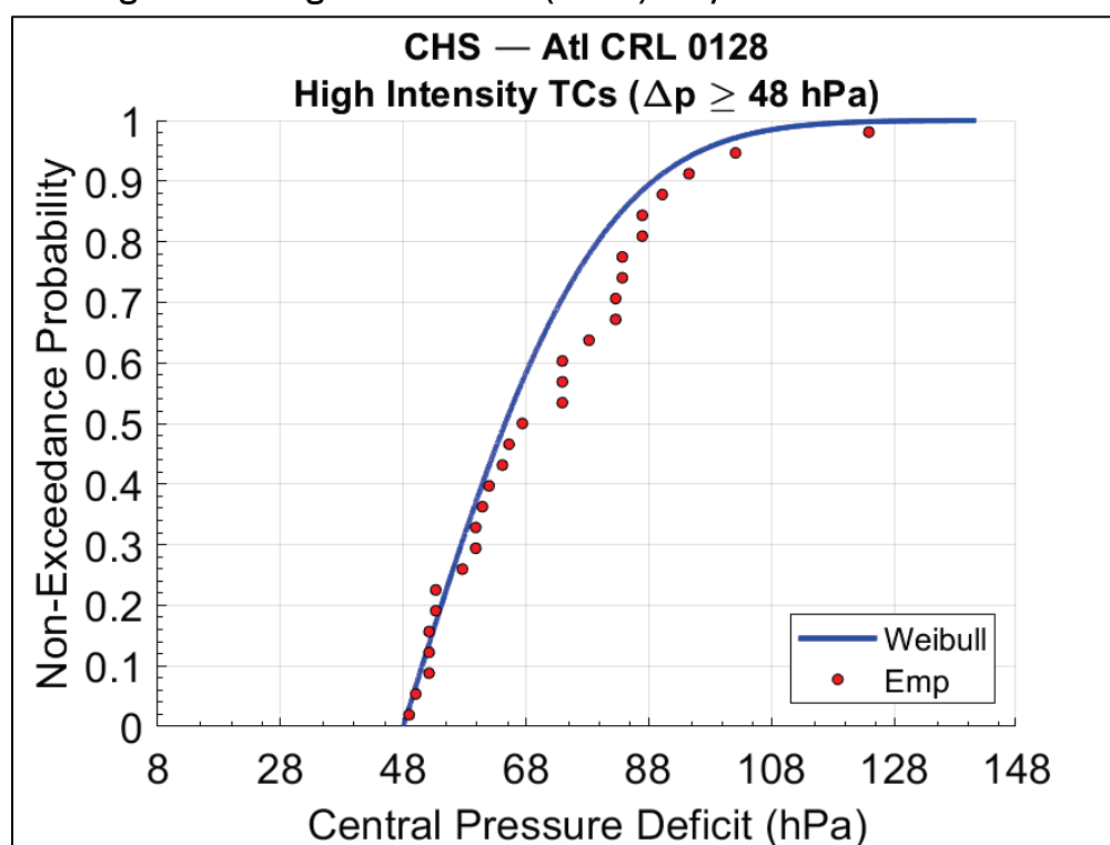
Figure 4-3. Marginal distribution (DTWD) of \Delta p for HI TCs at CRL 128.
