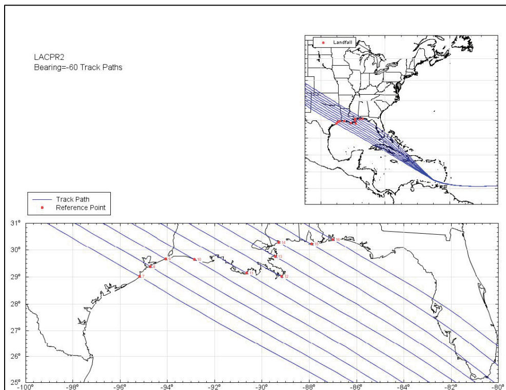
Figure 5-3. JPM heading -60^\circ track paths.
