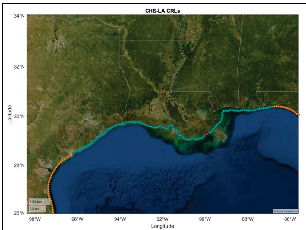
Figure 3-6. CRLs ( blue ) used in the PCHA for the CHS-LA study area.
