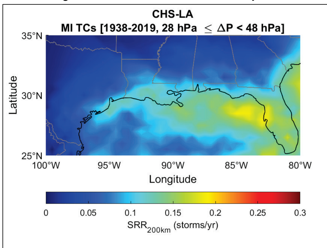
Figure 3-11. SRR for MI TCs within the CHS-LA study area.
