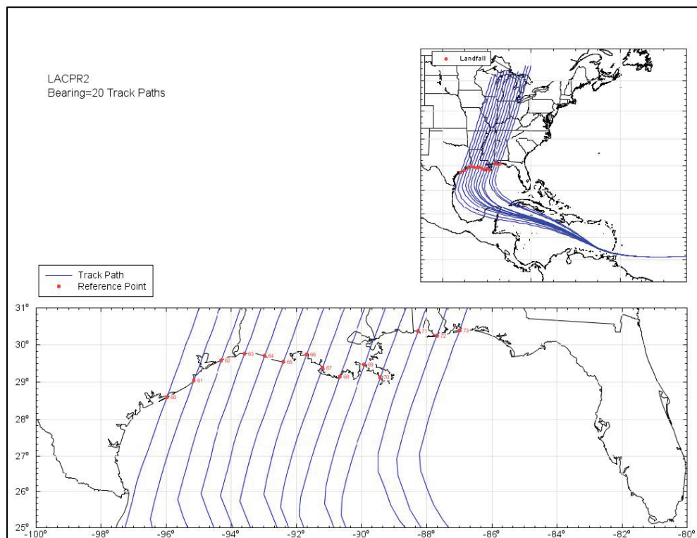
Figure 5-7. JPM heading 20° track paths.
