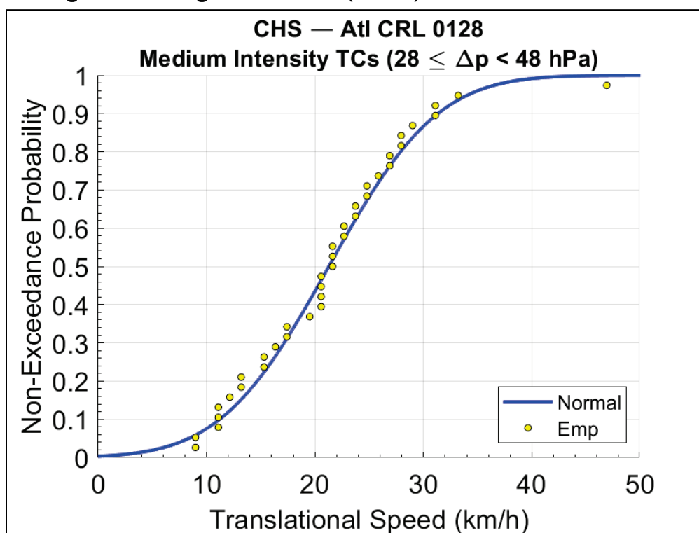
Figure 4-10. Marginal distribution (normal) of V_t for MI TCs at CRL 128.
