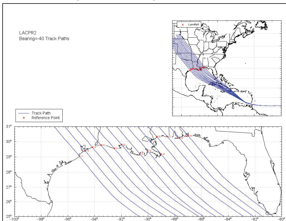
Figure 5-4. JPM heading -40^\circ track paths.
