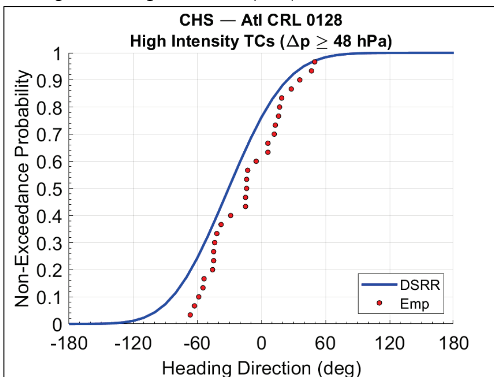
Figure 4-12. Marginal distribution (DSRR) of \theta for HI TCs at CRL 128.
