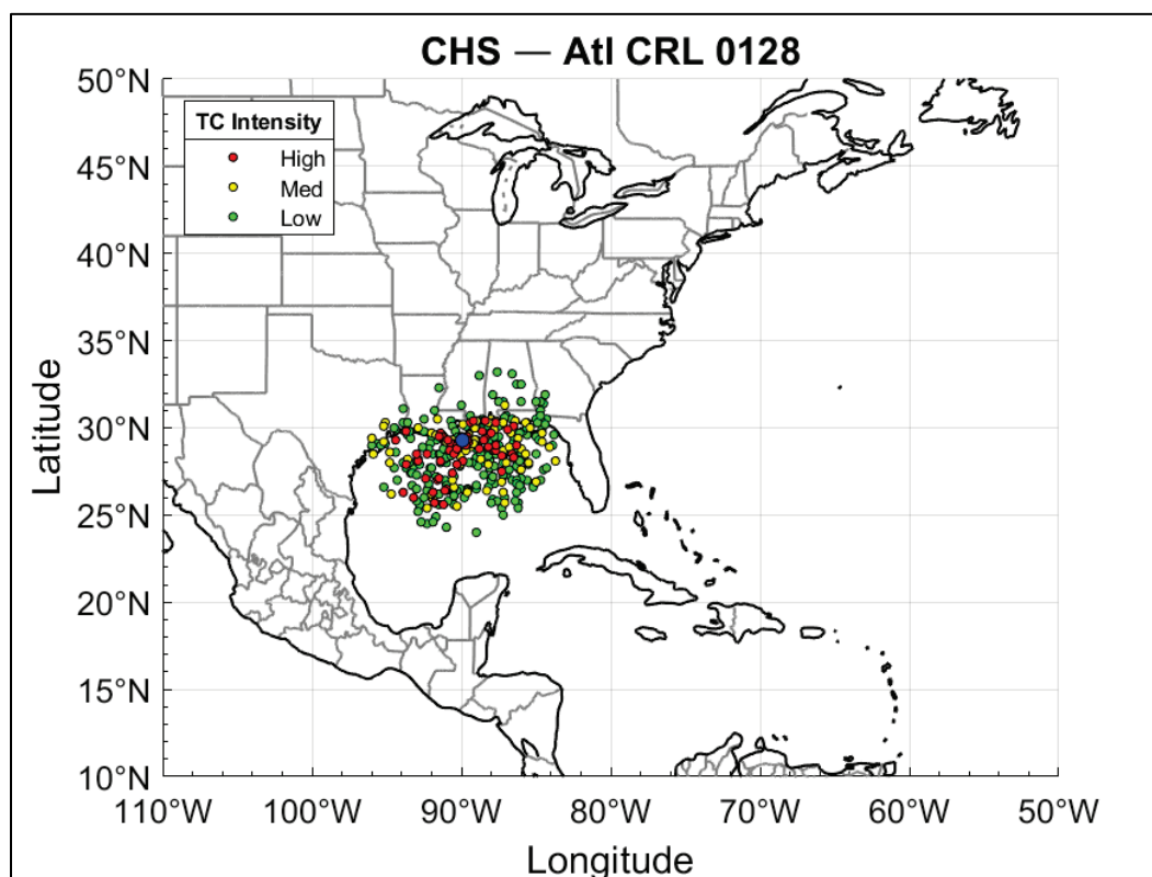
Figure 3-7. Optimal sampling locations of selected historical TCs within 600 km of CRL 128.
