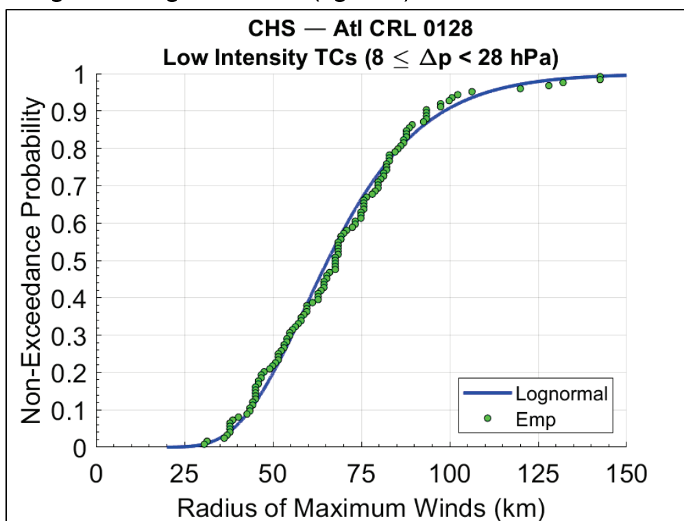
Figure 4-8. Marginal distribution (lognormal) of R_{max} for LI TCs at CRL 128.
