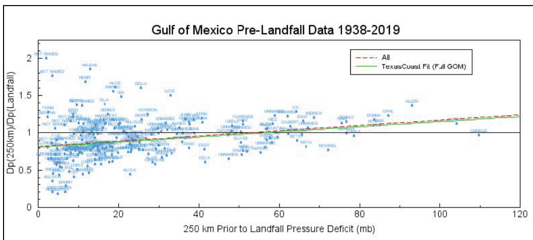
Figure 5-11. Linear fit to ratio of pressure deficit at 250 km and landfall as a function of pressure deficit at 250 km. Ratio of > 1 indicates storms weakening as they approach landfall, ratio < 1 are storms strengthening towards landfall. Relationship applied in Texas Coast/SACS study shown in green.
