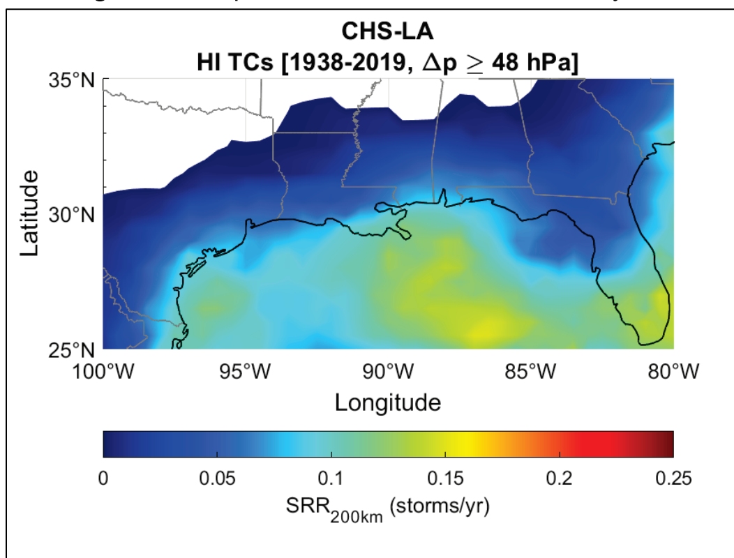
Figure 3-10. Geospatial SRR for HI TCs within the CHS-LA study area.
