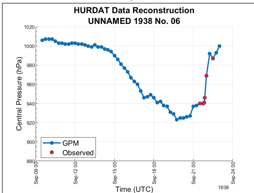
Figure 3-1. Reconstruction of \Delta p for a 1938 historical TC using metamodeling techniques.
