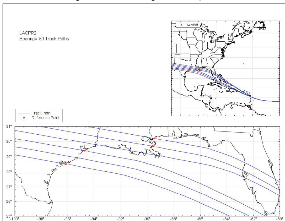
Figure 5-2. JPM heading -80^\circ track paths.
