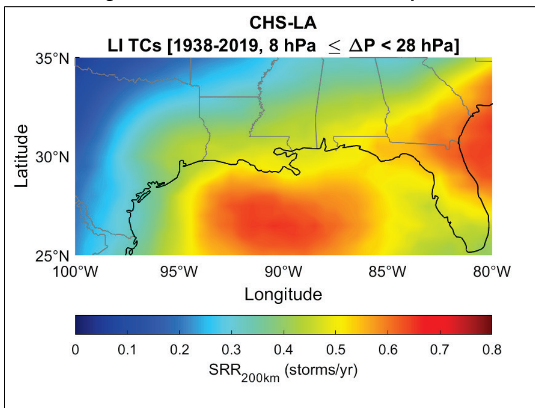
Figure 3-12. SRR for LI TCs within the CHS-LA study area.
