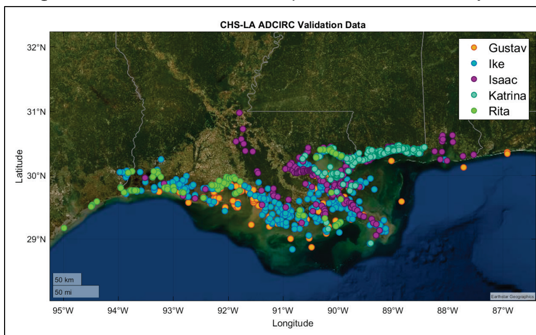
Figure C-1. Distribution of validation data points within the CHS-LA study area.
