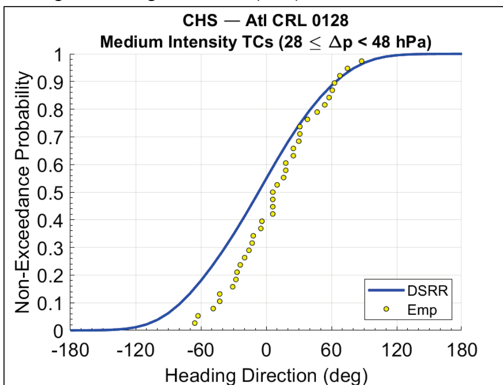
Figure 4-13. Marginal distribution (DSRR) of \theta for MI TCs at CRL 128.
