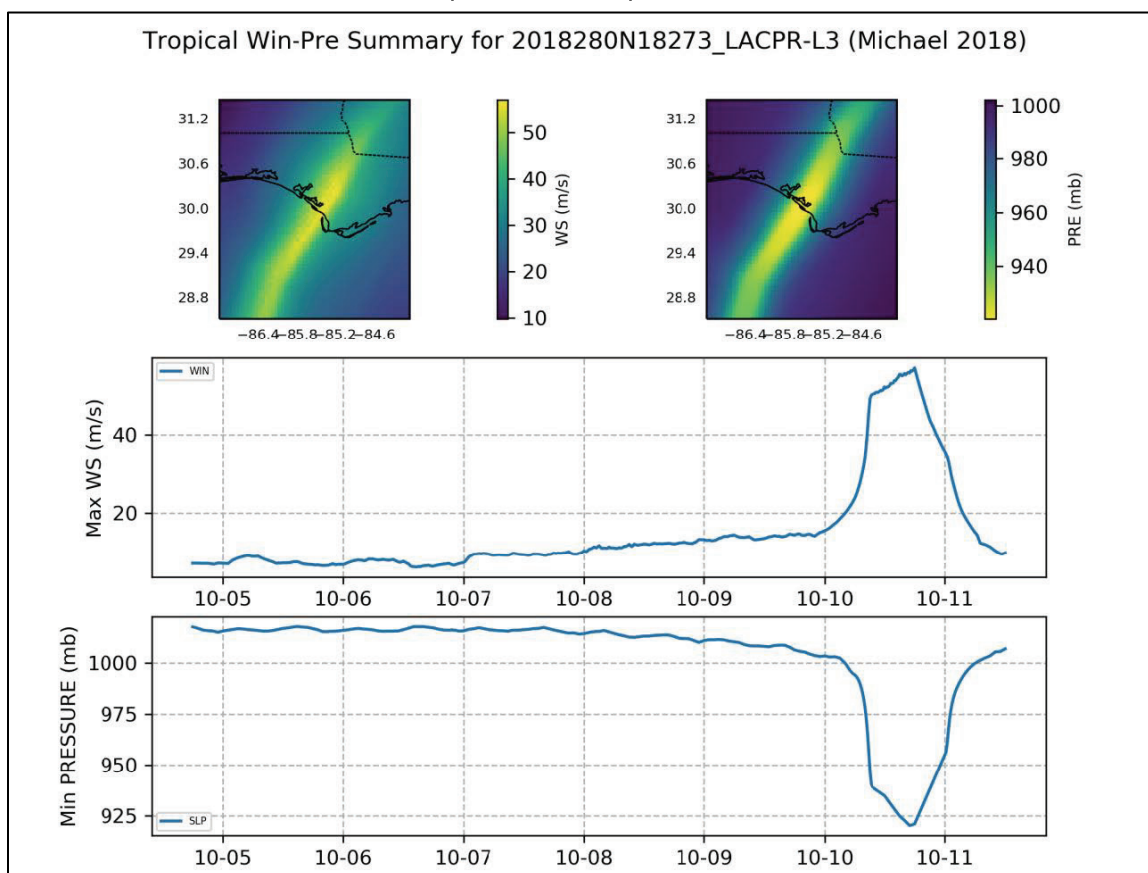
Figure 5-17. Summary of winds and pressures during 2018280N18273 (Michael 2018) for L3.
