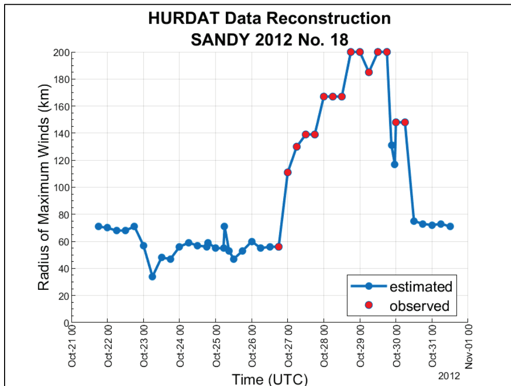
Figure 3-4. Reconstruction of R_{max} for Hurricane Sandy using metamodeling techniques.
