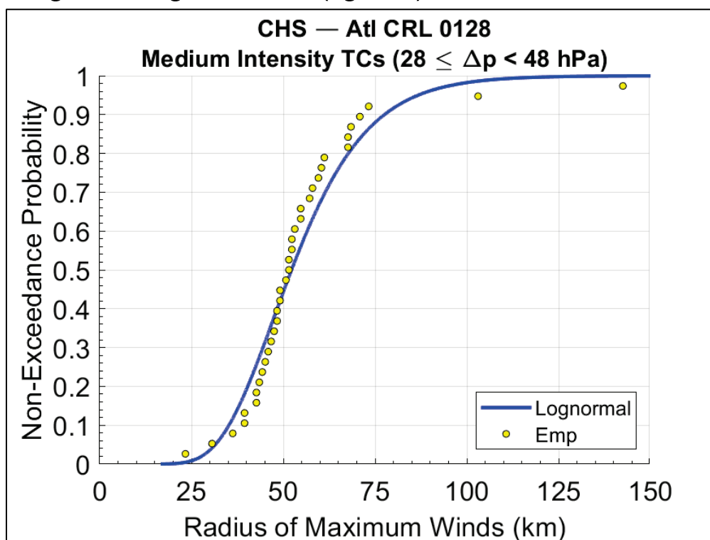
Figure 4-7. Marginal distribution (lognormal) of R_{max} for MI TCs at CRL 128.
