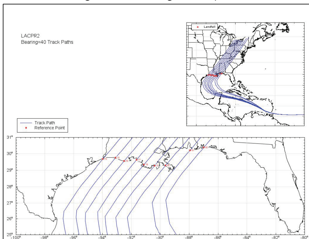
Figure 5-8. JPM heading 40° track paths.
