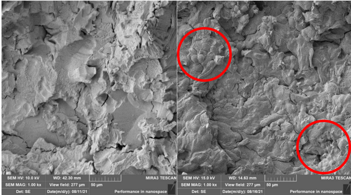
Figure 4.16 70Mo-25W-5Re fracture surface of the 100 mm/s sample (left) and the 600 mm/s sample (right) at 1.0kx magnification highlighting unmelted particles
