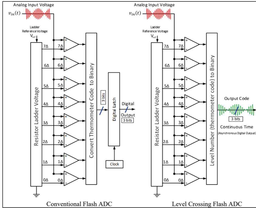
Fig. 6 Conventional flash ADC and CT level-crossing flash ADC. CT level-crossing flash ADC has the same structure as a conventional flash without the clocked latch. The CT flash also is more energy efficient.
