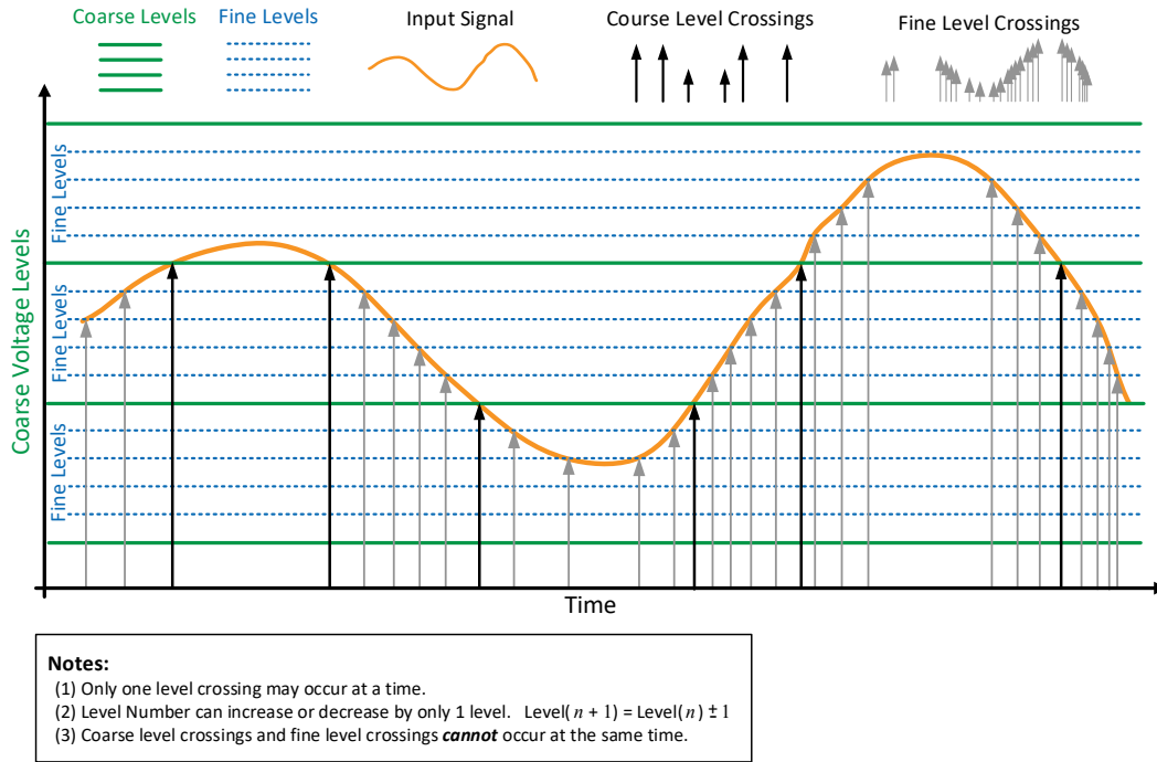
Fig. 30 The operation of a continuous-time pipeline level-crossing ADC. The first pipeline stage provides the coarse-level output. The second pipeline stage has its four fine levels inside the coarse voltage levels. This way there is no overlap between the coarse and fine levels. This ensures that only one level can be crossed at a time for all pipeline stages. The amplitude scaling for the coarse and fine voltage levels is a key feature of this invention. By only allowing for a single level to be crossed at a time, the present invention overcomes timing and amplitude accuracy errors present in conventional pipeline flash ADCs.
