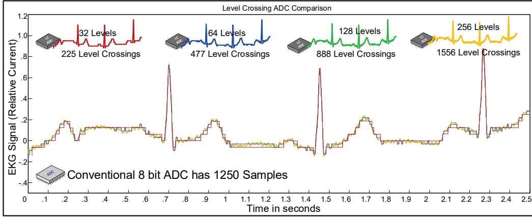
Fig. 22 Conventional 8-bit ADC has 1250 samples, f_s = 500 Hz. Tsividis 2 shows a level-crossing ADC has about 20 dB better SNR compared to an “equivalent” conventional ADC. To achieve an extra 20-dB SNR, a conventional ADC requires an oversample factor of OSR = 100 to achieve a 10\log(100) = 20 -dB SNR improvement. The total number of samples is 1250 \cdot 100 = 125,000 which is much greater than 1556 for a level-crossing ADC.
