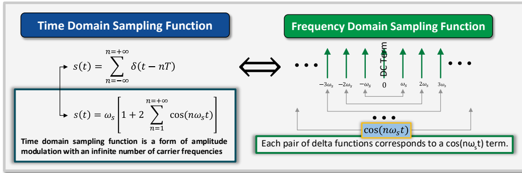
Fig. 10 Time domain sampling function is an infinite sum of cosine terms. By grouping pairs of delta functions in the frequency domain, an infinite sum of cosine terms is found. The infinite sum helps explain the origins of frequency aliasing.
