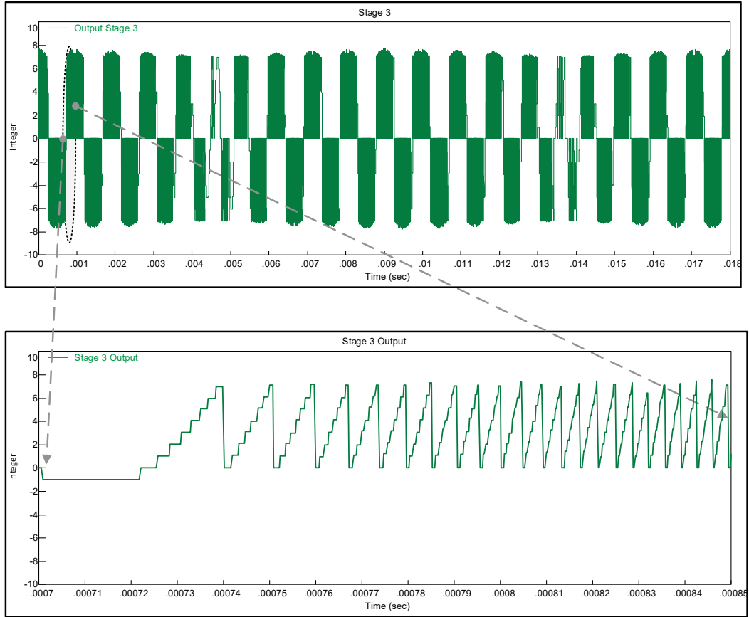
Fig. 36 Simulated pipeline stage 3 output for a three-stage pipeline level-crossing ADC
