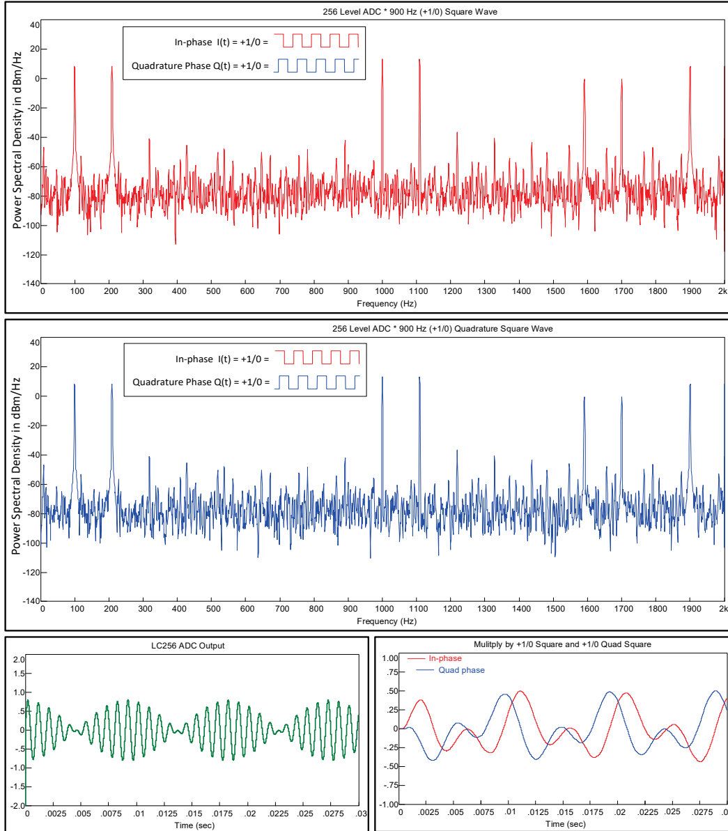
Fig. 46 Software-reconfigurable radio simulation using a +1/0 in-phase and quadrature-phase square waves. A 256-level, level-crossing ADC was used for the simulations. Input signal is 1.0 and 1.11 kHz. I/Q modulator is 0.9-kHz quadrature square waves with +1/0 amplitudes. Frequency down-conversion for I/Q channels are shown. There are tones present at 100 and 211 Hz. There are image frequencies at 1.0, 1.1, 1.6, and 1.7 kHz. Bottom graphs are level-crossing ADC time domain waveforms and I/Q channels.
