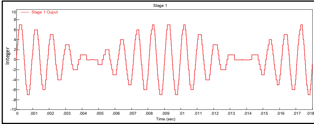
Fig. 34 Simulated pipeline stage 1 output for a three-stage pipeline level-crossing ADC
