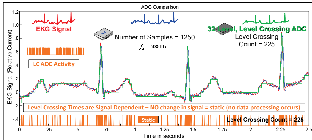
Fig. 21 Conventional ADC and level-crossing ADC for ECG data. For a conventional ADC, 1250 samples are required. For a 32-level, level-crossing ADC, only 225 samples are required.
