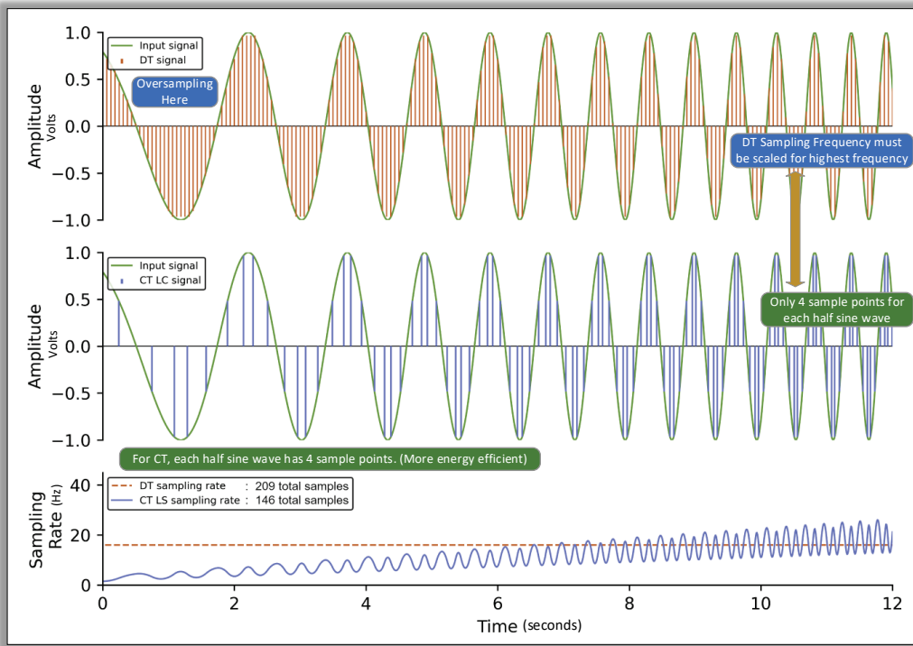
Fig. 5 Comparison of conventional DSP to CT for frequency chirp signal. For continuous time, the chirp signal has a constant number of sample points per half sine wave cycle. Frequency chirp will be a useful waveform for testing continuous-time systems.
