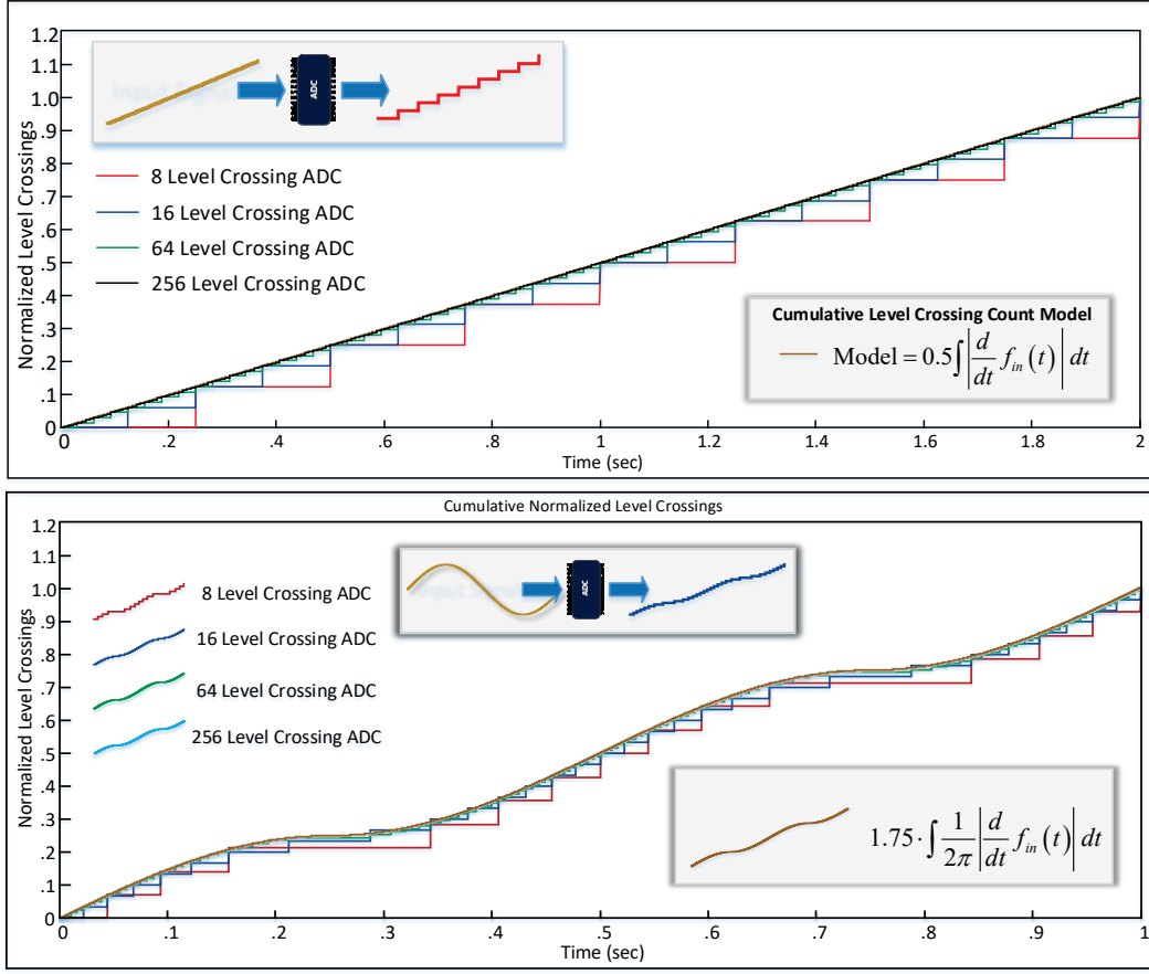
Fig. 24 For level-crossing analog-to-digital conversion, the level-crossing time differences, t_k - t_{k-1} , are inversely proportional to the slope of the input signal. The effective sampling frequency is proportional to the slope of the input signal. Cumulative level-crossing count is proportional to the integral of the input signal's slope. The top graph shows a ramp input signal, and the bottom graph shows a sine wave input signal. Level-crossing times are shown in Fig. 23.
