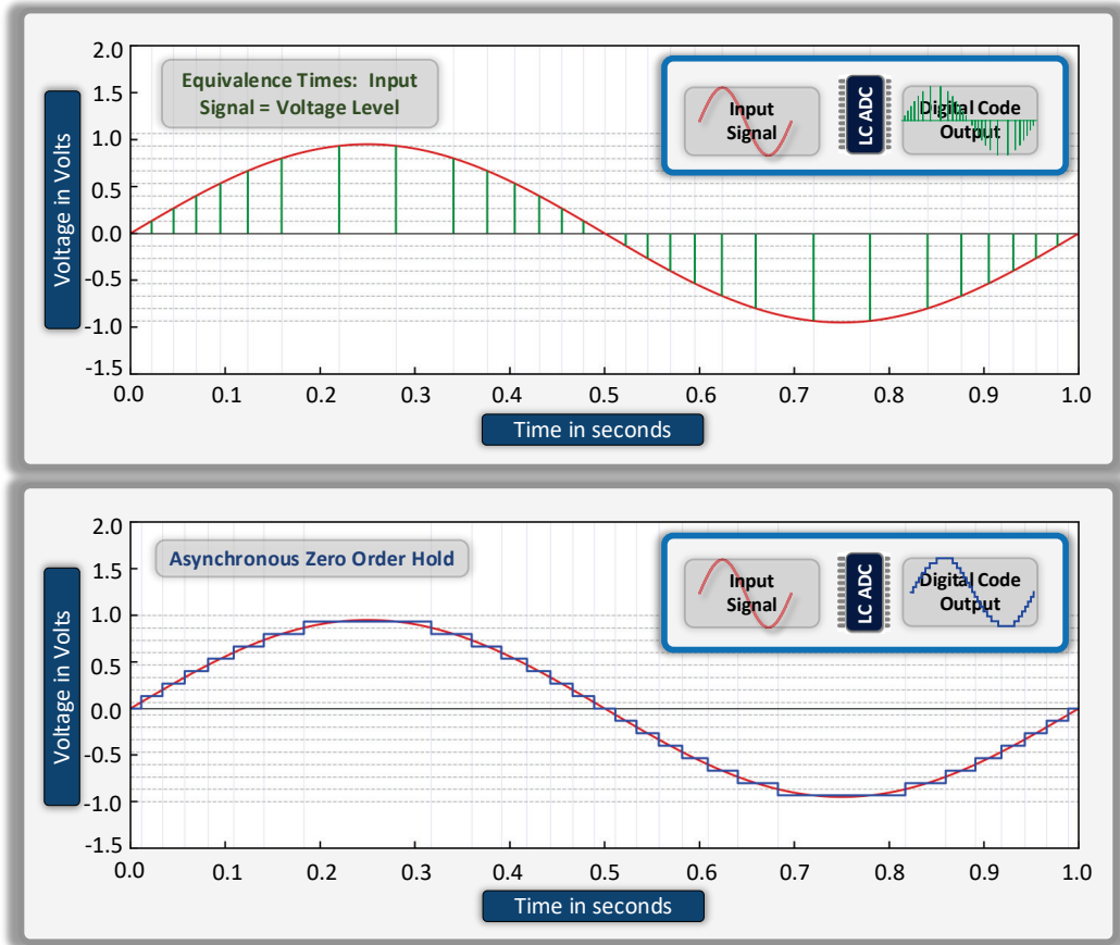
Fig. 23 Level-crossing analog-to-digital conversion. A level-crossing ADC creates a pulse when the input signal exactly equals a discrete voltage level. The equivalence times, t_k , occur when the input signal exactly equals a voltage level. The pulse amplitude is equal to the voltage level crossed. An asynchronous (nonuniform) zero-order hold will keep the output value constant until the next level crossing occurs.
