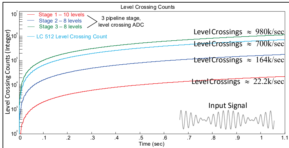
Fig. 37 Comparison of the number of level crossings for each stage in a three-stage pipeline level-crossing ADC to a 512 level-crossing ADC. Figures 33–36 show the stage activity for a two-tone test signal. Stage 1 has a level-crossing activity of 22.2k levels/s. Stage 1 is nearly static compared to stage 3 with 980k levels/s. The light blue line shows that the level-crossing activity for a 512-level ADC is slightly less than stage 3 at 700k levels/s.
