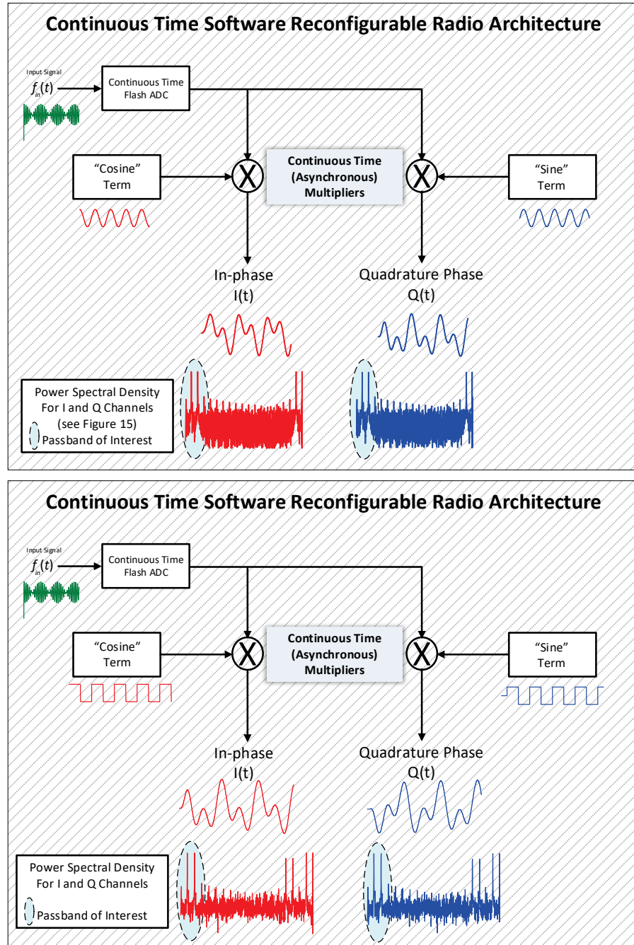
Fig. 43 Continuous-time software-reconfigurable radio simulation. Multipliers are continuous time (asynchronous digital, not analog). Simulations for cosine/sine down-conversion and in-phase square wave and quadrature-phase square wave down-conversion are shown. Both architectures have similar power spectral density graphs. The passband of interest, containing the frequency terms 100 Hz and 211 Hz, is highlighted.
