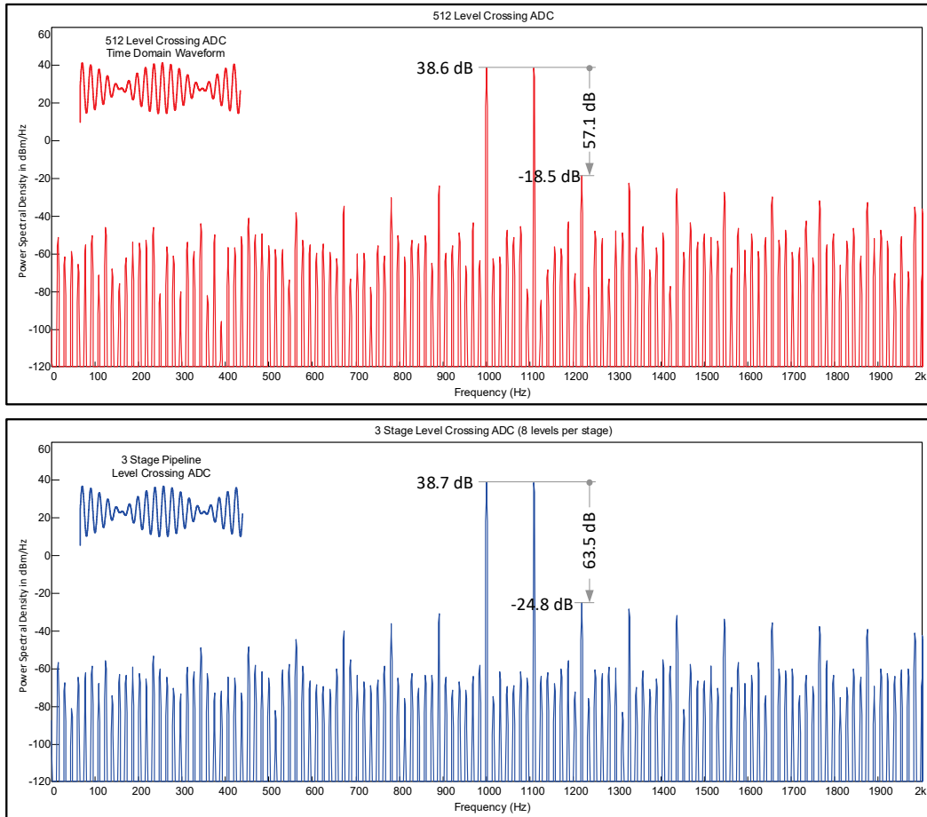
Fig. 38 Comparison of the present continuous-time three-stage pipeline level-crossing ADC to a conventional 512 level-crossing ADC. The present invention provides better intermodulation distortion compared to a conventional level-crossing ADC. The three-stage level-crossing ADC only requires 26 comparators compared to 512 for the 512 level-crossing ADC.
