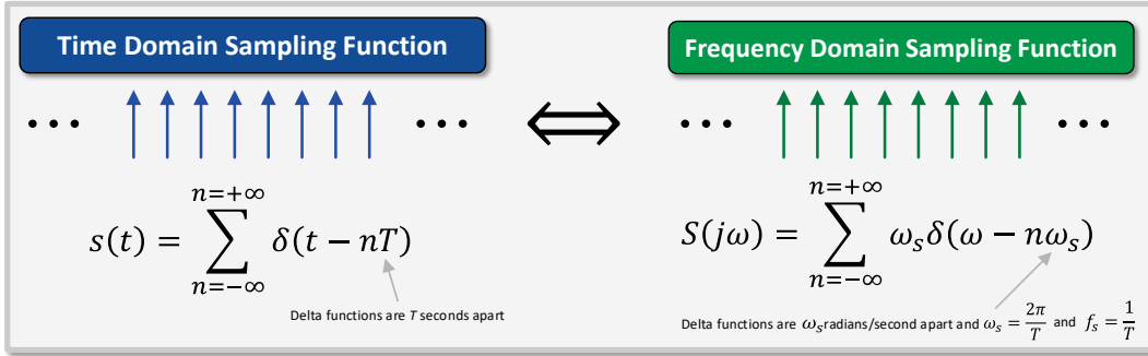
Fig. 9 Sampling function Fourier transform pair
