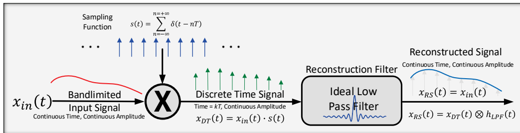
Fig. 8 Block diagram for Shannon’s sampling and reconstruction theorem
