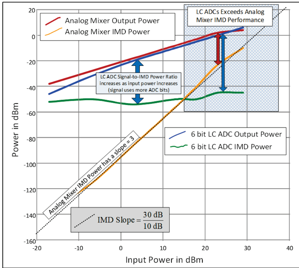
Fig. 40 Comparison of analog mixer (multiplier) to 64-level (6-bit), level-crossing ADC. Level-crossing ADC does not have a significant increase in intermodulation distortion power for high-signal-input powers.
