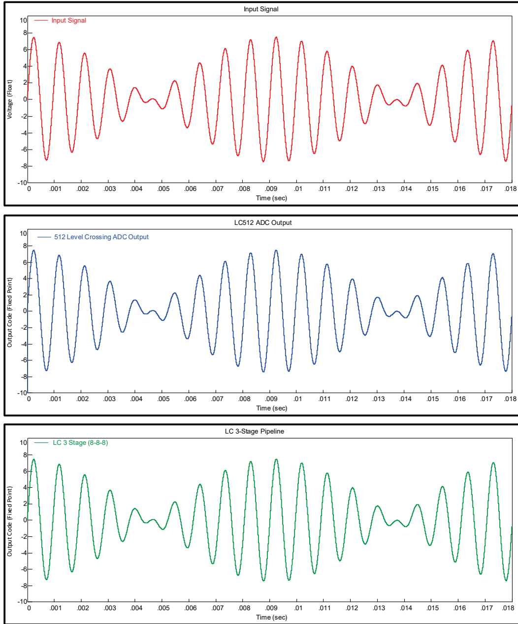
Fig. 33 Comparison of a simulated three-stage pipeline level-crossing ADC (requires 26 comparators and it is equivalent to a 512-level ADC) to a simulated 512-level, level-crossing ADC (requires 512 comparators). A two-tone input signal is used to compare the performance of the three-stage pipeline level-crossing ADC to a 512-level ADC.
