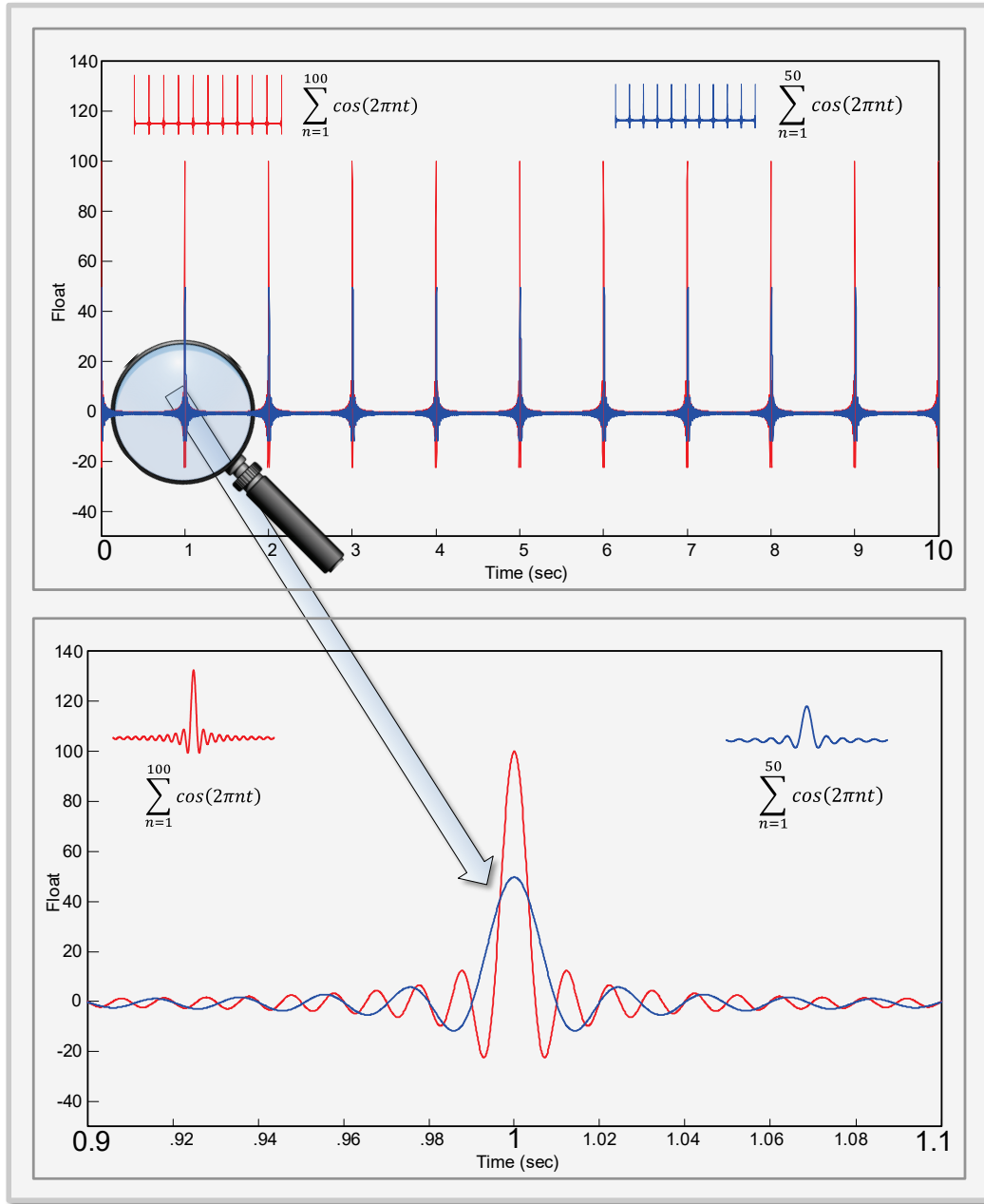
Fig. 14 Sampling function approximation. The sampling function has a slow convergence. For 50 terms, the peak amplitude is 50, and for 100 terms, it is 100. Each term adds 1 to the height. The sum converges very slowly. The slow convergence causes limitations for ADCs.
