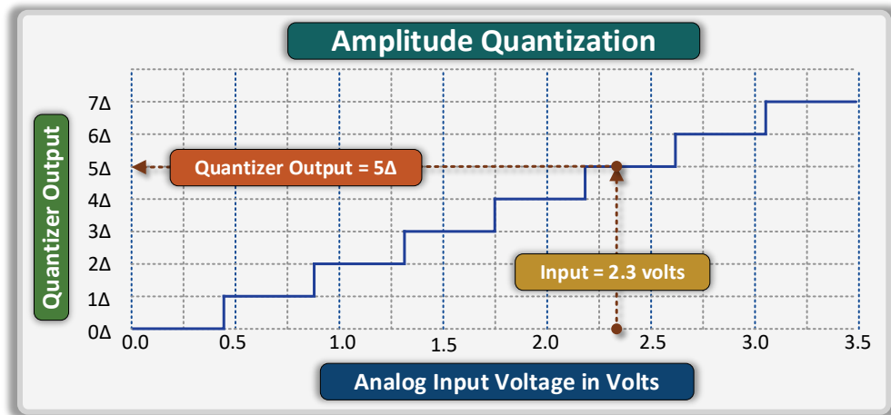
Fig. 16 Input voltage/output quantization transfer function
