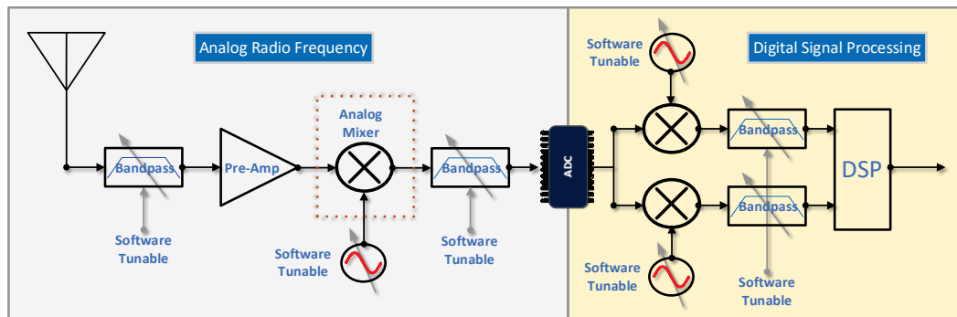
Fig. 41 A conventional software-reconfigurable radio. Analog mixer limits performance of a software-reconfigurable radio. Mixers are limited by dynamic range, intermodulation distortion, mixer conversion loss, and mixer noise.
