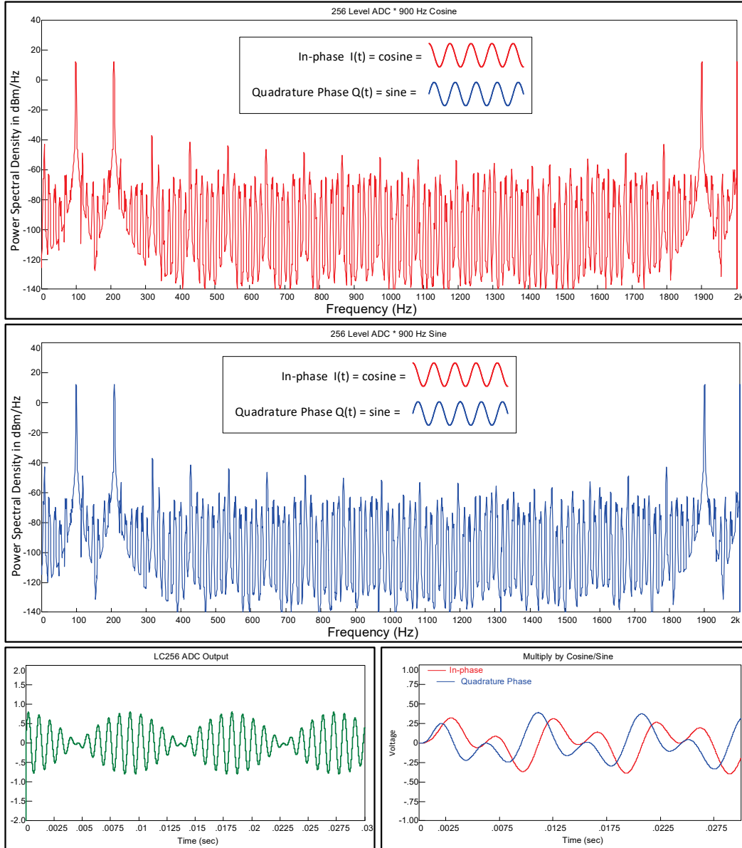
Fig. 44 Software-reconfigurable radio simulation using cosine/sine in-phase and quadrature-phase sine waves. A 256-level, level-crossing ADC was used for the simulations. Input signal is 1.0- and 1.11-kHz sine waves. I/Q modulator is 0.9-kHz complex sine wave. Frequency down-conversion for I/Q channels is shown. Tones at present at 100 and 211 Hz. Bottom graphs are level-crossing ADC time domain waveforms and I/Q channels.
