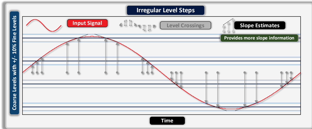
Fig. 25 Irregular level steps. By placing a fine level \pm 10\% above and below a coarse level, the level-crossing ADC can measure more details about the input signal's slope.
