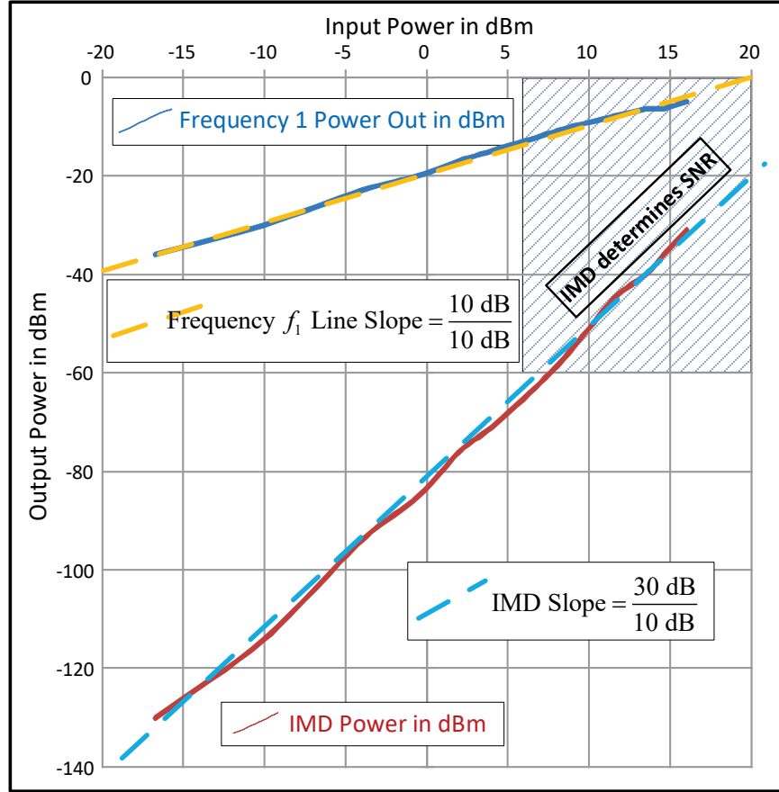
Fig. 39 Typical analog mixer third-order intermodulation distortion. The intermodulation distortion graph shows intermodulation distortion 57 for a typical analog mixer (multiplier). The analog mixer has an intermodulation distortion power with a slope of 30 dB/decade. The input signal power has a slope of 10 dB/decade. At high-input-signal powers, the intermodulation distortion power dominates and determines the SNR.
