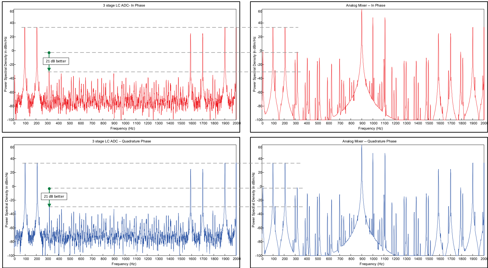
Fig. 47 Comparison of conventional simulated SRR with analog mixer front end and continuous-time SRR. This figure presents a simulation for the continuous-time software-reconfigurable radio using a continuous-time three-stage pipeline level-crossing ADC. Performance is compared to an “equivalent” conventional analog mixer front-end SRR. The graphs demonstrate a significant performance improvement for intermodulation distortion for the continuous-time SRR and continuous-time pipeline level-crossing ADC.
