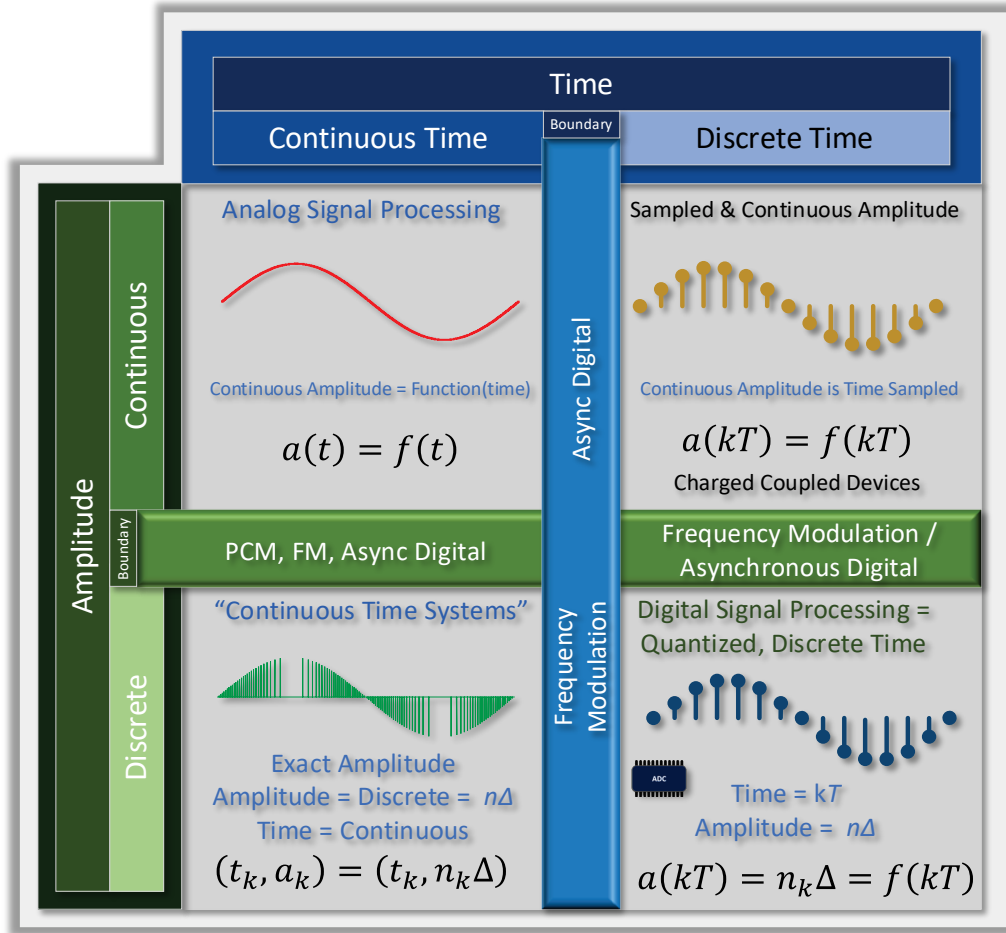
Fig. 1 Signal processing architectures. There are four signal processing domains. 14 Continuous and discrete for both time and amplitude. The boundary regions offer unique signal processing properties. 15 Discrete time is characterized by sample times = kT . Digital is quantized amplitude (amplitude = n\Delta ) and sample times = kT . For continuous-time signals, time is continuous (not quantized). Discrete-amplitude continuous time, often shortened to continuous time, is characterized by equivalence times, the times, t_k , when the input signal equals a discrete value. At the equivalence times, the input signal exactly equals a discrete amplitude; there is no quantization error compared to digital signal processing. Continual signal processing is defined as exact "discrete" amplitude (no amplitude quantization error) and continuous time (time is not quantized).
