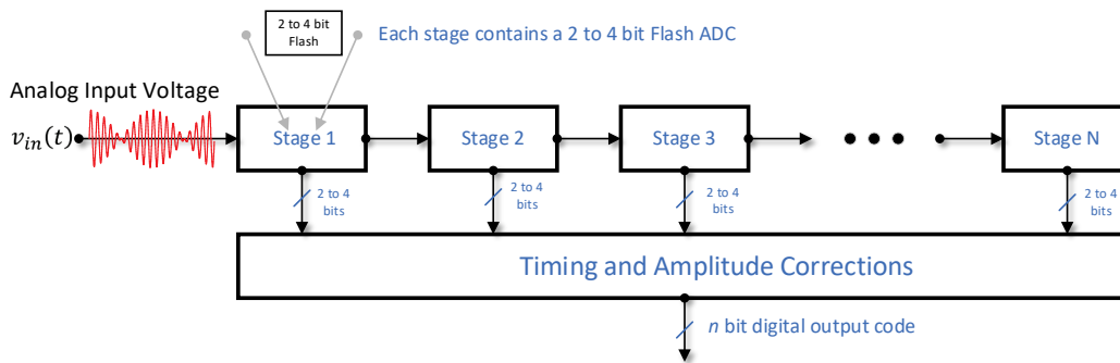
Fig. 29 Prior art conventional pipeline flash ADC. A pipeline flash ADC consists of n -stages, where the error voltage (stage input – digital output) is fed into the next stage and repeated.
