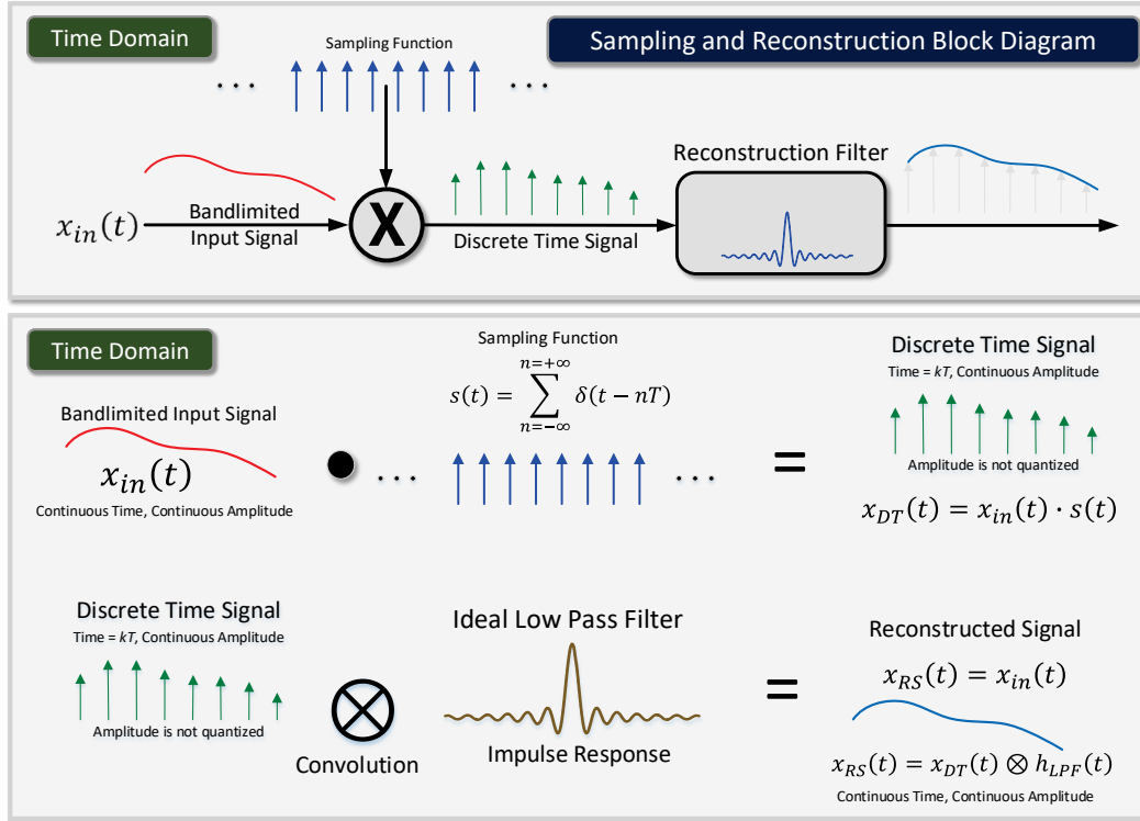
Fig. 11 Shannon sampling algorithm in the time domain. The input signal is sampled using an array of delta functions. The input signal is exactly recovered using an ideal low-pass filter with a \text{sinc}(at) impulse response.
