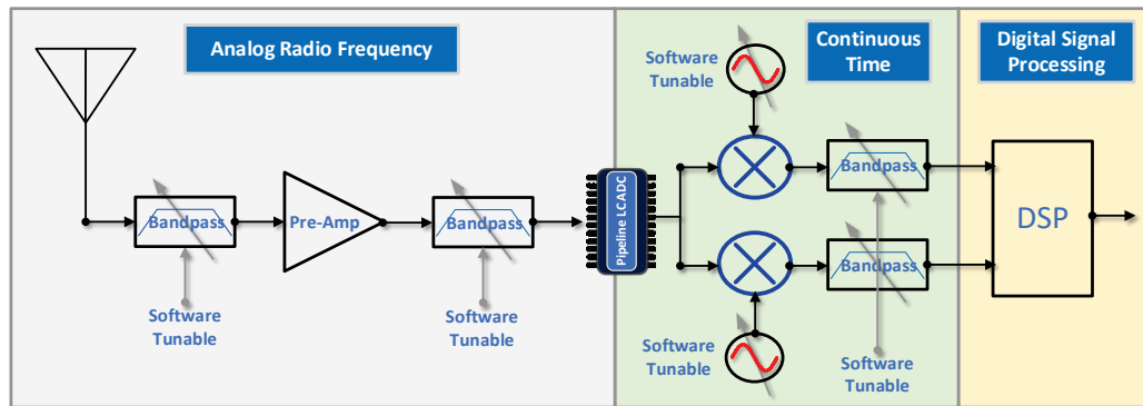
Fig. 42 Software-reconfigurable radio with pipeline level-crossing ADC. Continuous-time multipliers are asynchronous digital multipliers, not analog, and not clocked digital. Asynchronous digital multipliers do not have the intermodulation distortion limitations present in conventional analog mixers (multipliers). All signal processing can be done in continuous time; however, conventional digital signal processors and FPGAs are clocked. By using a clocked latch, continuous time can be simply converted to digital for conventional DSP processing.
