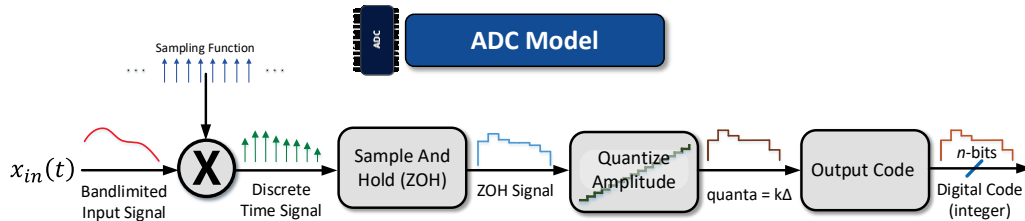
Fig. 17 Conventional ADC model. Shannon's sampling theorem requires the input signal to be bandlimited and the sampling frequency to be f_s > 2f_{bw} . A zero-order hold provides a constant value for 1 time step. The quantizer converts the ZOH signal to a quantized value. The coder stage assigns a digital code to the quantized value.
