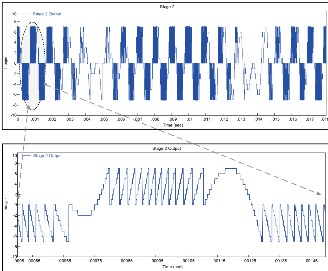
Fig. 35 Simulated pipeline stage 2 output for a three-stage pipeline level-crossing ADC
