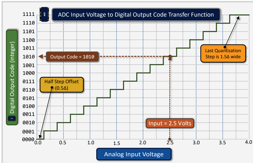
Fig. 18 Half-step offset quantization. For round-down quantization, the quantization error is bounded by 0 \leq \text{quantization error} \leq \Delta . For half-step offset quantization, the quantization error is bounded by -\frac{1}{2}\Delta \leq \text{quantization error} \leq \frac{1}{2}\Delta . Half-step offset quantization has half the maximum quantization error.
