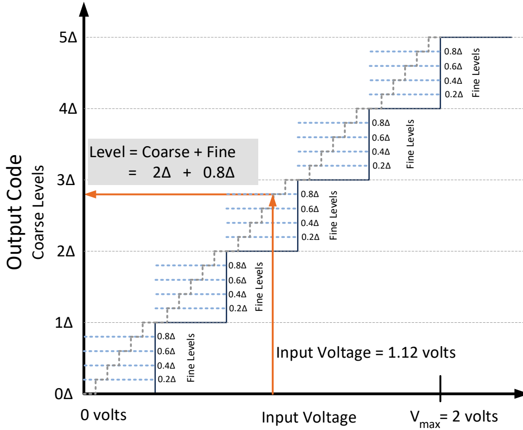
Fig. 31 An input voltage to output-level (digital code) transfer function. Coarse levels are located at 0\Delta, 1\Delta, 2\Delta, 3\Delta, 4\Delta , and 5\Delta . The error voltage between the input signal and coarse level value is fed into the fine level-crossing stage. The fine level-crossing voltage levels are 0.2\Delta, 0.4\Delta, 0.6\Delta , and 0.8\Delta . The fine voltage levels of 0.0\Delta and 1.0\Delta are not used. The fine voltage levels of 0.0\Delta and 1.0\Delta would overlap with the coarse voltage levels of 0\Delta, 1\Delta, 2\Delta, 3\Delta, 4\Delta , and 5\Delta . The pipeline design guarantees that only one level in any pipeline stage may be crossed at a time. An example input voltage of 1.12 V is mapped to coarse level = 2\Delta and fine level = 0.8\Delta for an output value = 2.8\Delta .
