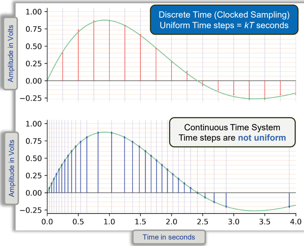
Fig. 2 Comparison of discrete time (uniform time steps) to continuous time (nonuniform time steps). For discrete time, each sample is a fixed time step apart (sample times = kT ). For a continuous-time signal, the “sampling frequency” is proportional to the input signal’s slope. The distance between samples is not constant (nonuniform time steps). The sampling frequency self-adapts to the input signal, and it is more energy efficient than DSP.
