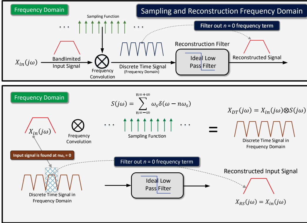
Fig. 12 Shannon sampling in the frequency domain. The input signal's frequency spectrum is sampled by convolving it with an array of delta functions. The discrete-time signal's frequency spectrum is the input signal's spectrum replicated across each delta function. By applying an ideal low-pass filter, the frequency spectrum of the input signal is exactly recovered.
