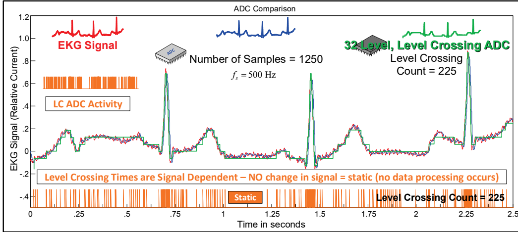
Fig. 4 Comparison of conventional DSP to CT for ECG signals. The 32-level, level-crossing ADC requires significantly fewer sample points compared to conventional Shannon sampling. This illustrates the low-power potential for nonuniform time step, level-crossing sampling.
