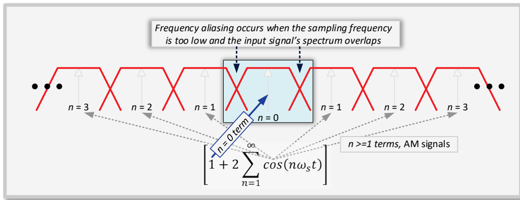
Fig. 13 Frequency aliasing occurs when the sampling frequency is too low and the input signals' spectrums overlap. Frequency aliasing cannot be removed. If the input signal is a cosine, the product of \cos(2\pi f_1 t) \cdot \cos(2\pi f_2 t) results in \cos[2\pi(f_1 \pm f_2)t] . The sum and difference frequencies, f_1 \pm f_2 , cause frequency aliasing.
