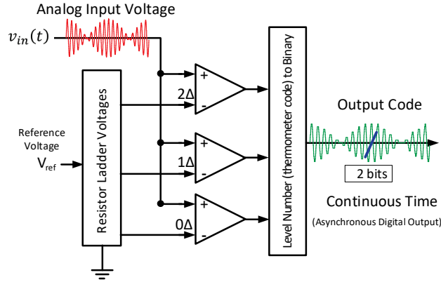
Fig. 28 Prior art 2-bit* continuous-time level-crossing ADC. A level-crossing ADC is similar to a conventional flash ADC without the clocked latch. An n -bit flash ADC requires 2^n - 1 comparators and has exponential complexity. Each bit of resolution doubles the number of comparators. (*Costs more than 25 cents.)
