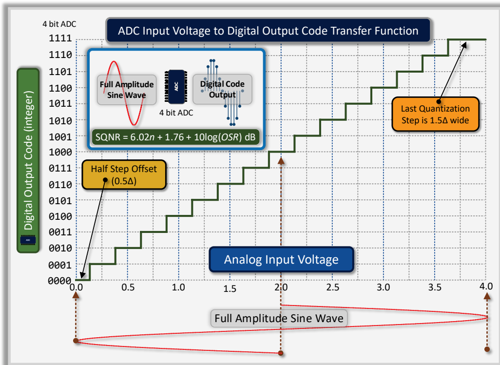
Fig. 19 Full-amplitude input sine wave. A sine wave that completely covers the input voltage range is used to calculate the signal-to-quantization noise ratio for an ADC.
