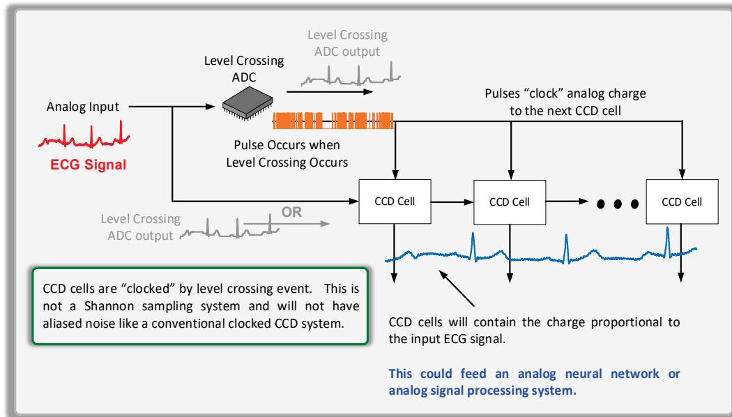
Fig. 27 Continuous-time analog CCD system. With a level-crossing ADC, an array of CCD cells can be clocked with the level-crossing times to create an analog CCD continuous-time system. The CCD cells' outputs can then be used in a fully analog signal-processing system.
