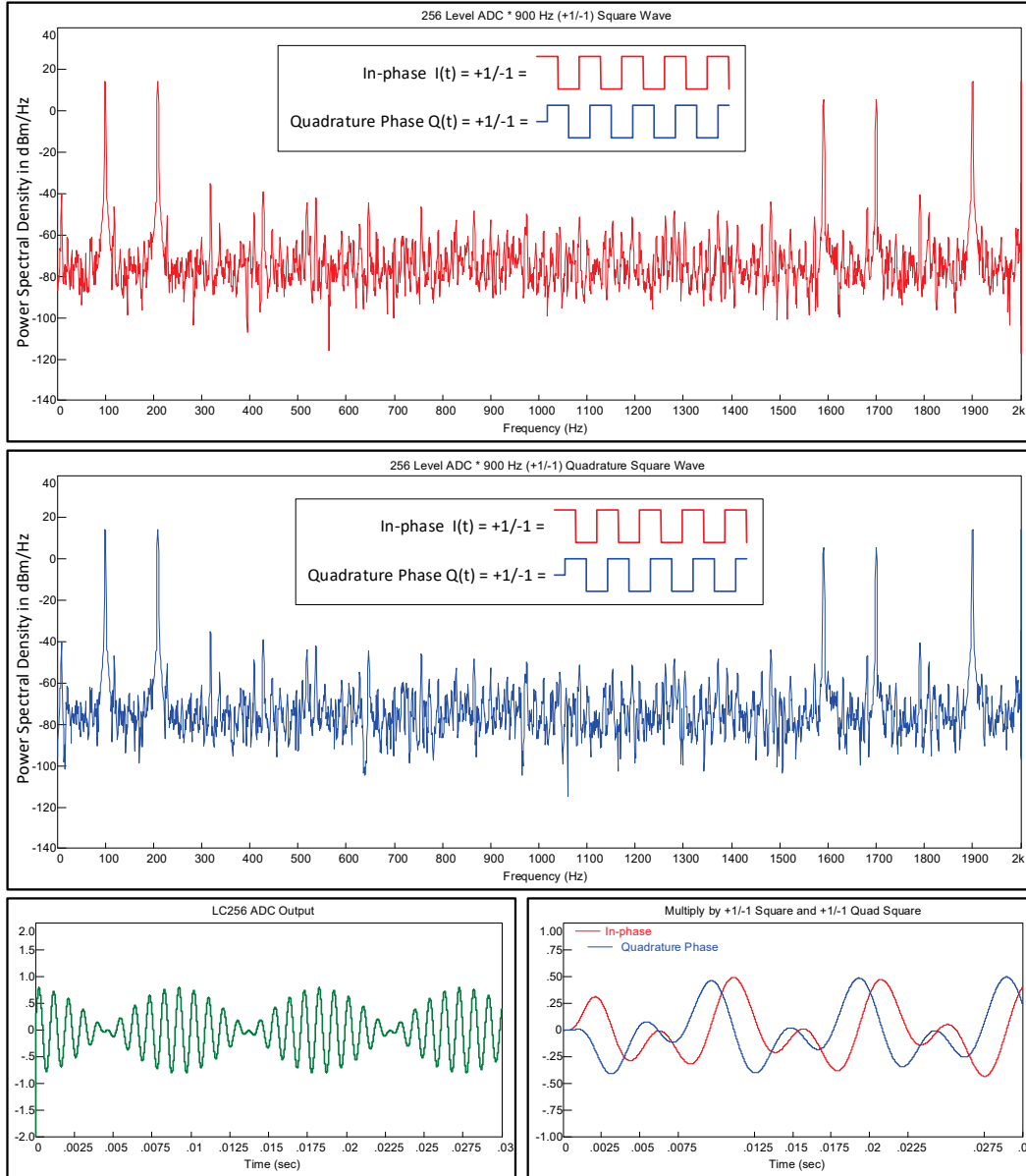
Fig. 45 Software-reconfigurable radio simulation using +1/-1 in-phase and quadrature-phase square waves. A 256-level, level-crossing ADC was used for the simulations. Input signal is 1.0- and 1.11-kHz sine waves. I/Q modulator is 0.9-kHz complex square wave with +1/-1 amplitude. Frequency down-conversion for I/Q channels is shown. Tones are present at 100 and 211 Hz. Image frequencies occur at 1.6 and 1.7 kHz. Bottom graphs are level-crossing ADC time domain waveforms and I/Q channels.
