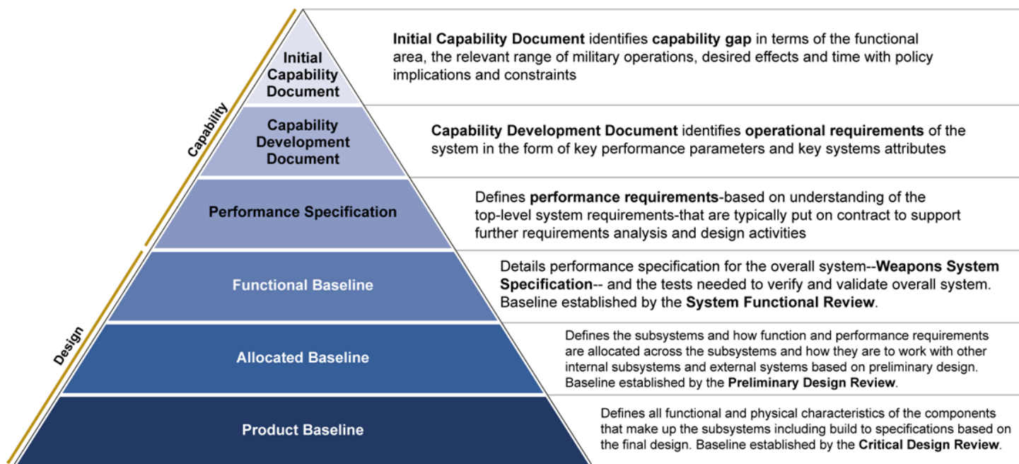
Figure 1: Requirements Decomposition
