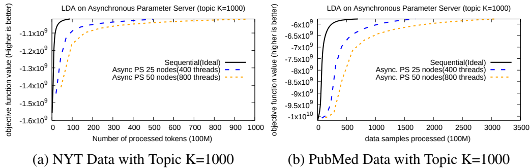
Figure 3.7: LDA topic modeling on asynchronous parameter server: reports convergence per processed data (= progress per update). Note that larger degree of parallelism leads to less progress per update due to model dependency.
