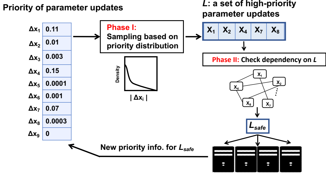
Figure 5.1: Workflow of Two-Phase Scheduling in Dynamic-SchMP: Dynamic scheduler keeps track of priority information of individual model parameter updates. Priority of a model parameter update represent convergence distance of parameter values assoricated with the parameter update, and we approximate convergence distance by sum of delta of parameter values. Phase-I selects a set of model parameter update L based on the priority distribution. Phase-II builds model dependency graph for model parameters in L and checks on dependency structure. If a pair of parameters are found to have too strong dependency (larger than a threshold), one of them are set aside for next round. After dependency check, L is reduced to L_{safe} that degree of dependency on all possible pairs is less than a threshold.
