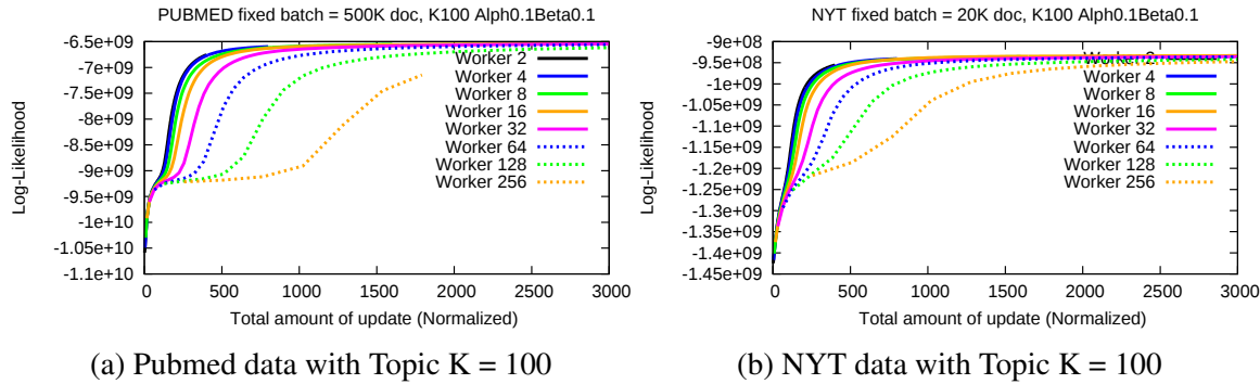
Figure 3.6: LDA topic modeling on BSP simulation: reports convergence per update. Note that larger degree of parallelism leads to less progress per update due to model dependency.
