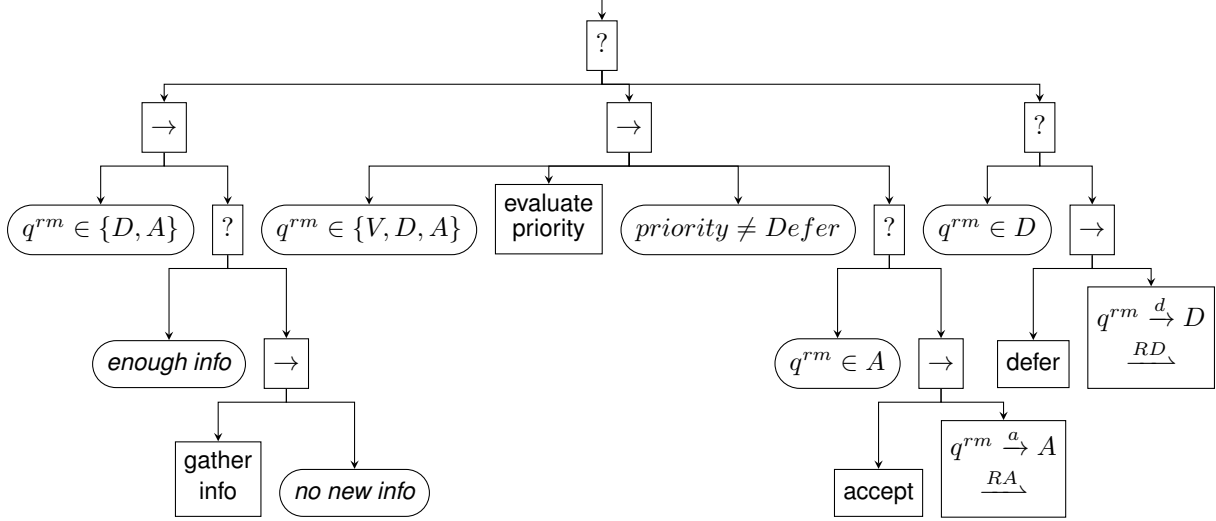
Figure 7.6: Prioritize Report Behavior Tree
