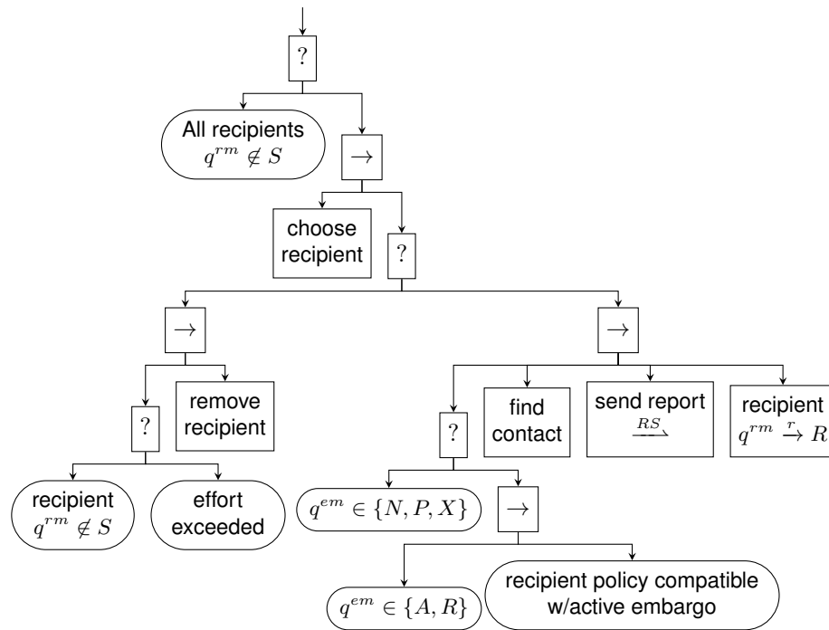
Figure 7.16: Notify Others Behavior Tree
