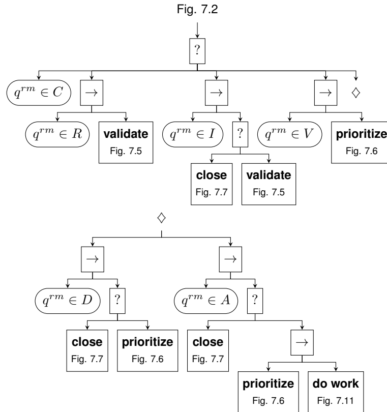
Figure 7.4: Report Management Behavior Tree
