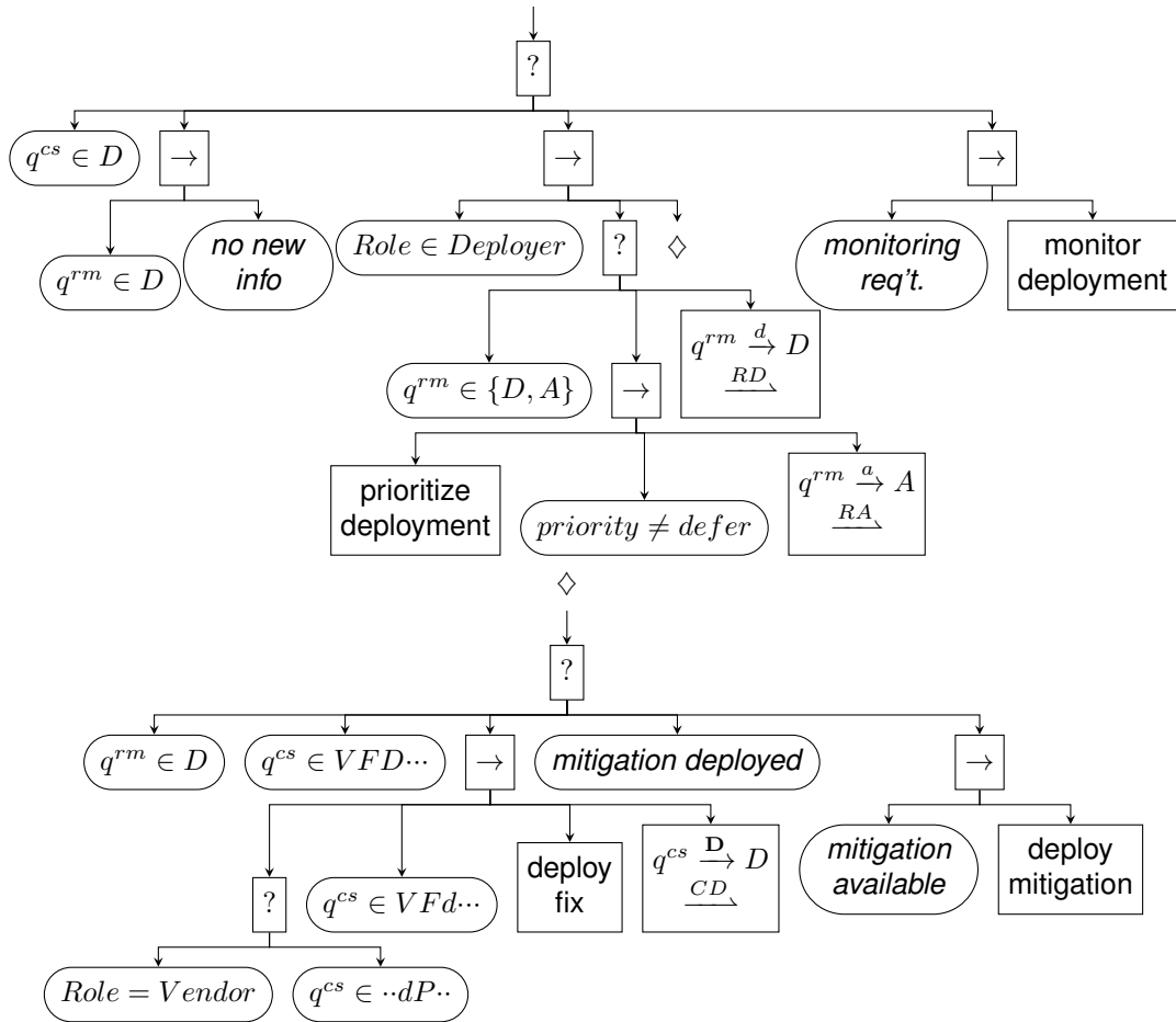
Figure 7.12: Deployment Behavior Tree
