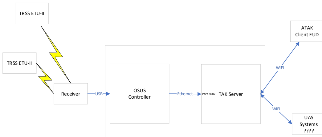
Fig. 1 System architecture
