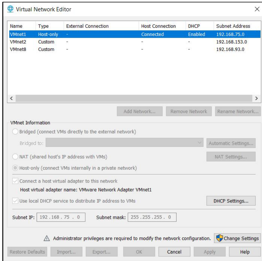
Fig. 2 Virtual network editor
