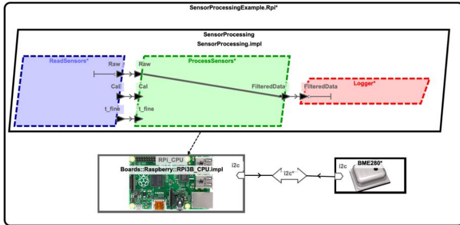
Figure 14: SensorProcessing/AADL Model
