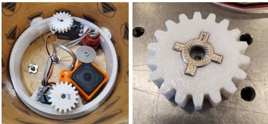
Figure 94. Sled Coupling Base (Left) and Gear Titanium Insert (Right).
