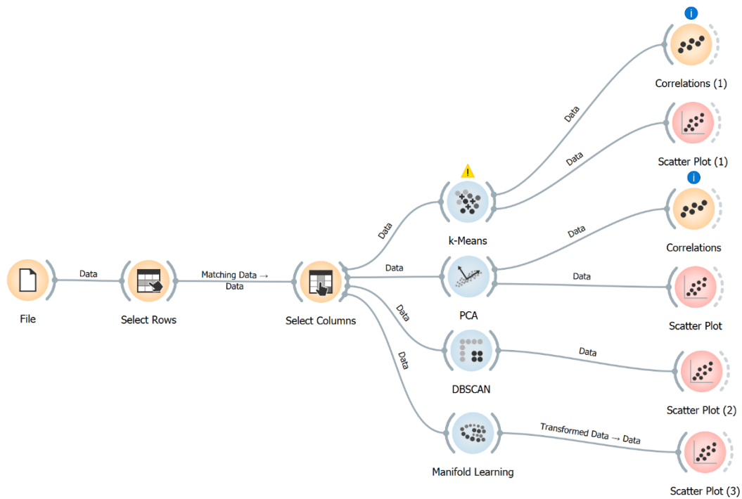
Figure 31. Orange Workflow
