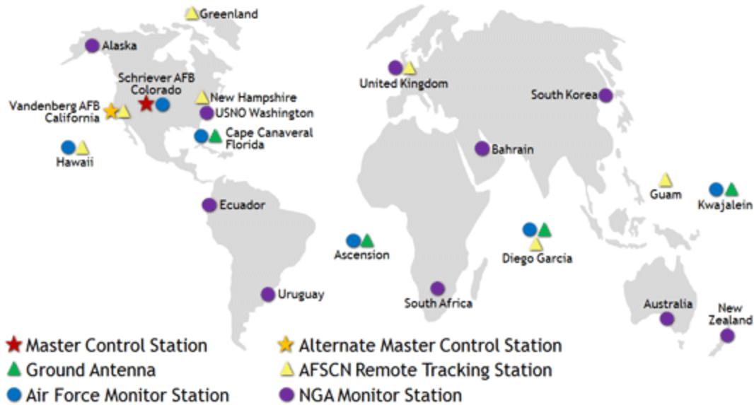
Figure 5. Control Segment. Source: GPS.gov (2018).
