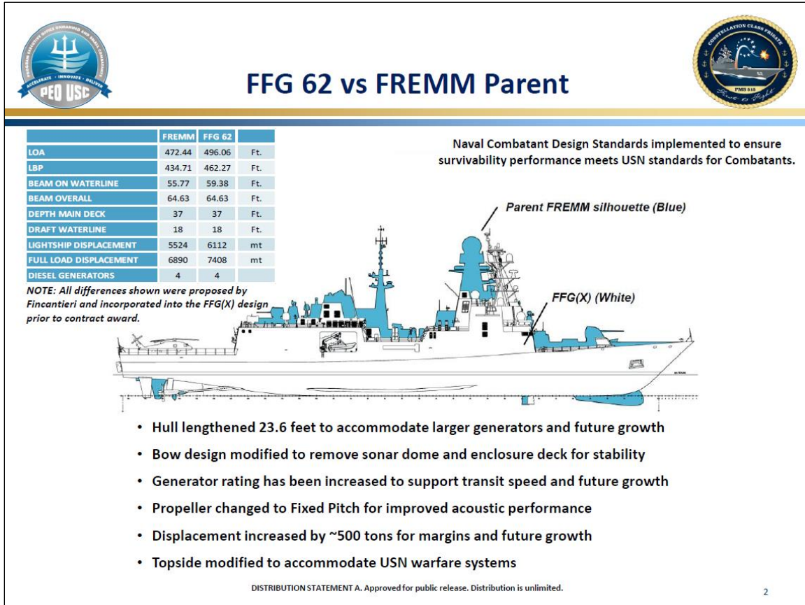
Figure 4. Navy Briefing Slide Comparing FFG-62 Design to FREMM Design
