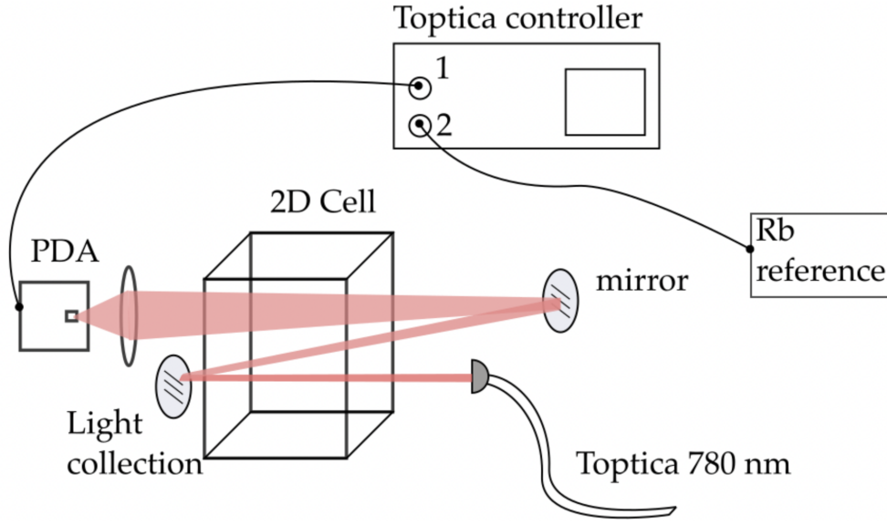
Fig. 2—Schematic of the saturation spectroscopy setup. 10\ \mu\text{W} of the trap laser is coupled to the 2D vapor cell. The beam slowly diverges as it passes through the vapor cell multiple times. The trap laser (“Toptica”) controller continuously scans while recording the absorption signal of both the 2D cell and Doppler-free Rb reference.
