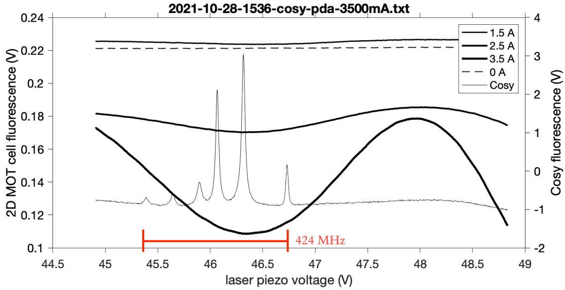
Fig. 3—Absorption profile of the ^{87}\text{Rb } 2S_{1/2} (F=2) \rightarrow 2P_{3/2} transition. Left axis: several Doppler-limited saturation spectroscopy measurements at different oven currents. Right axis: Doppler-free reference spectrum (Cosy), which reveals the hyperfine splittings.
