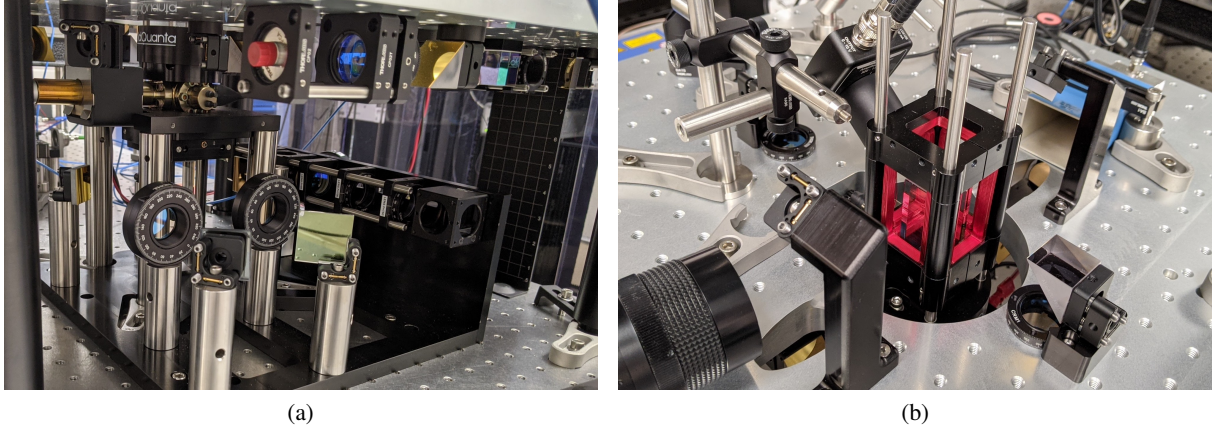
Fig. 1—Left: the lower 2D MOT loading chamber. Right: the upper 3D MOT trapping chamber. The chambers are connected by a 0.75 mm diameter pinhole.
