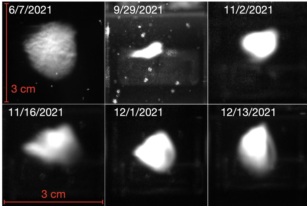
Fig. 7—Snapshots of the rubidium cloud confined in a 3D MOT as the lasers and optics are refined over a six-month period.
