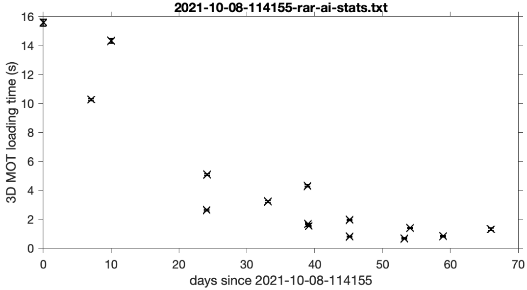
Fig. 6—The rubidium MOT load time as improvements to the apparatus are made over the course of several months. The trapping laser powers and repump laser power are tuned each week. Other small optimizations of the apparatus are made throughout this time. Notable changes are listed in what follows. Day 24: refined 2D MOT beam alignment, refined 2D stage positioning. Day 33: refined 3D MOT beam alignment, refined magnetic field supply current, refined pump laser frequency. Day 45: implement 2D MOT push beam.
