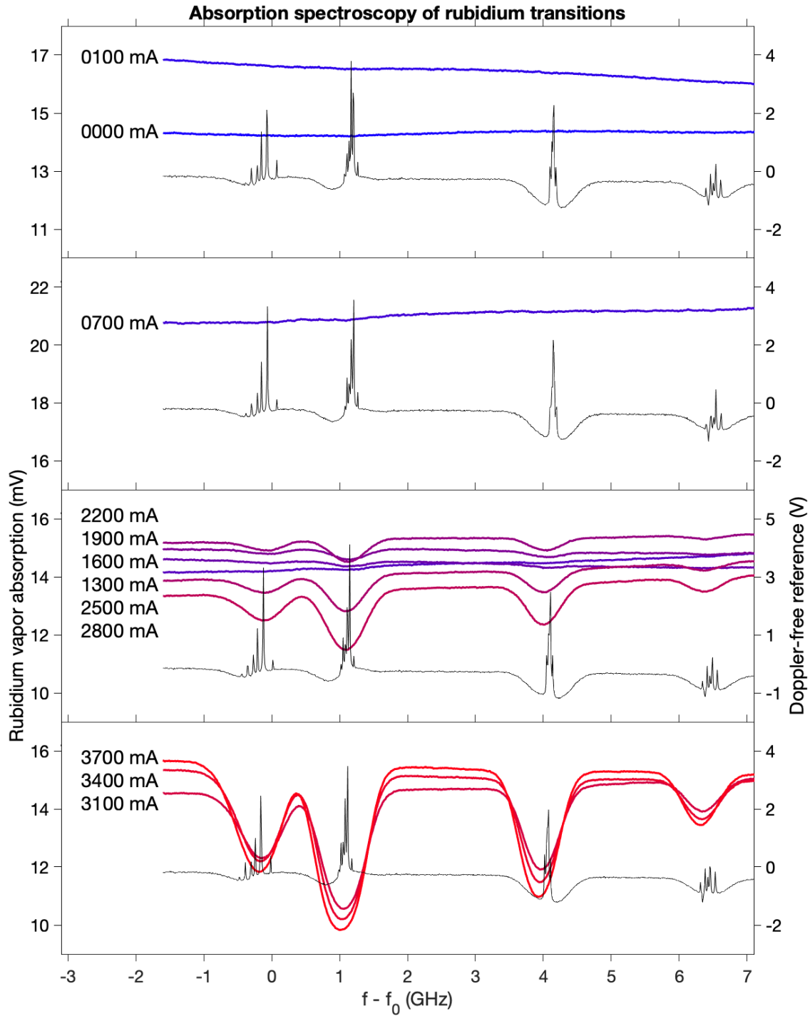
Fig. 4—Wide scan of the rubidium absorption profile for a range of rubidium cell currents, up to the manufacturer-specified limit of 3.7 A. The horizontal scale is the fitted laser frequency relative to the clock transition ^{87}\text{Rb } 2S_{1/2} (F = 2) \rightarrow 2P_{3/2} (F' = 3) . From left to right, the Doppler-limited transitions are: ^{87}\text{Rb } 2S_{1/2} (F = 2) \rightarrow 2P_{3/2} , ^{85}\text{Rb } 2S_{1/2} (F = 3) \rightarrow 2P_{3/2} , ^{85}\text{Rb } 2S_{1/2} (F = 2) \rightarrow 2P_{3/2} , ^{87}\text{Rb } 2S_{1/2} (F = 1) \rightarrow 2P_{3/2} .
