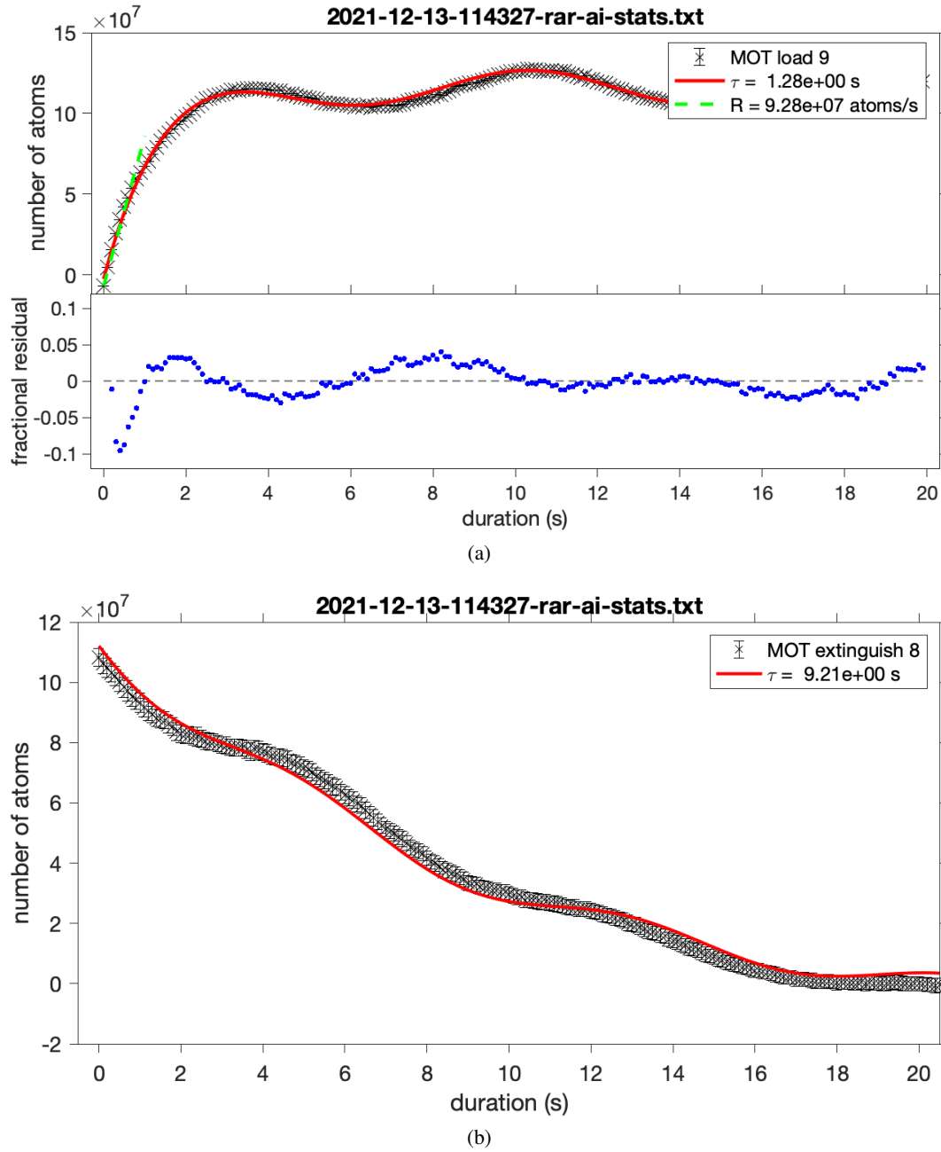
Fig. 5—(a) A fit to a selected 3D MOT loading sequence. The bottom half of the plot is the relative deviation of the fit from the data. (b) A fit to a selected 3D MOT lifetime sequence.
