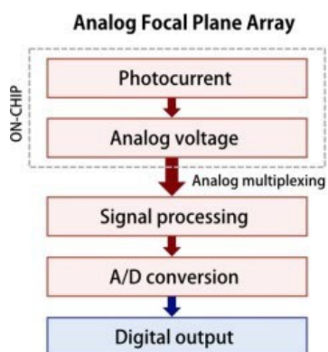
Figure 9. Typical building blocks in an analog FPA and ROIC design
