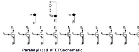
Parallel-placed nFETs schematic
