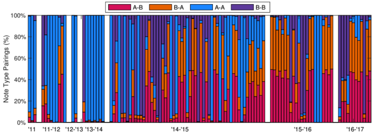
Figure 12. Percentage of different note pairings for each of the 115 fin whale tracks, spanning 2011–2017.
