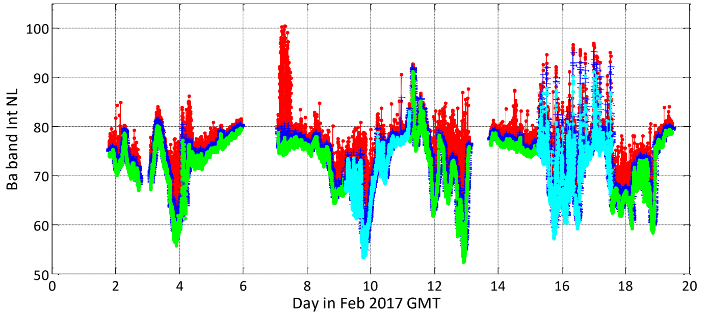
Integrated Levels in Ba detection band for Feb 2017 hydrophone K-5
