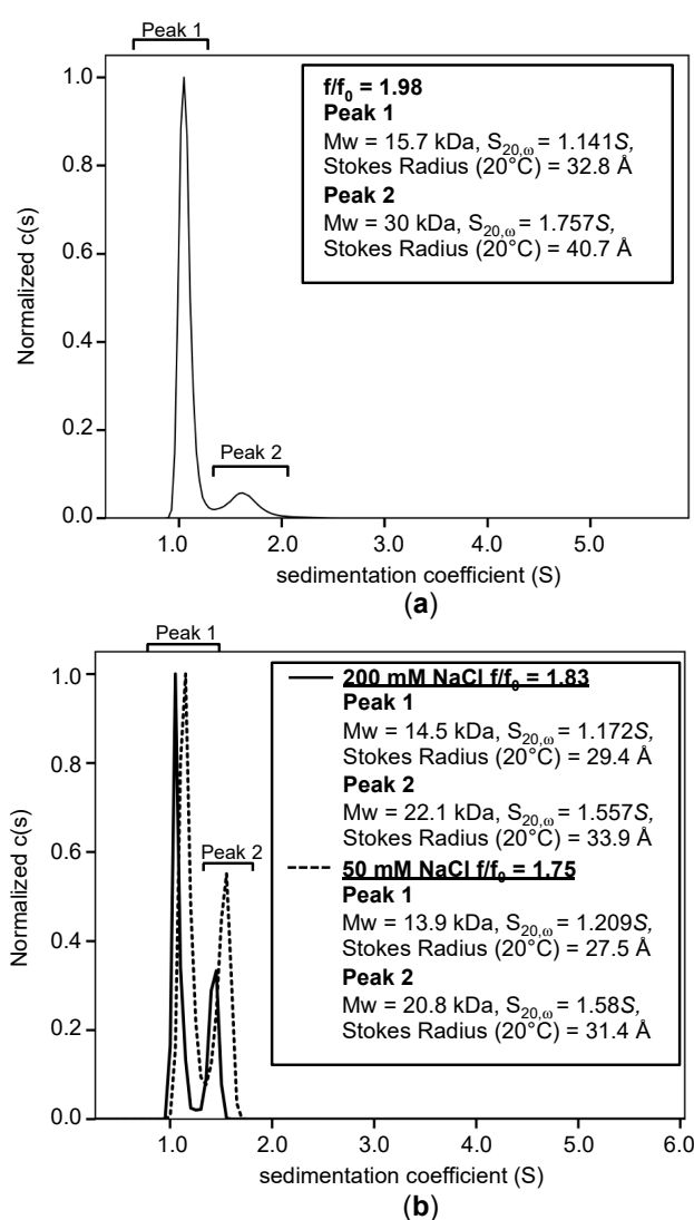
Figure 8. Sedimentation velocity of TNIP1 417-509 reveals oligomerization potential. Analytical ultracentrifugation sedimentation velocity of purified TNIP1 417-509 at 20 mM was performed in (a) 20 mM sodium phosphate buffer (pH 8.0) and 200 mM NaCl or (b) 20 mM sodium phosphate buffer (pH 5.8) and either 50 mM (dotted line) or 200 mM (solid line) NaCl with protein at 20 \mu M. Experimental runs were performed at 20 °C with scans at 6-min intervals at 230 nm for a total of 20 h. (a, b insets) Data analysis performed using SedFit.
