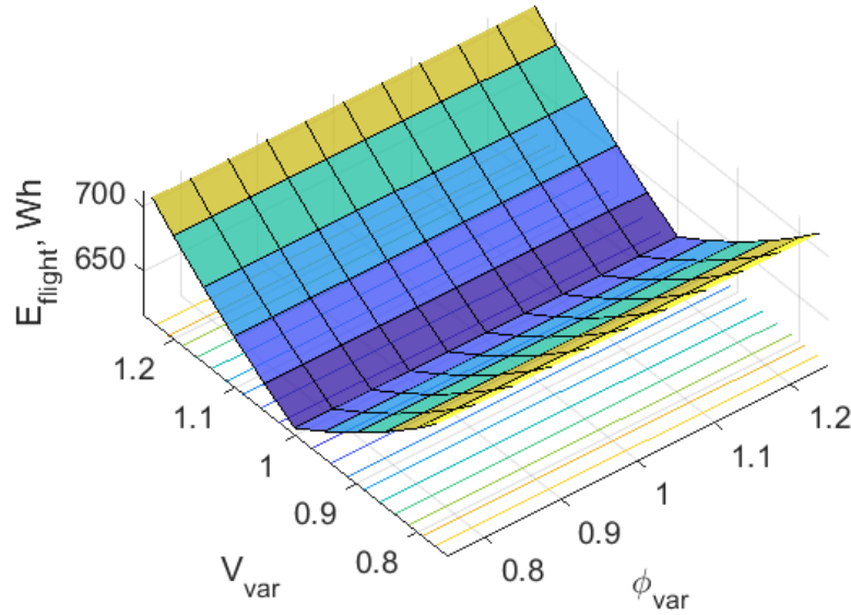
Figure 4.12. Variance of Optimal Energy Consumption from BVP Solver.
