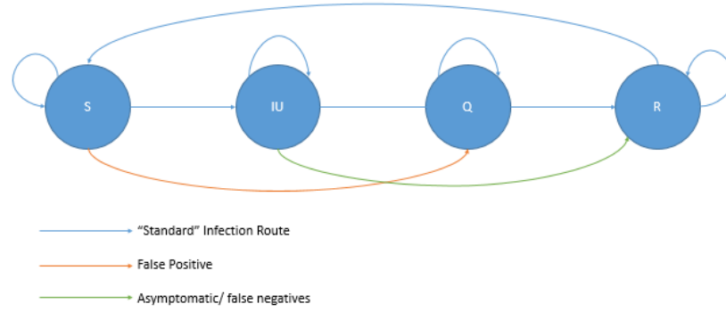
Figure 1. 4-Stage Markov Model
