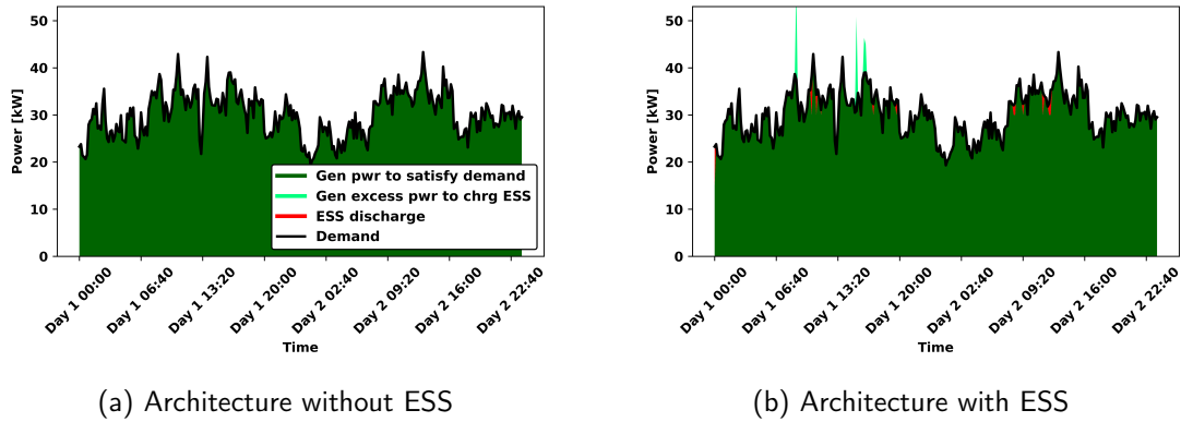
Figure 4.10. Power output plot for summer demand without ESS (left) and with ESS (right).
