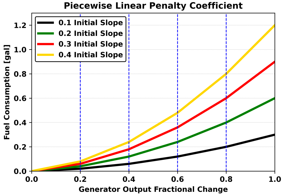
Figure 3.5. Fuel consumption plots for piecewise linear penalty profiles with varying initial slopes.
