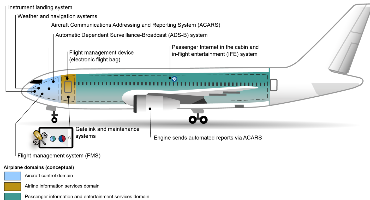
Figure 1: Key Systems Connections to Commercial Airplanes
