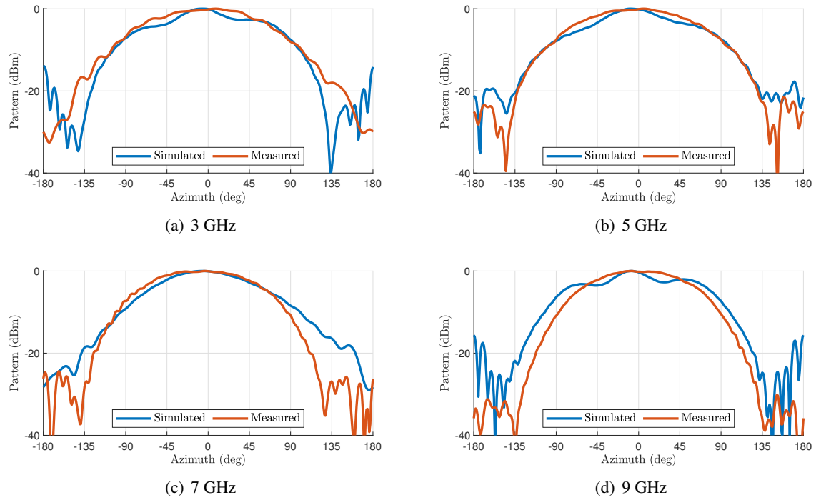
Fig. 10 — Comparison between simulated and measured column patterns for select frequencies.
