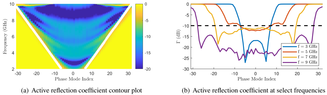
Fig. 4 — Active reflection coefficient, \Gamma .
