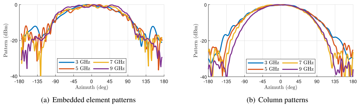
Fig. 8 — Measured patterns for select frequencies across the bandwidth. (a) Embedded element patterns for a center element in a column. (b) Column pattern.
