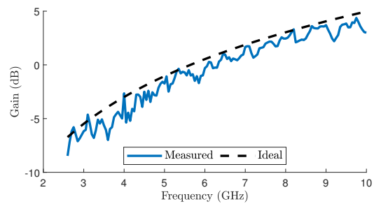
Fig. 11 — Gain of element with respect to the ideal gain.
