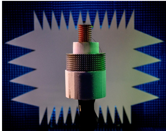
(b) Array fabricated
