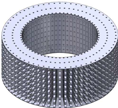
(a) Array design
