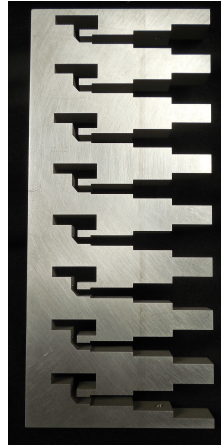
Fig. 6 — Fabricated column element using EDM
