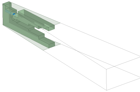
Fig. 2 — HFSS unit cell simulation setup
