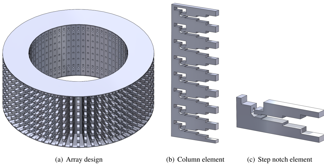
Fig. 1 — Cylindrical array design.
