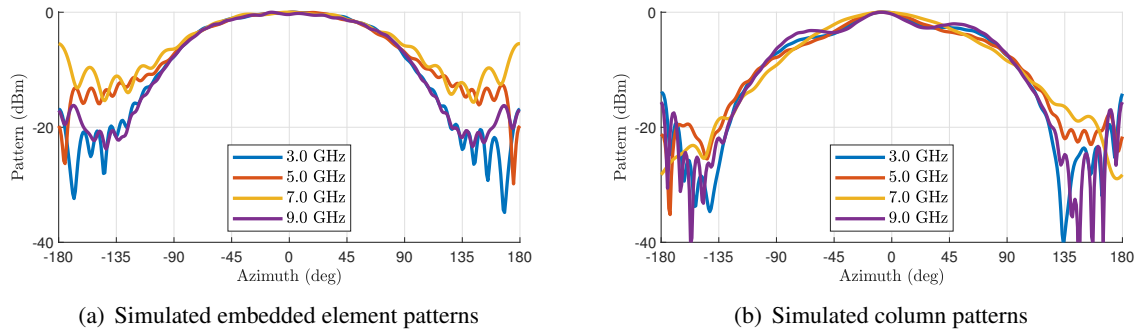
Fig. 5 — Simulated patterns at select frequencies.
