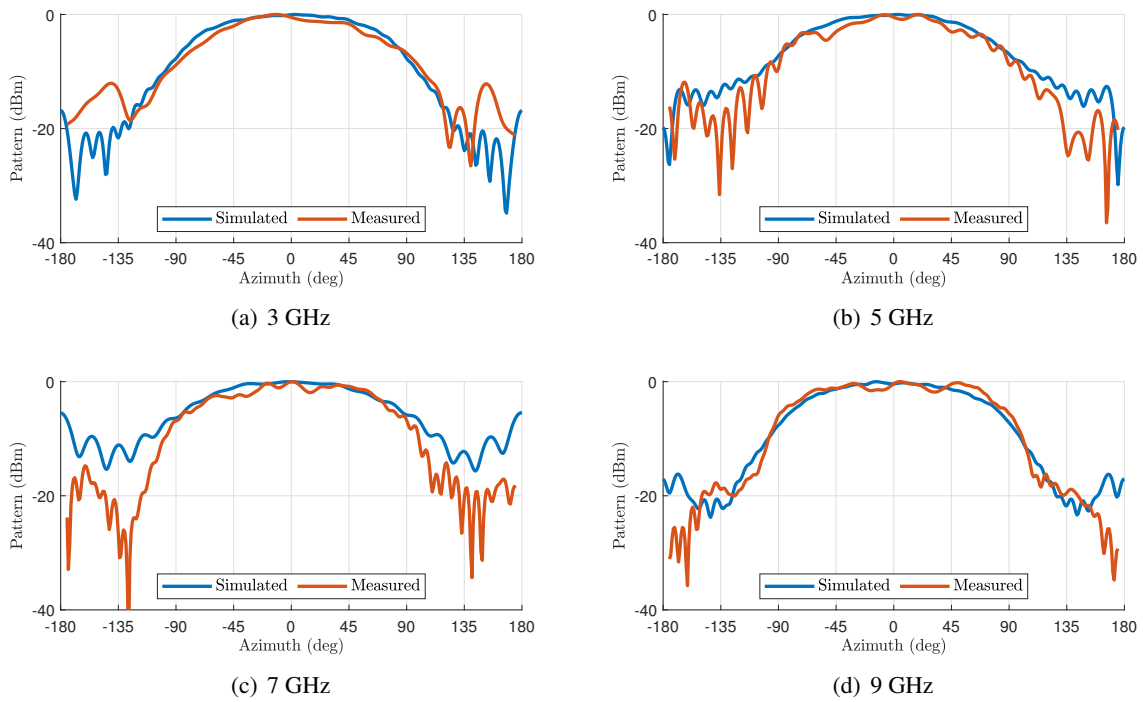
Fig. 9 — Comparison between simulated and measured embedded element patterns for select frequencies.
