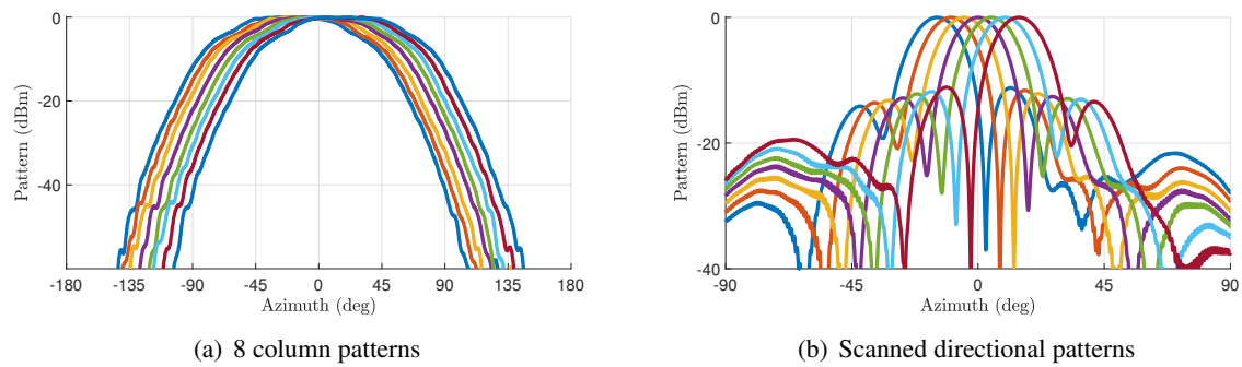
Fig. 12 — (a) Measured column patterns for the 8 column elements to be used in the demo. The shift in pointing direction between the patterns correlates to the angular distance between each element. (b) Scanned directional patterns over the \pm 15 deg scan area desired.
