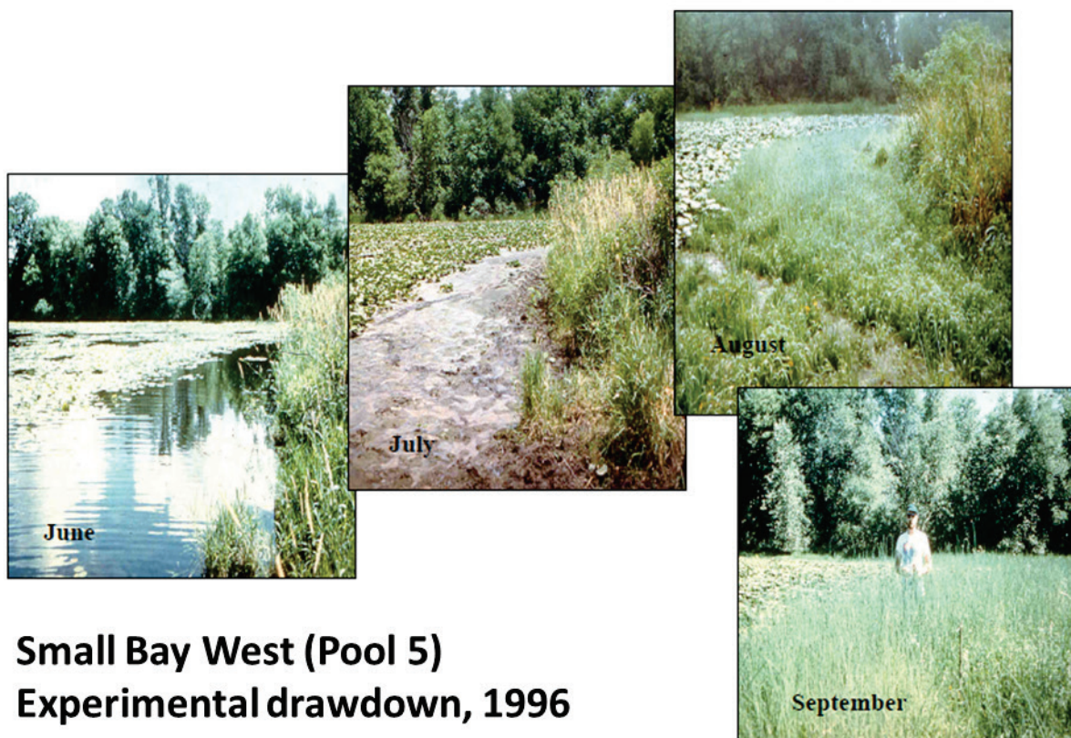
Figure 5. Pool 5 experimental backwater drawdowns in 1996. The sequence of photographs (left to right) through time from June to September 1996 shows the positive plant response to the planned drawdown (USACE 2007, 2).
