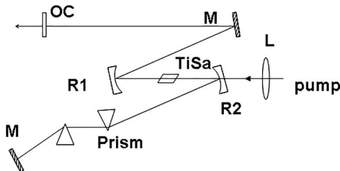
FIGURE 6.4 Typical cavity layout for a Ti:sapphire laser using prisms for dispersion compensation.
