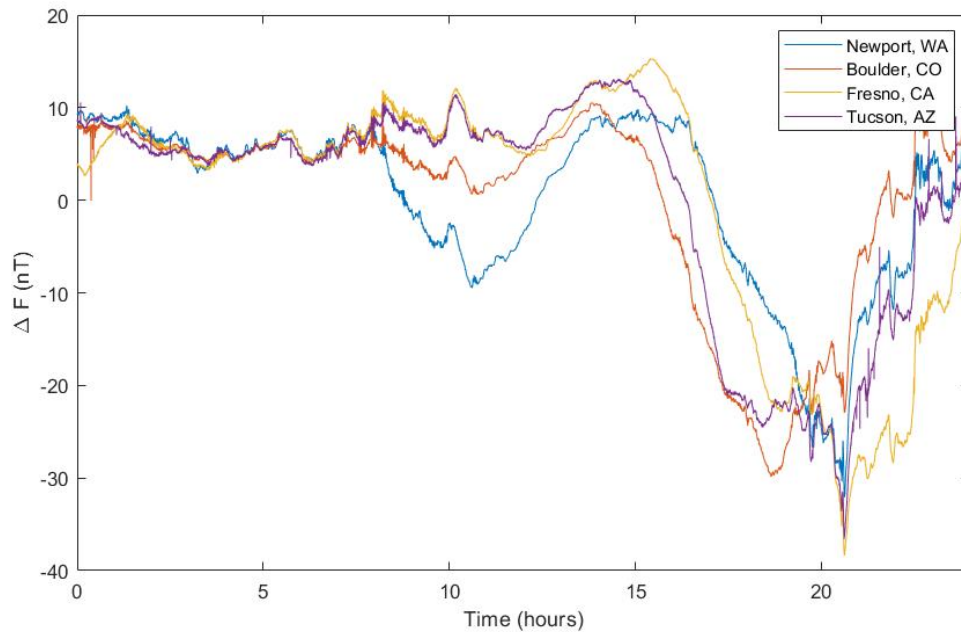
Figure 4: Temporal Variations with mean removed over a 24 hour period at different base stations in the Western United States. Figure generated from data provided by [15]
