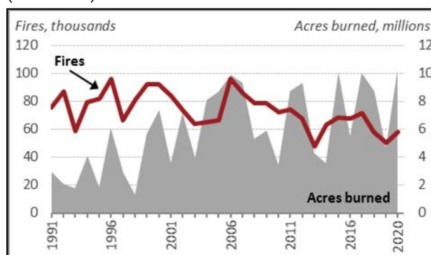
Figure 1. Annual Wildfires and Acres Burned (1991-2020)
