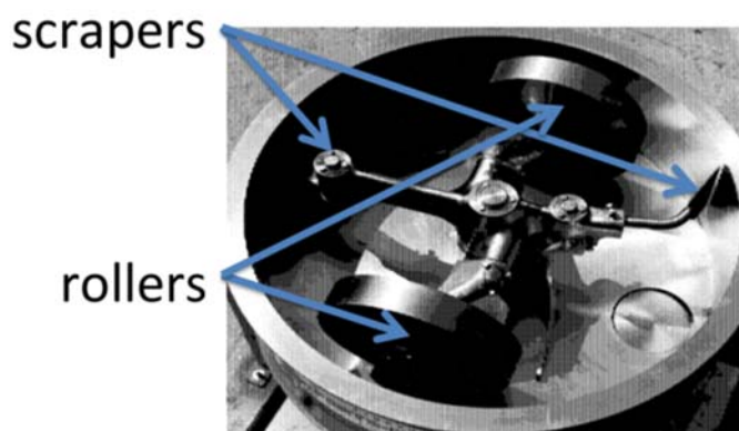
Figure 2. Example of a mix-muller mixer.
