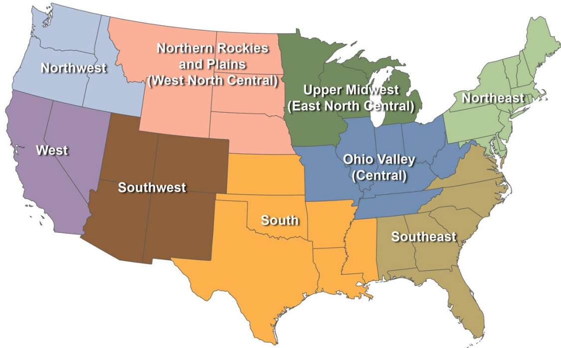
Figure 2. The National Centers for Environmental Information (NCEI) climate regions used in this study. Abbreviations for the regional titles are: Northwest — NW; West North Central — WNC; East North Central — ENC; Northeast — NE; West — W; Southwest — SW; South — S; Central — C; Southeast — SE.
