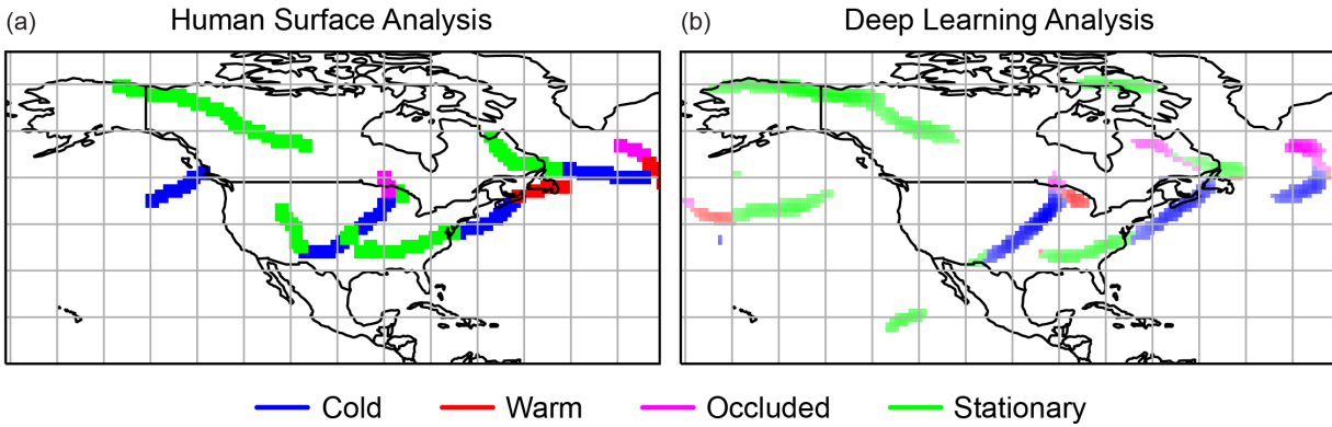
Figure 6. Side-by-side comparison of CSB (a) and DL-FRONT (b) front boundaries for 2009-08-01 12:00:00. The CSB fronts were drawn three grid cells wide. The intensities of the colors for the different front types in the DL-FRONT image represent the likelihood value (from 0.0 to 1.0) associated with each grid cell.
