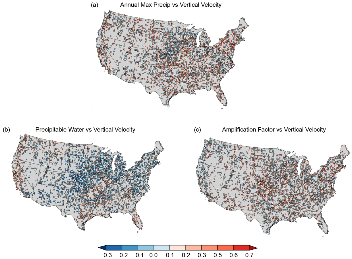
Figure 22. Correlation coefficients for the annual maximum series of (a) EP event magnitude with -\omega , (b) PW with -\omega , and (c) A with -\omega . PW and -\omega are the simultaneous day's 3-hr maximum precipitable water and 3-hr maximum vertical velocity, respectively. Triangles indicate statistically significant (0.05 level) correlations.
