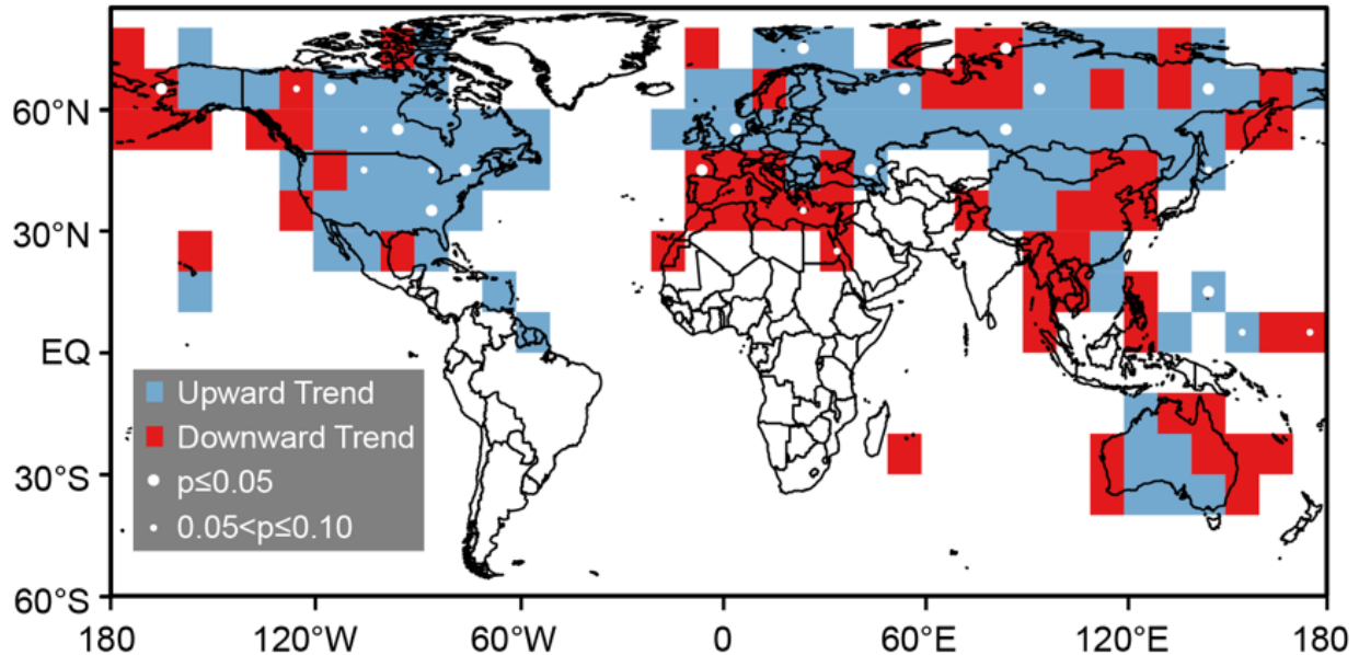
Figure 13. The 1951–2014 trend of the number of 5-day total precipitation events exceeding the station-specific threshold for an average 10-yr recurrence interval. White dots indicate that the trend is significant at the 0.05 < p \leq 0.10 (small dots) or p \leq 0.05 (large dots) level.
