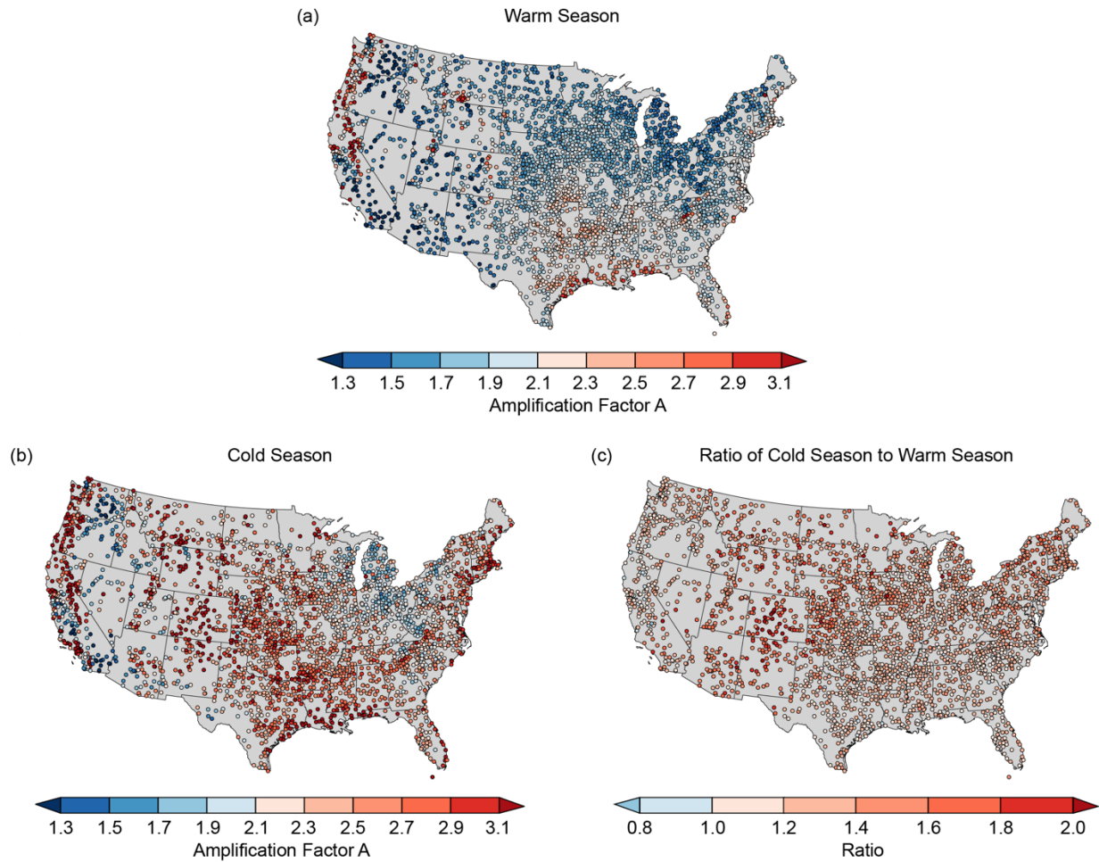
Figure 24. Average amplification factor ( A ) for each station for precipitation events exceeding the 1-yr, 1-day threshold for (a) warm season, (b) cold season, and (c) cold-to-warm season ratio of A .
