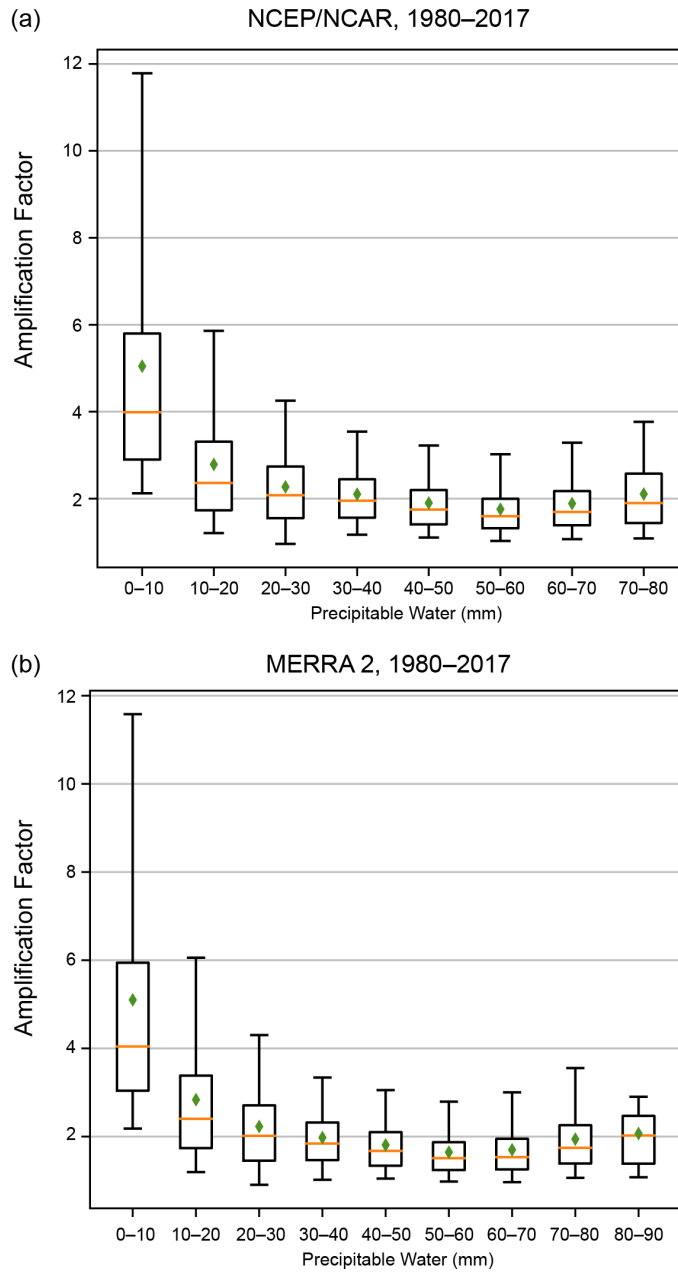
Figure A6. Boxplot distributions for the 1-yr, 1-day PDS of the amplification factor A ( EP/PW ) for (a) NCEP/NCAR, 1980–2017, and (b) MERRA-2, 1980–2017. Boxplot parameters include mean (green diamonds), median (orange horizontal lines), 25th and 75th percentiles (box limits), and 5th and 95th percentiles (whiskers).
