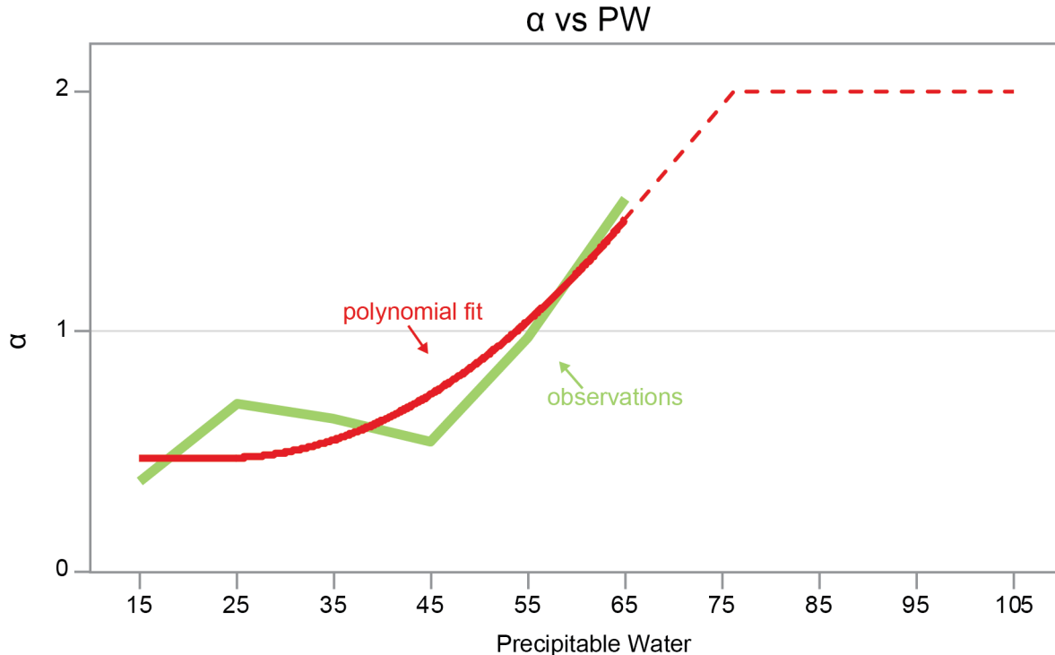
Figure 21. Observed and fitted relationship between PW and \alpha . These are the values of \alpha that are used in the CAUSES equation (3).
