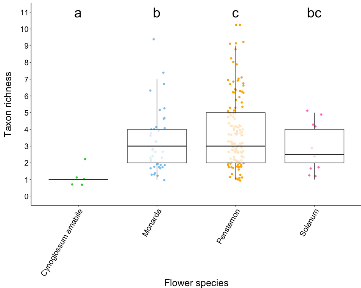
Figure 6. Boxplot showing the number of taxa detected in eDNA samples from different flower species. Taxon richness was significantly different in relation to flower species. Boxes show 25th, 50th, and 75th percentiles, and whiskers show 5th and 95th percentiles.
