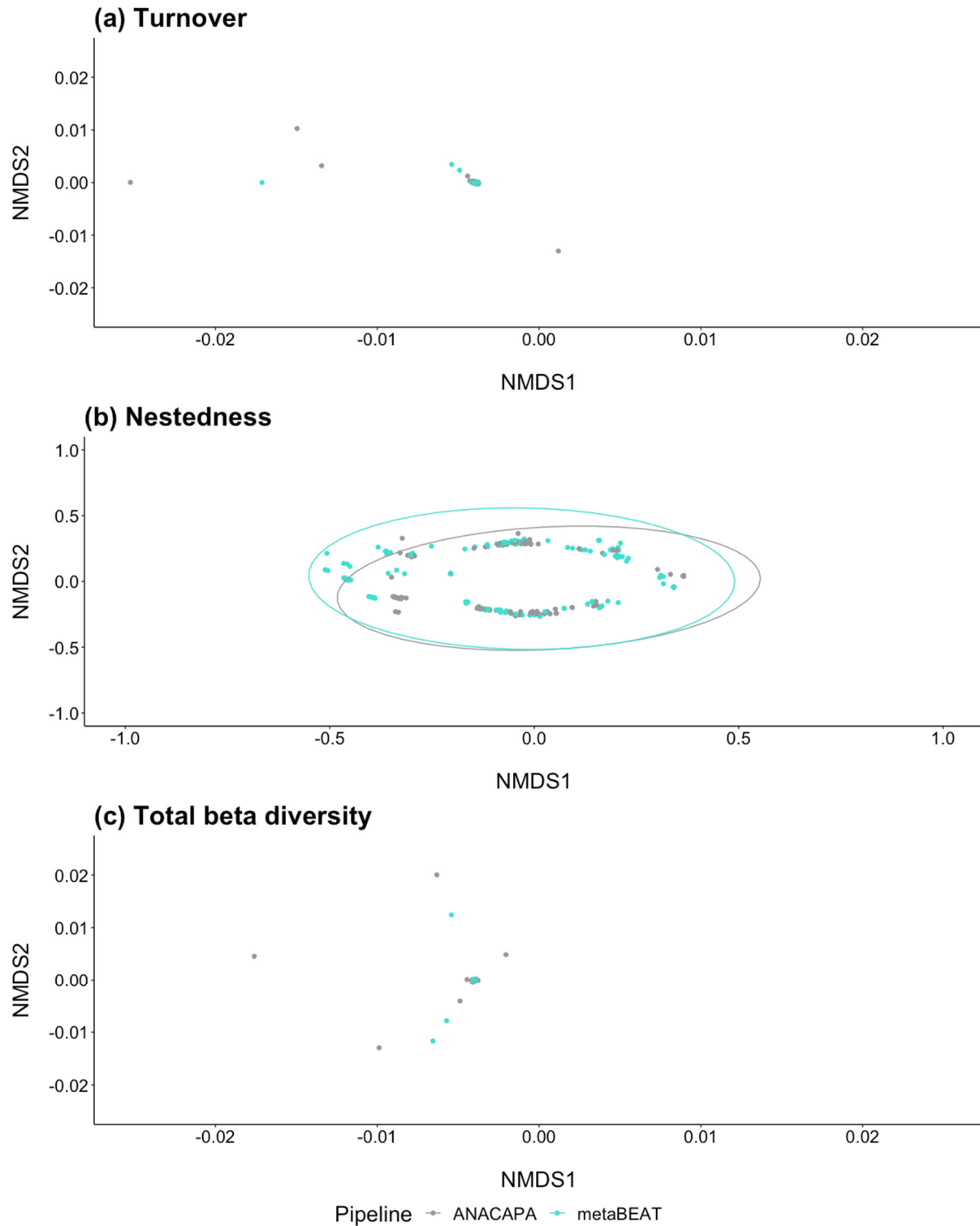
Figure 15. Non-metric Multidimensional Scaling (NMDS) plots of communities (Jaccard dissimilarity) produced by different bioinformatics pipelines (colored points/ellipse). The turnover (a) and nestedness (b) partitions of total beta diversity (c) are shown.
