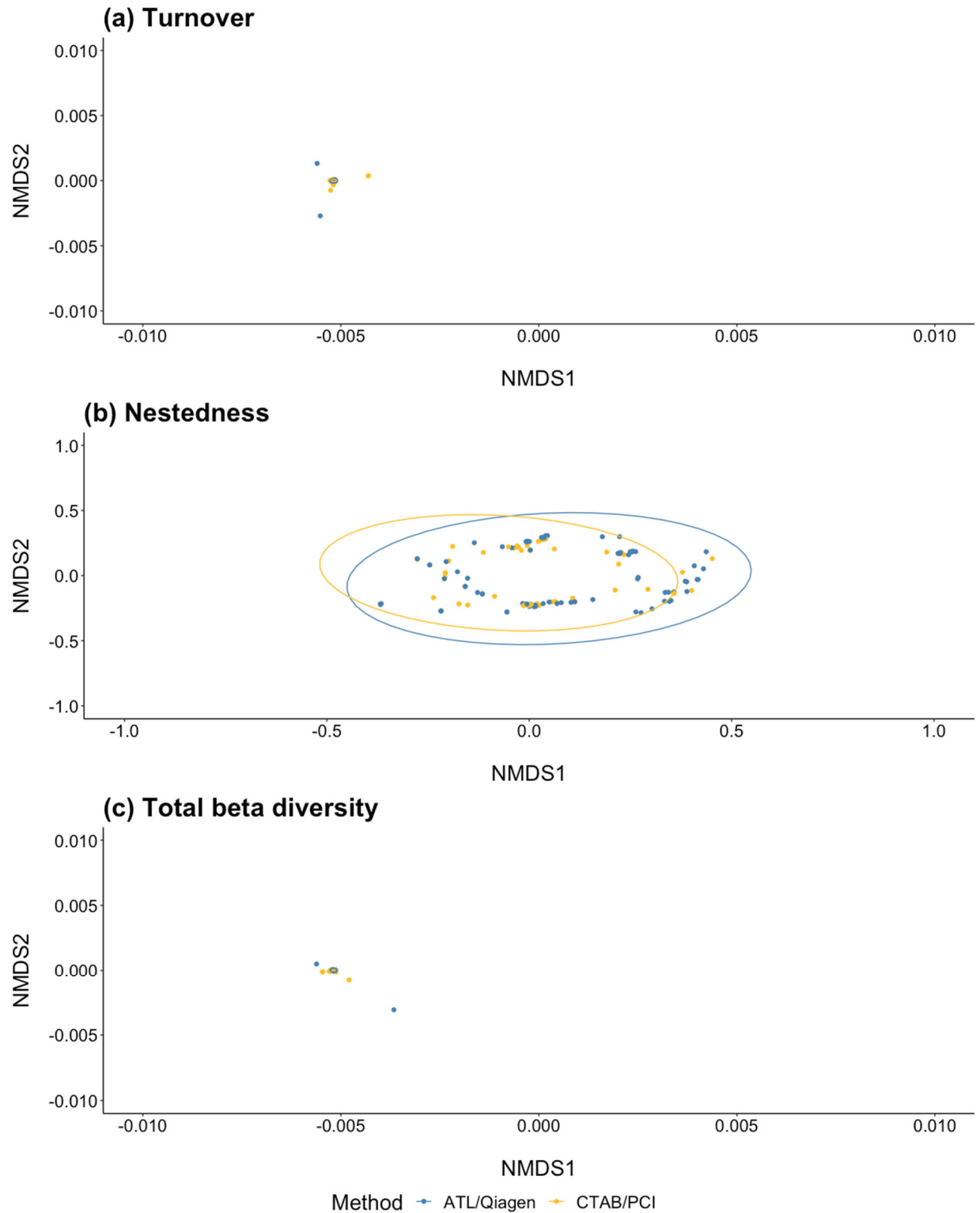
Figure 11. Non-metric Multidimensional Scaling (NMDS) plots of communities (Jaccard dissimilarity) produced by different preservation/extracton methods (colored points/ellipse). The turnover (a) and nestedness (b) partitions of total beta diversity (c) are shown.
