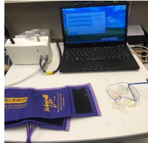
Figure 5: Prototype device to measure central venous pressure non-invasively using bioimpedance
