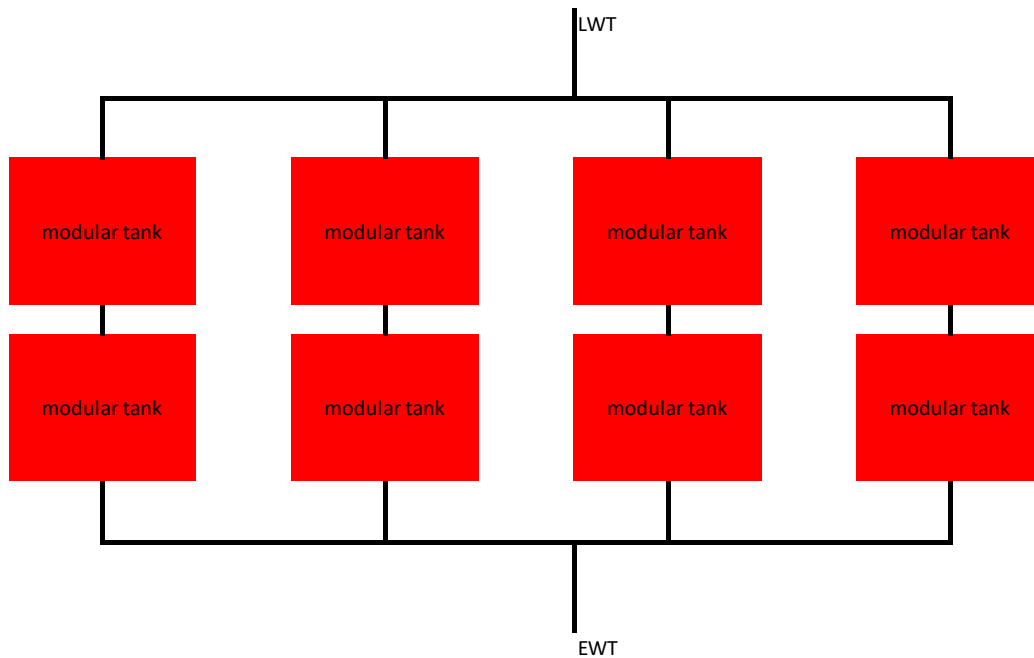
Figure 17. Schematic Diagram for the Circuit of the Tanks for Phase 2.
