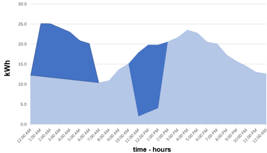
Figure 28. Daily (June) Load Profile for B1020 with TES
