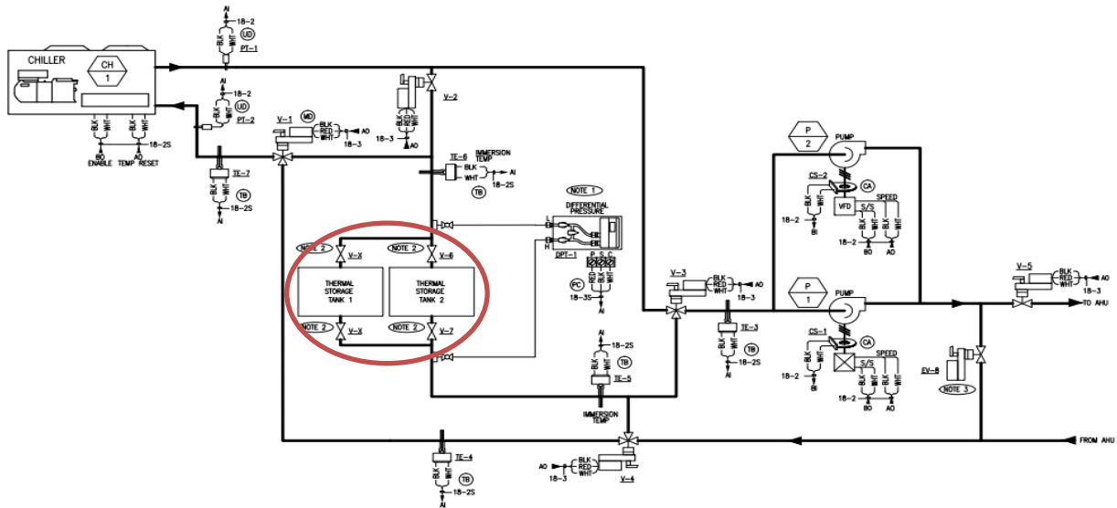
Figure 16. Schematic Diagram for the Integration of Thermal Storage Tanks.
