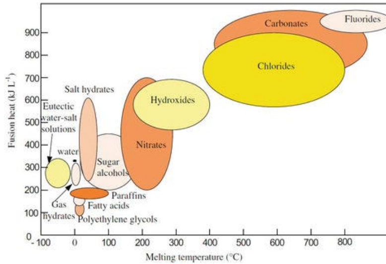
Figure 3. Melting Temperature and Heat of Fusion of Different Type of PCMs [Zhenjun et al. 2017]
