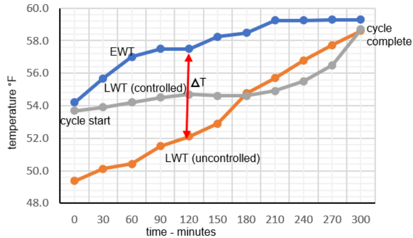
Figure 25. Daily Peak Period Melt (Discharge) Cycle
