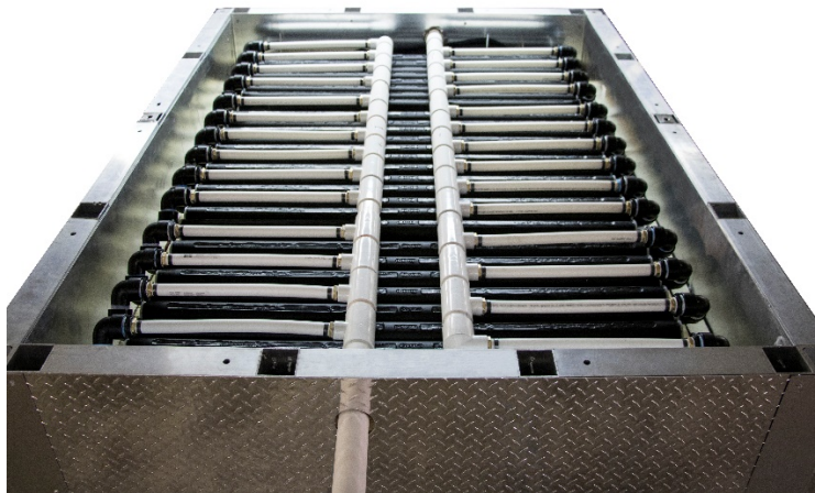
Figure 10. Top Sectional View of Heat-exchange Header and Manifold
