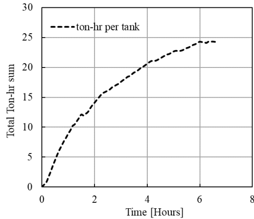
Figure 26. Verification of the Total Energy Capacity that Can Be Stored in One Tank
