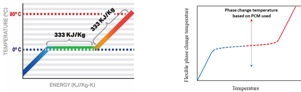
Figure 1. A Comparison between the Thermal Storage of Ice (left) and Flexible Thermal Storage Temperature PCMs (right)
