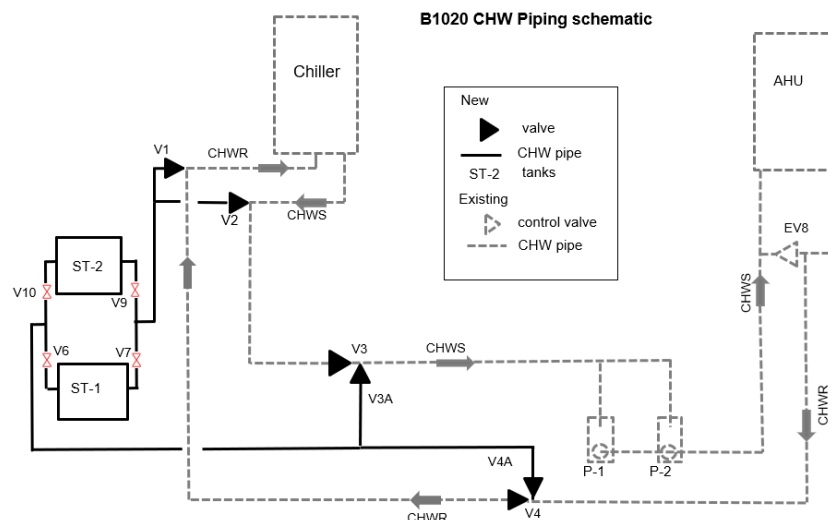
Figure 15. Revised Piping Schematic
