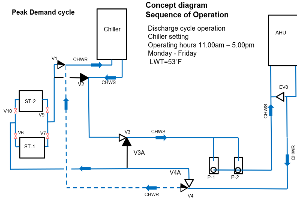
Figure 19. Diagrams Show the On-peak Sequence of Operations and Valve Control Strategy
