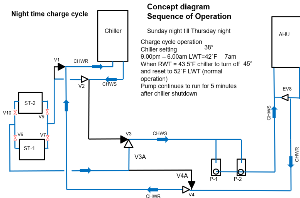
Figure 20. Diagrams Show the Charging Sequence of Operations and Valve Control Strategy
