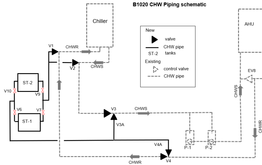
Figure 3. Revised Piping Schematic
