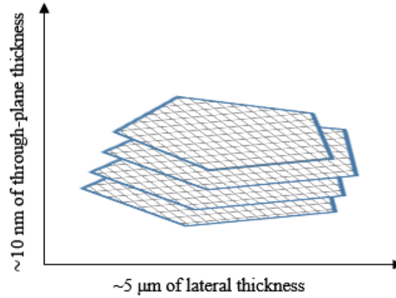
Figure 5. Schematic Diagram for a Stack of Nano Graphene Platelets (NGPs).
