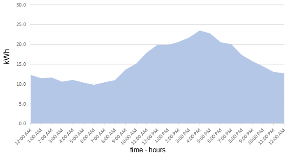
Figure 27. Typical Chiller Daily (June) Load Profile for B1020
