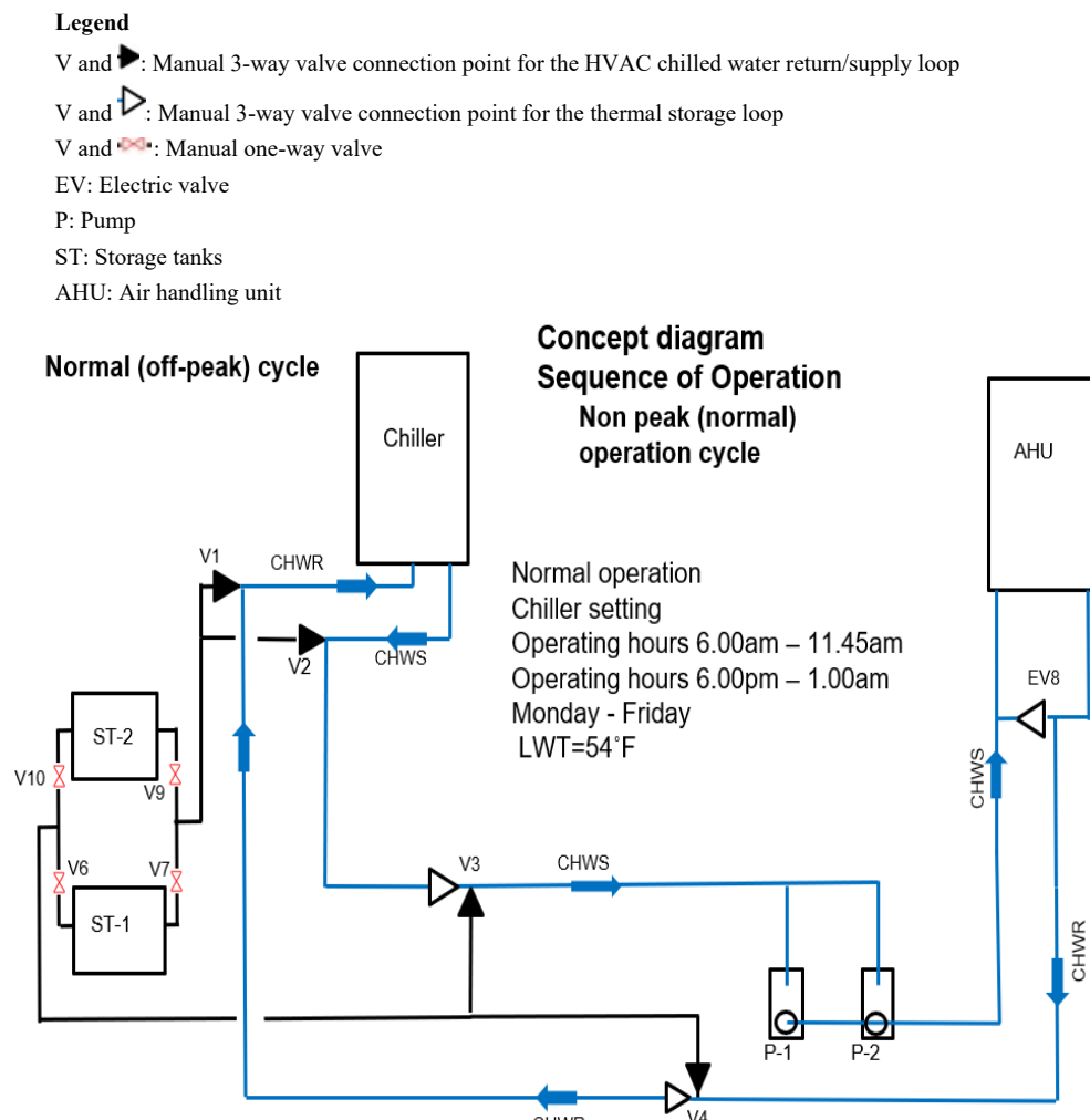
Figure 18. Diagrams Show the Off-peak Sequence of Operations and Valve Control Strategy
