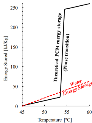
Figure 2. Performance Comparison between PCMs Latent Heat and Sensible Heat Energy Systems [Saeed et al. 2018]
