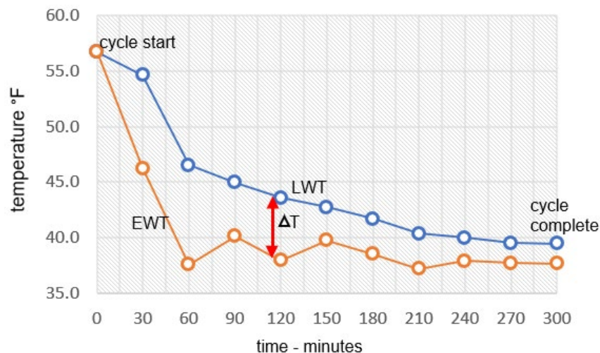
Figure 24. Daily Peak Period Melt (Discharge) Cycle
