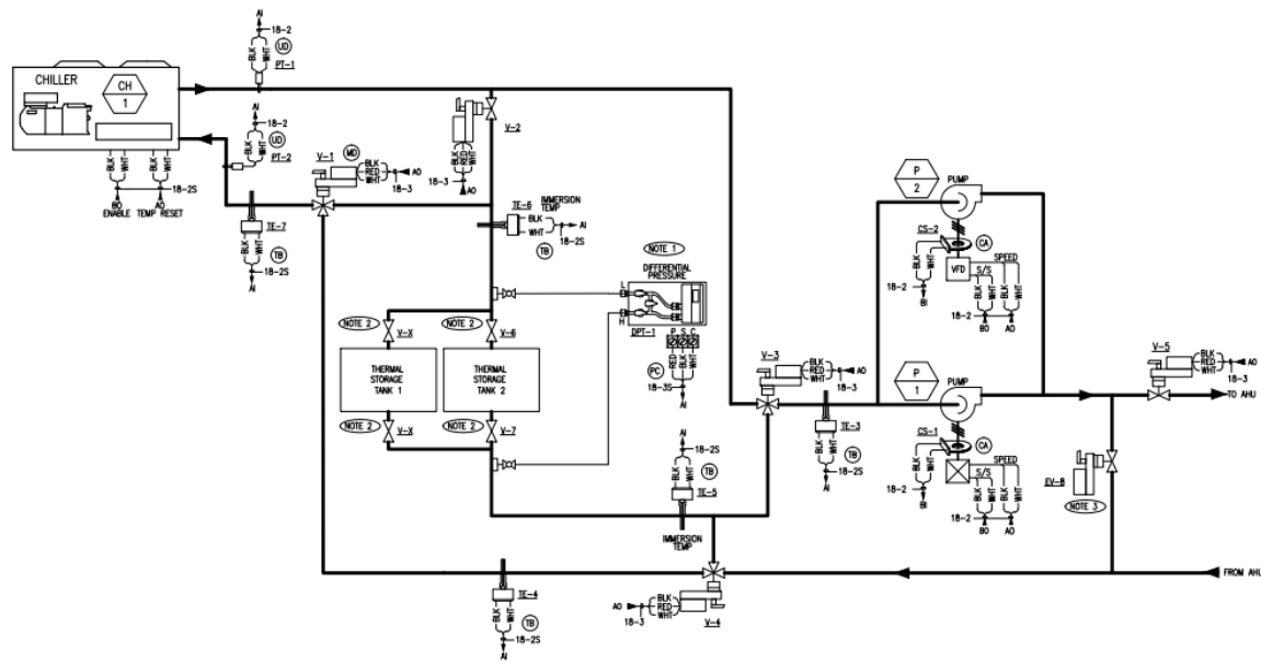
CHILLED WATER SYSTEM FLOW DIAGRAM
