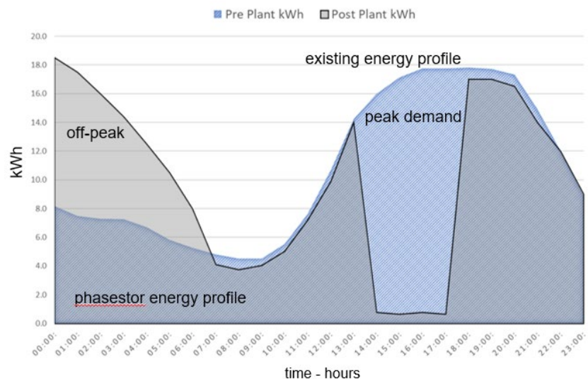
Figure 29. Reduced Energy Use During the Peak Demand Cycle.
