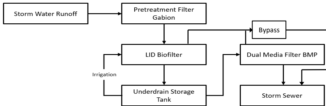
Figure 2-1. Technology Process Flow Diagram
