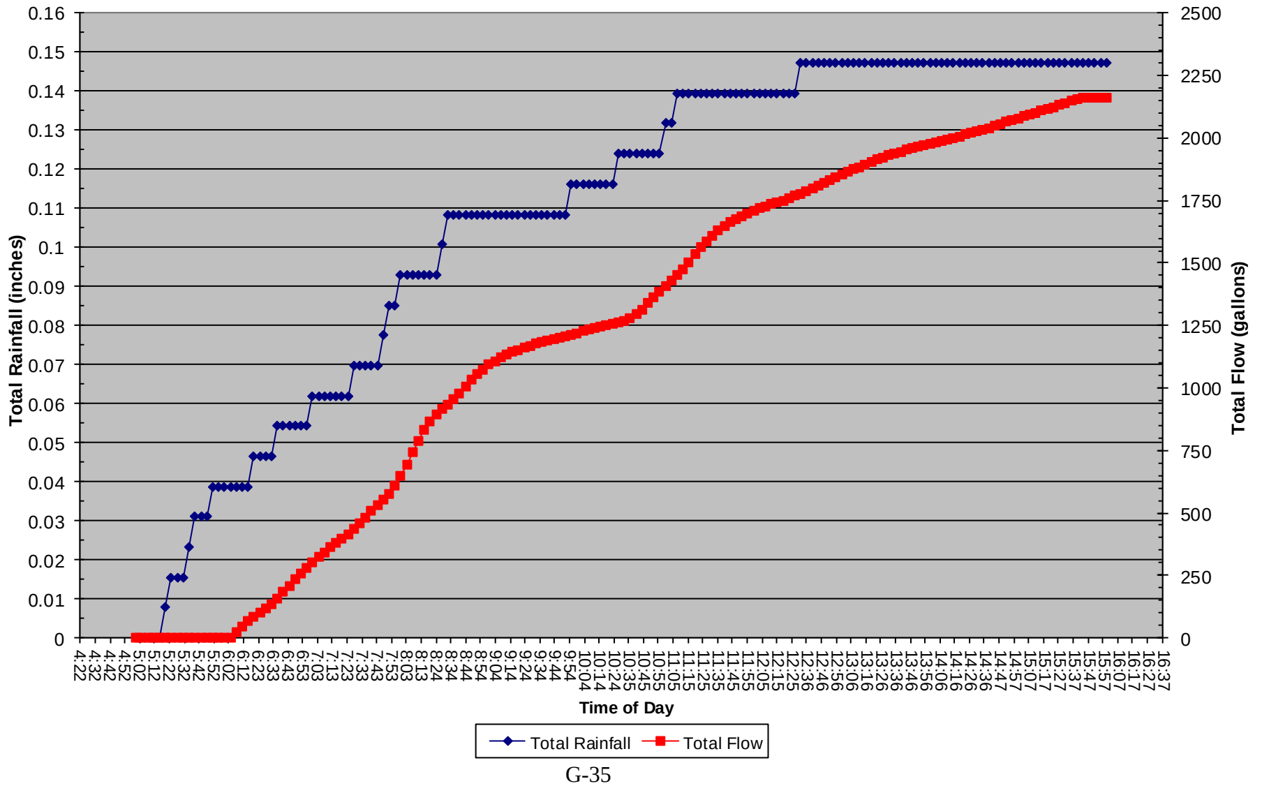
2 Mar 2019 Total Rainfall and Total Flow vs. Time of Day
