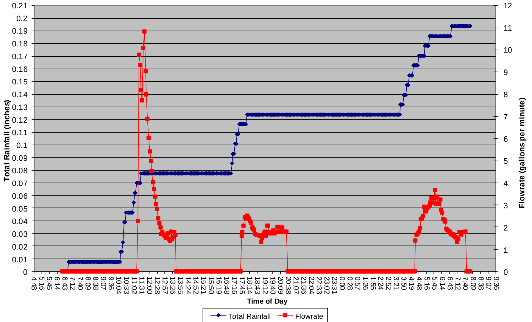
29 April 2019 Total Rainfall and Flowrate vs. Time of Day
