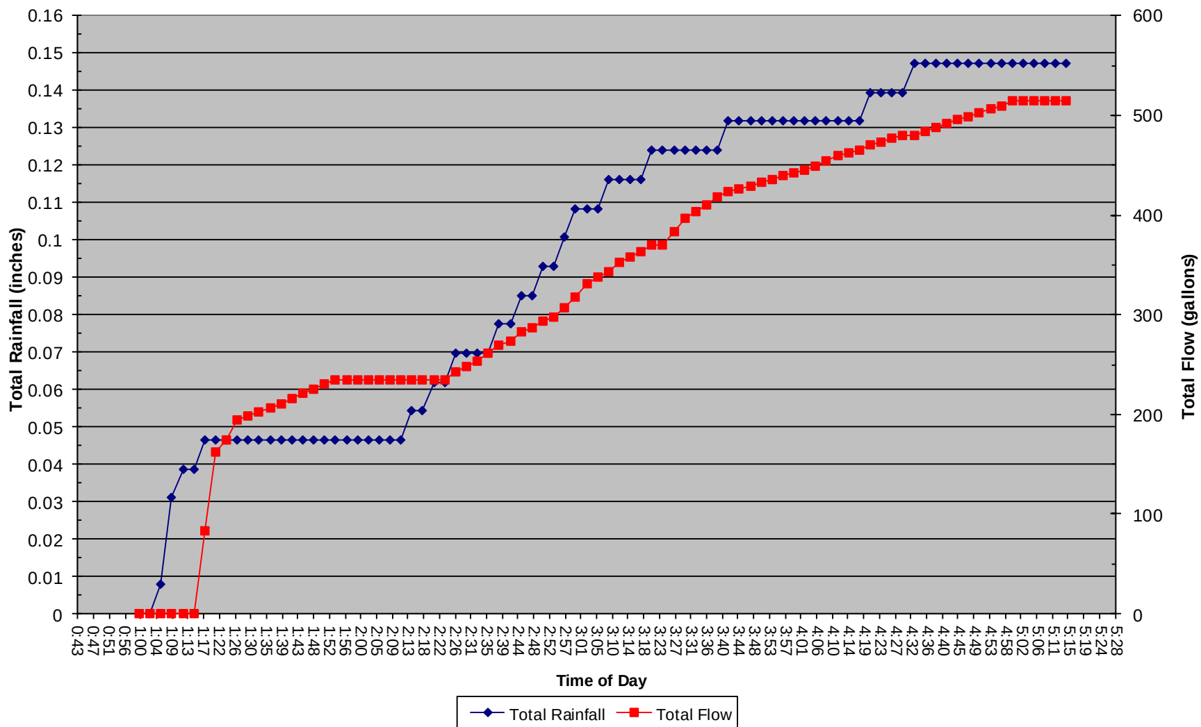
27 Feb 2018 Total Rainfall and Total Flow vs. Time of Day
