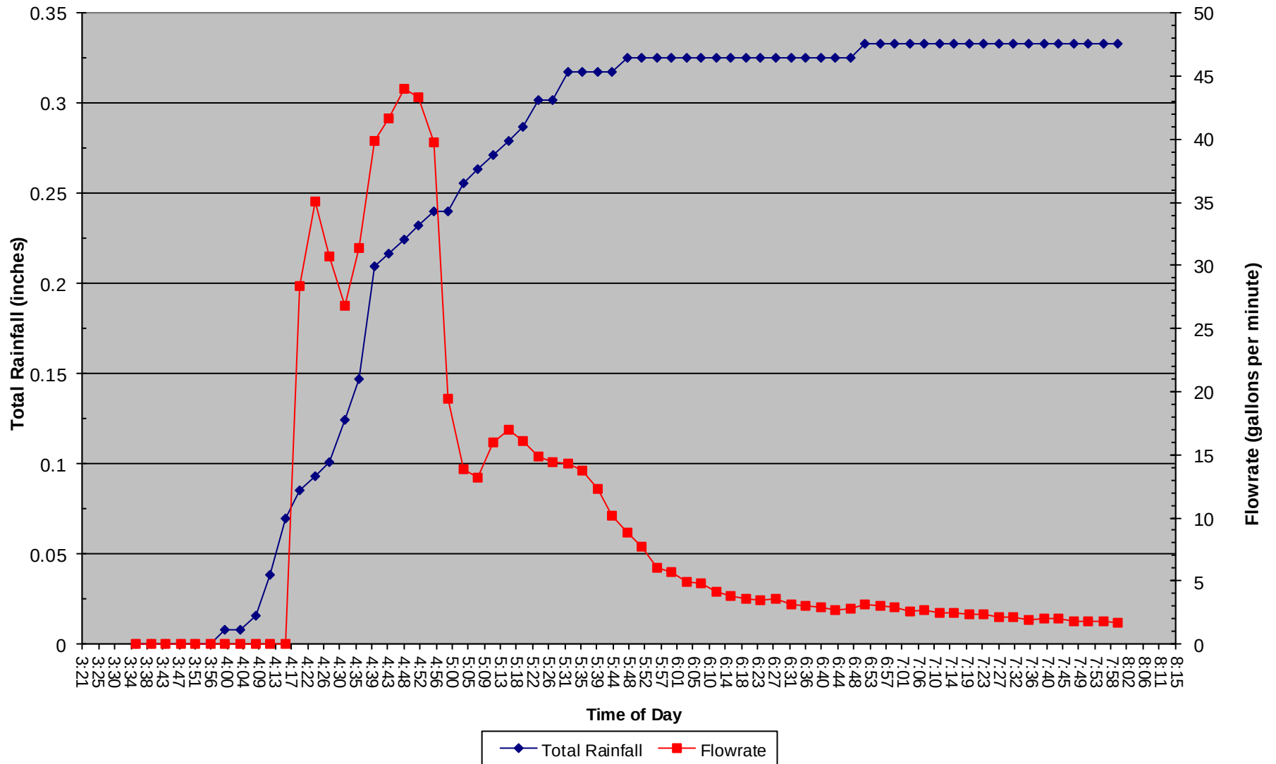
12 Jan 2019 Total Rainfall and Flowrate vs. Time of Day
