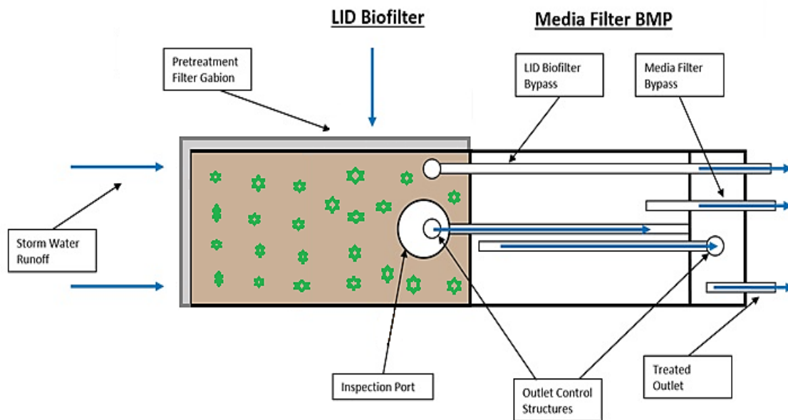
Figure 2-3. Conceptual Plan View Diagram for Hybrid LID / BMP System
