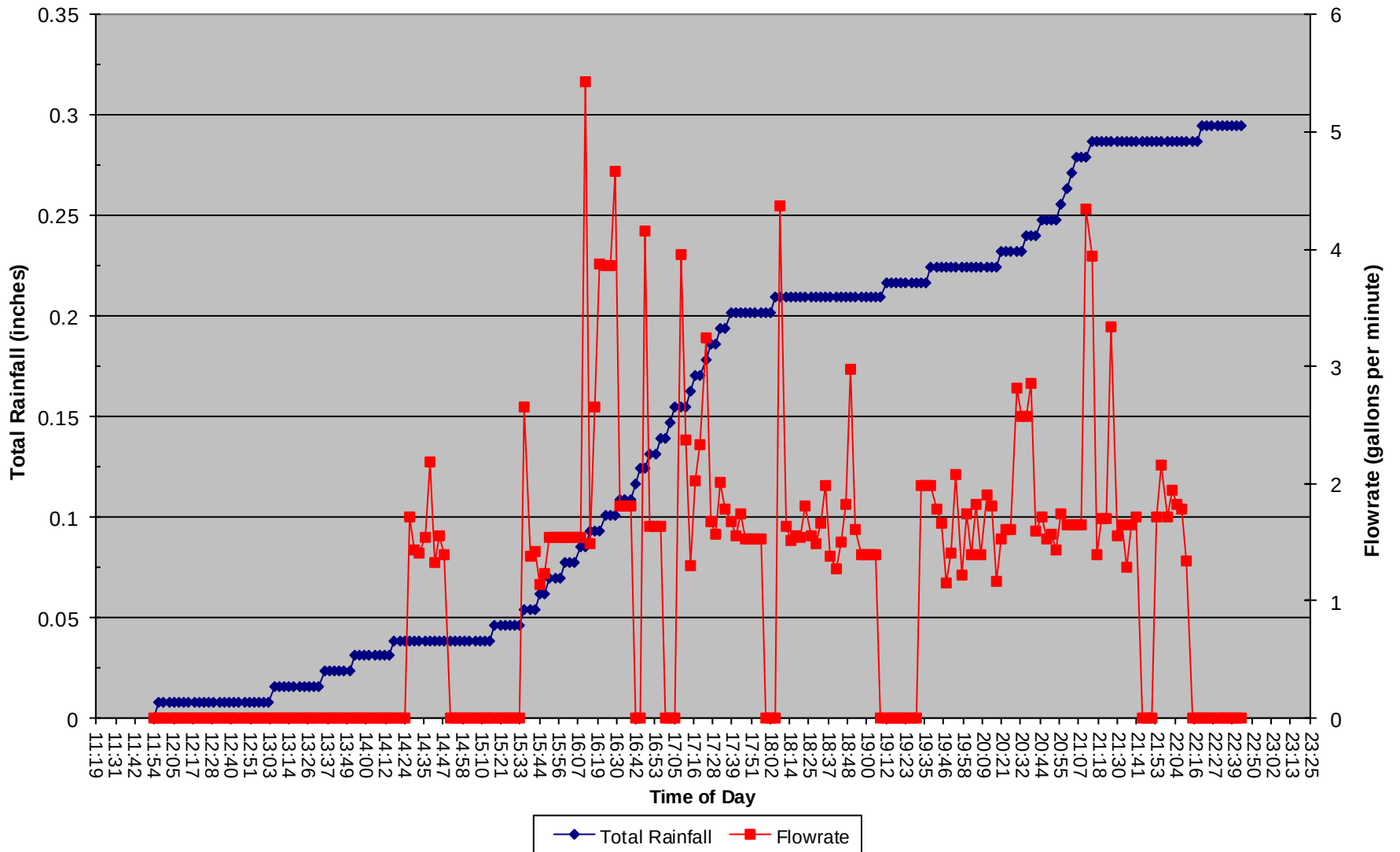
10 Mar 2018 Total Rainfall and Flowrate vs. Time of Day
