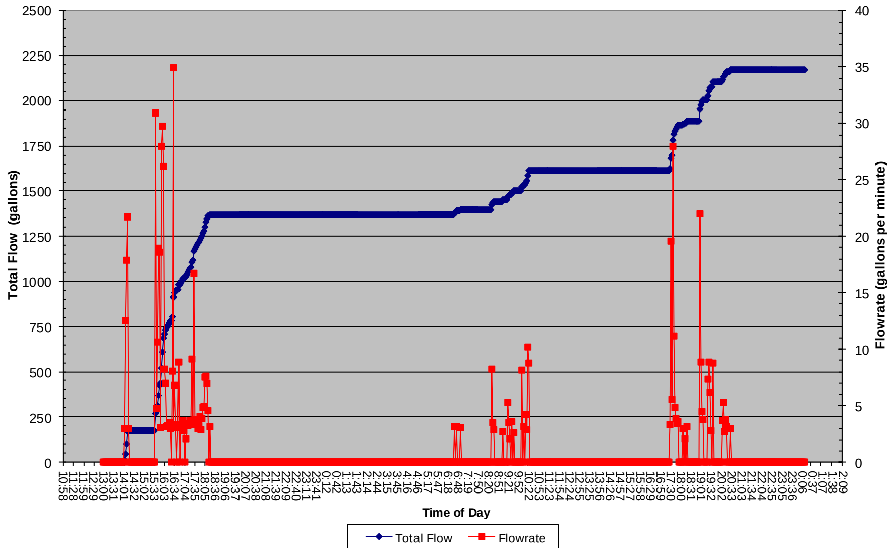
5 Dec 2018 Total Flow and Flowrate vs. Time of Day
