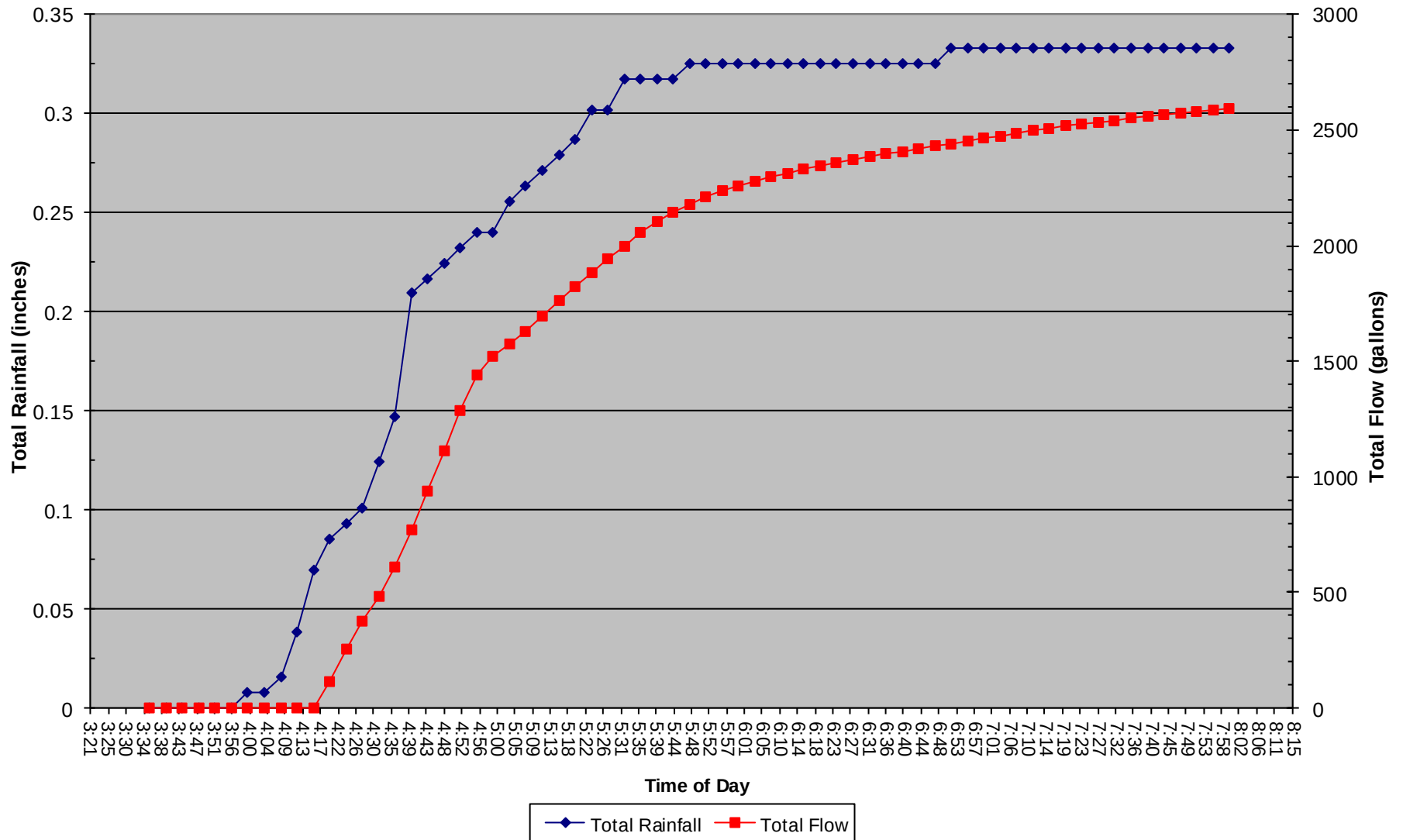
12 Jan 2019 Total Rainfall and Total Flow vs. Time of Day
