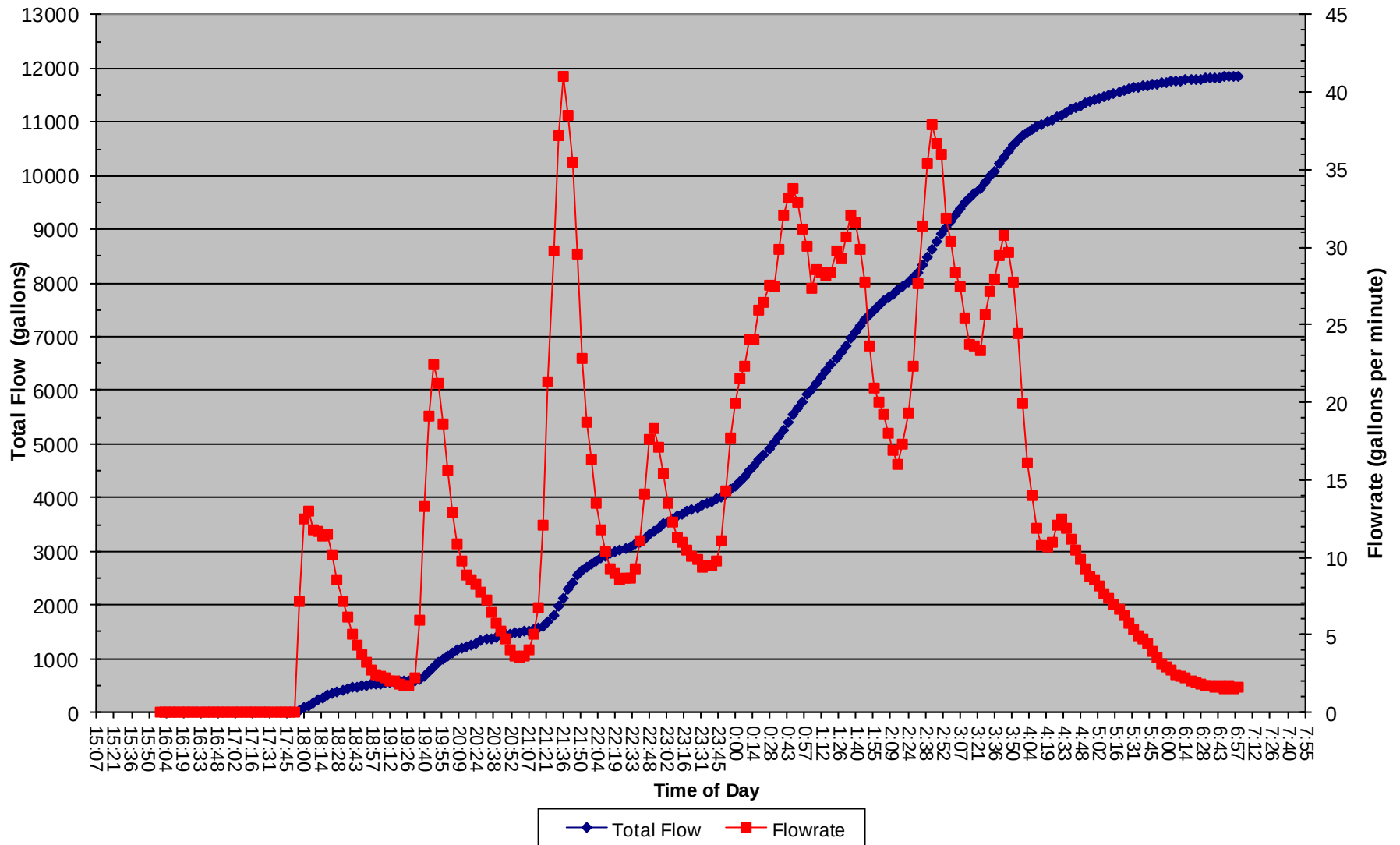
11 Mar 2019 Total Flow and Flowrate vs. Time of Day
