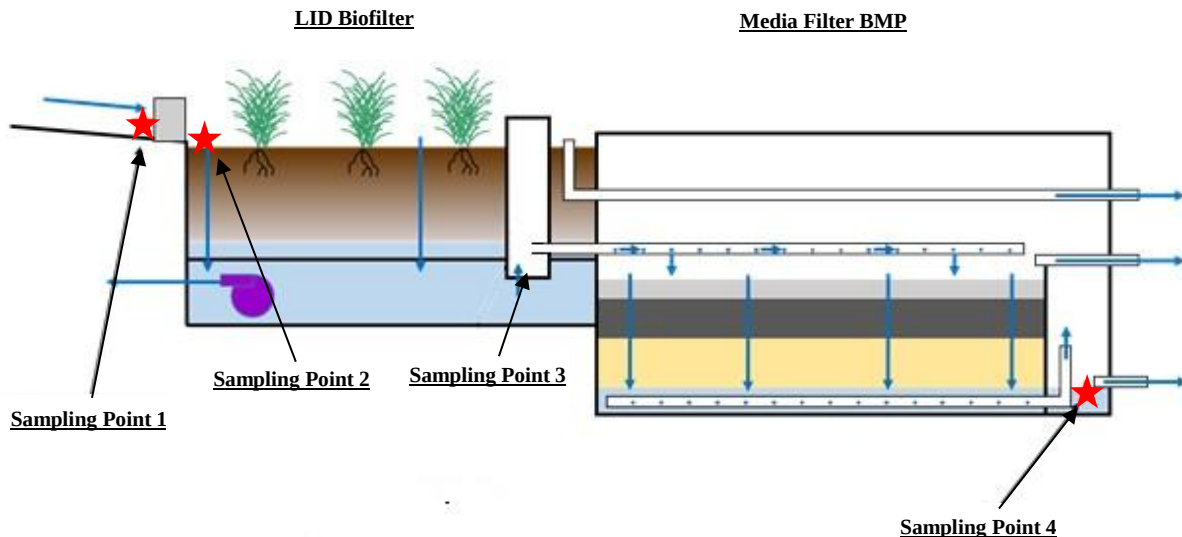
Figure E-1. Sampling Points on System
