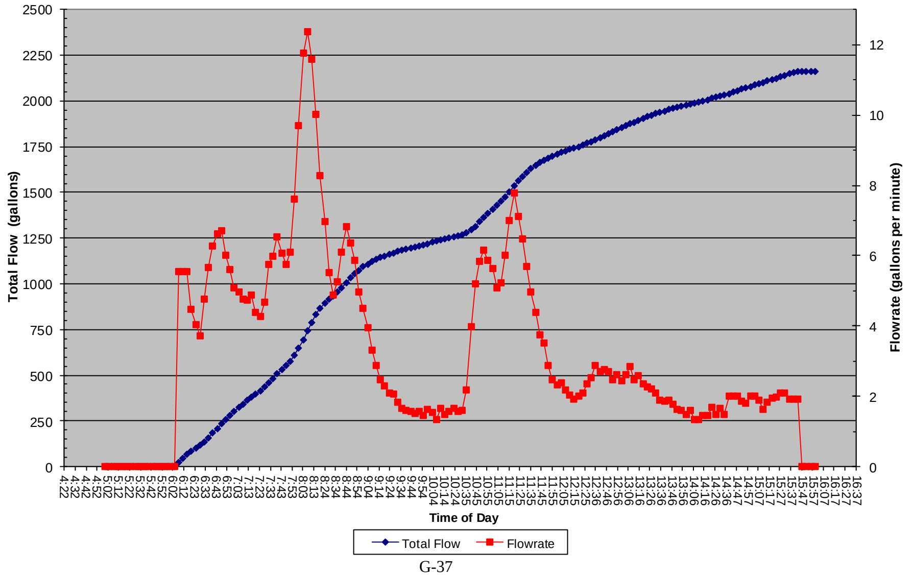
2 Mar 2019 Total Flow and Flowrate vs. Time of Day
