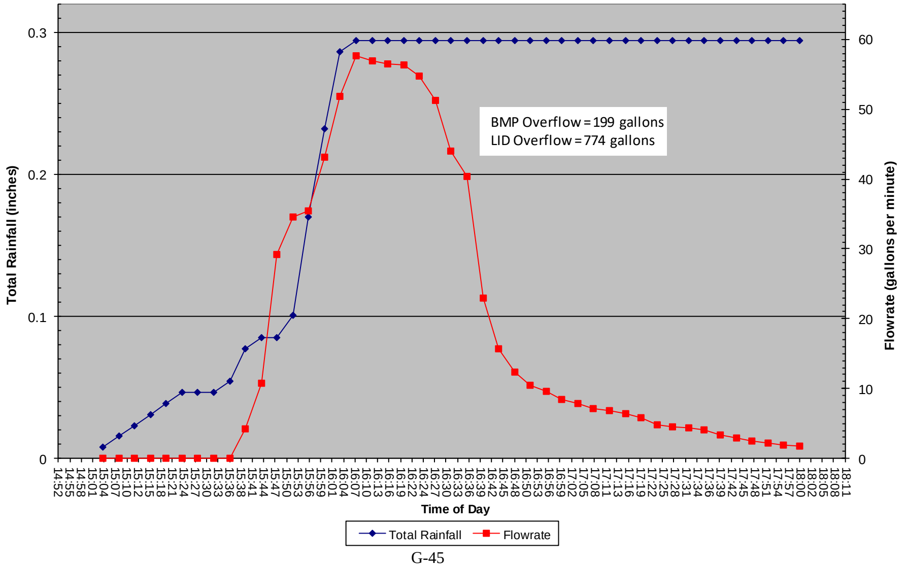
21 Mar 2019 Total Rainfall and Flowrate vs. Time of Day
