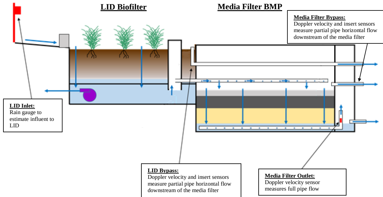
Figure 5-1. Layout of Flow Monitoring Equipment.
