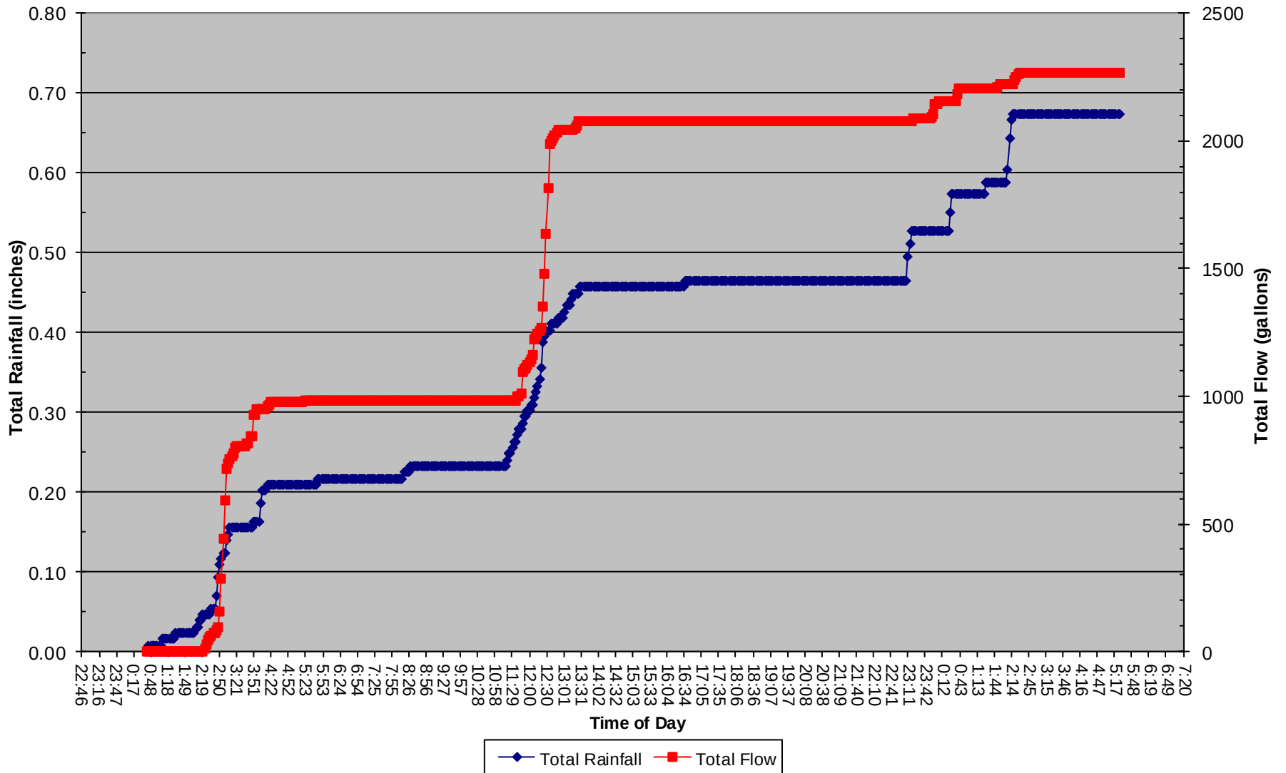
29 Nov 2018 Total Rainfall and Total Flow vs. Time of Day
