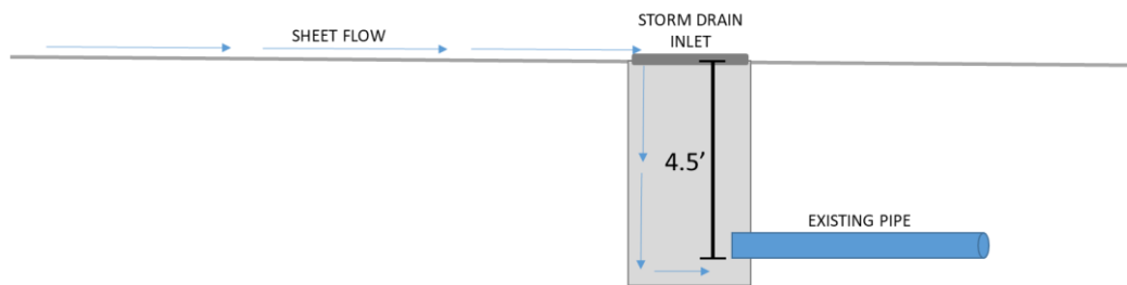
Figure 8-1. Typical Storm Drain Inlet Elevation Configuration
