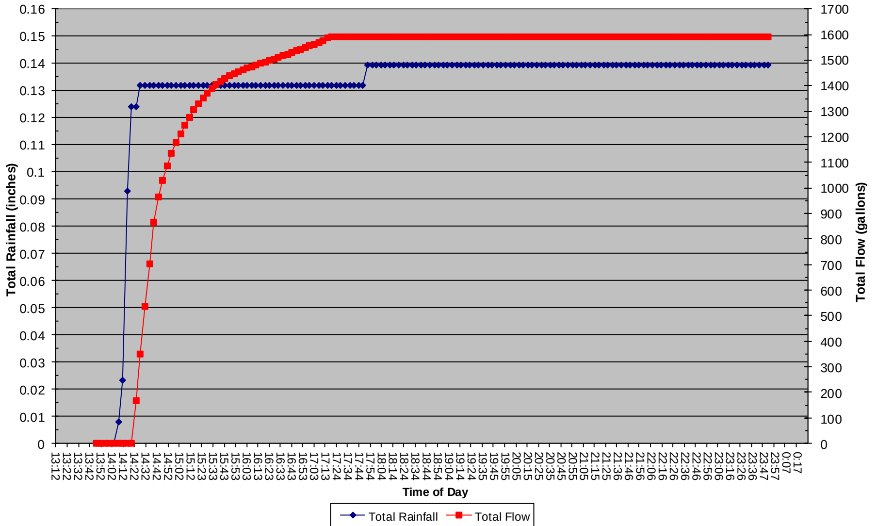
20 Mar 2019 Total Rainfall and Total Flow vs. Time of Day
