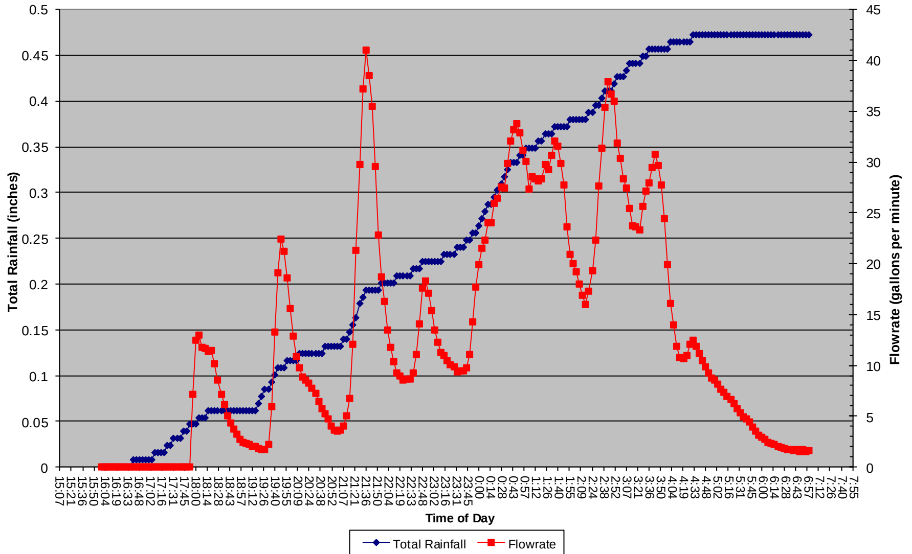
11 Mar 2019 Total Rainfall and Flowrate vs. Time of Day
