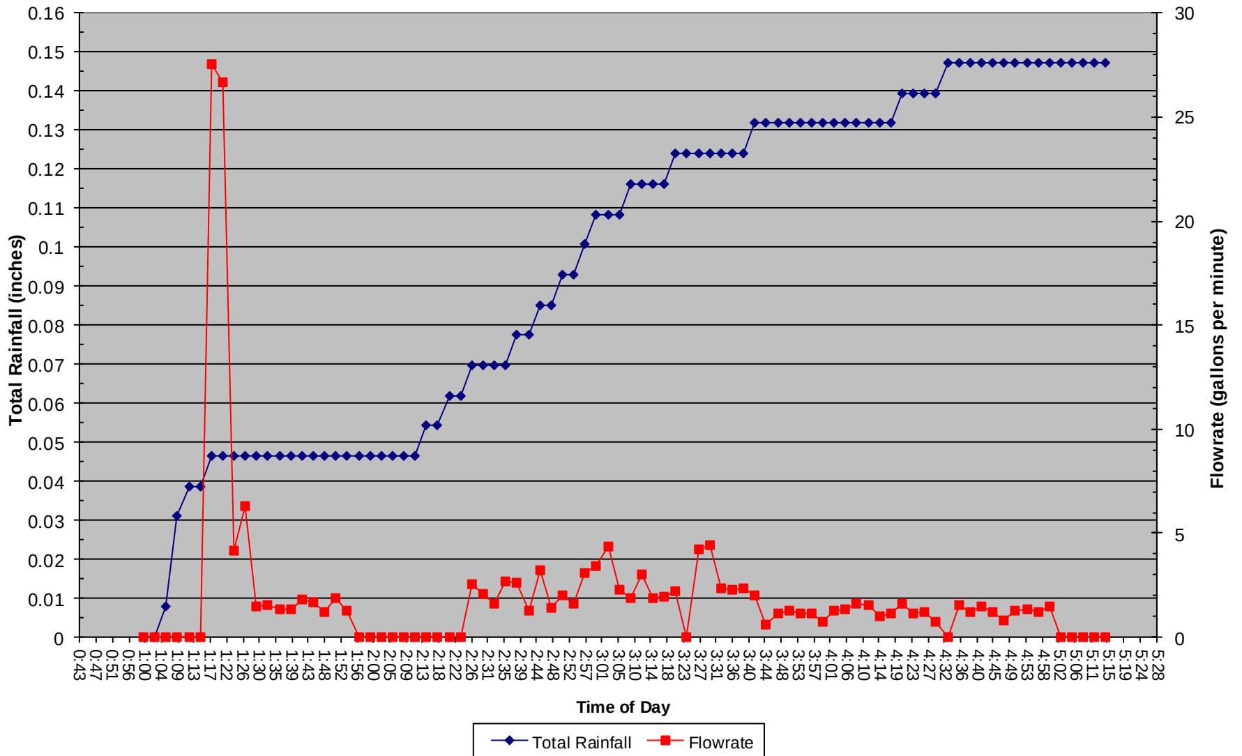
27 Feb 2018 Total Rainfall and Flowrate vs. Time of Day
