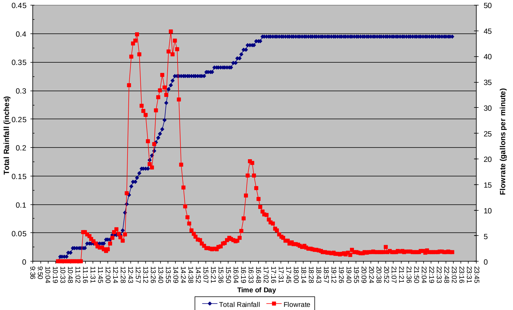
14 Jan 2019 Total Rainfall and Flowrate vs. Time of Day
