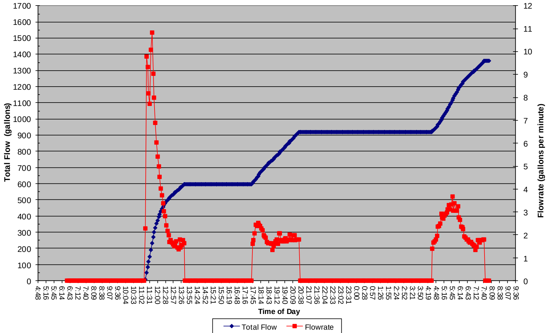
29 April 2019 Total Flow and Flowrate vs. Time of Day
