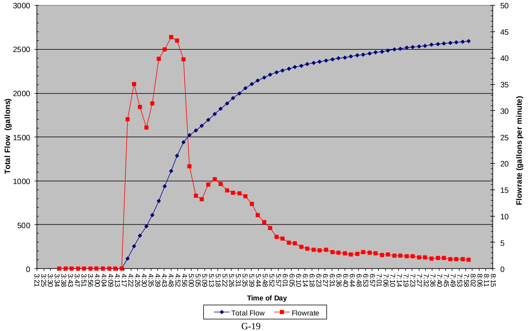
12 Jan 2019 Total Flow and Flowrate vs. Time of Day
