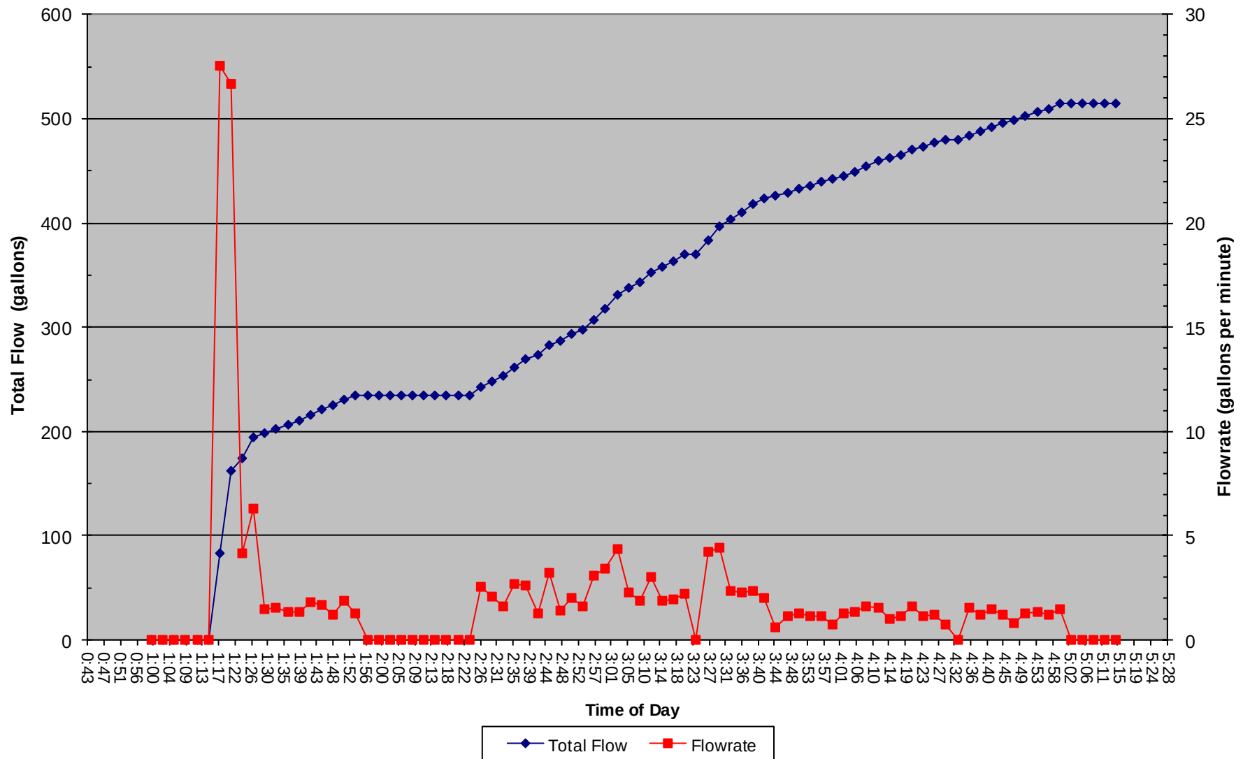
27 Feb 2018 Total Flow and Flowrate vs. Time of Day
