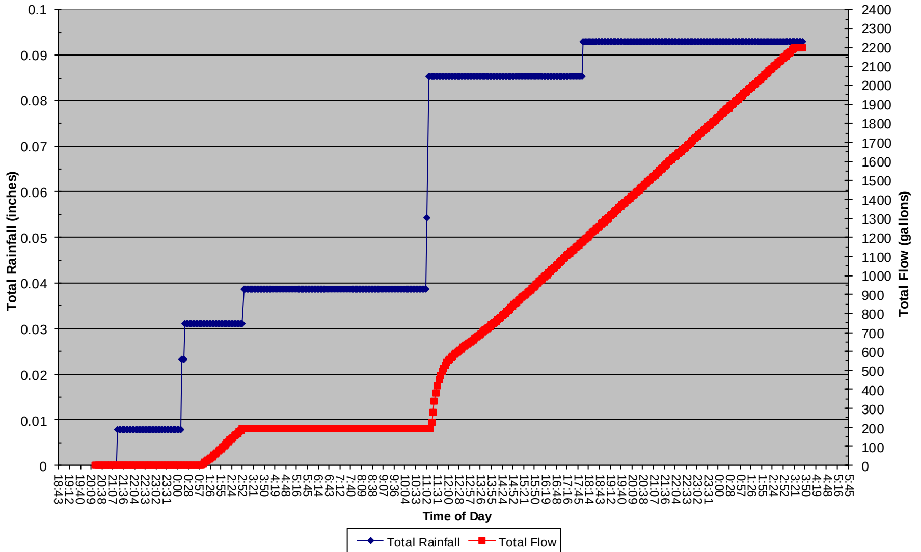
20 Feb 2019 Total Rainfall and Total Flow vs. Time of Day
