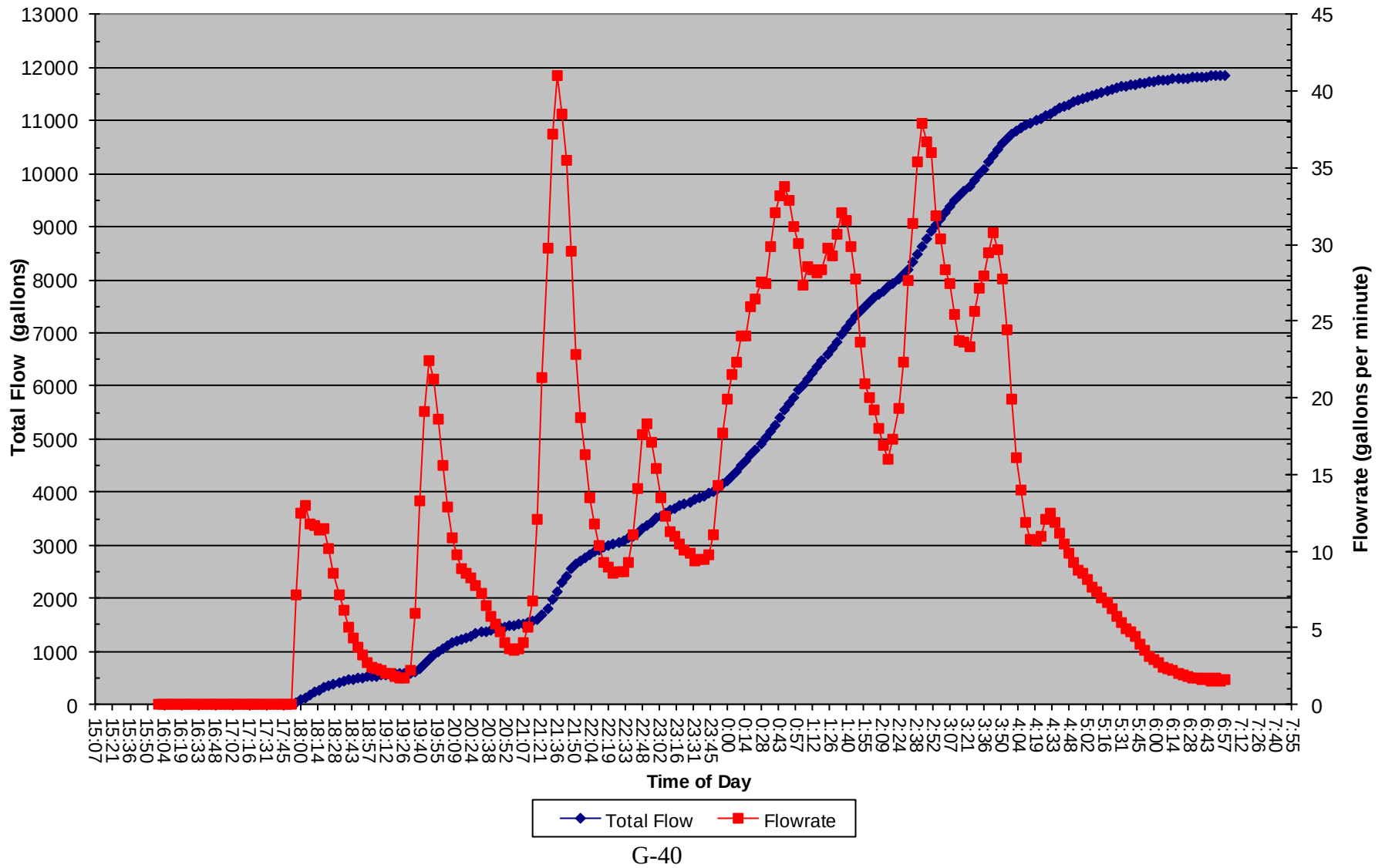
11 Mar 2019 Total Flow and Flowrate vs. Time of Day
