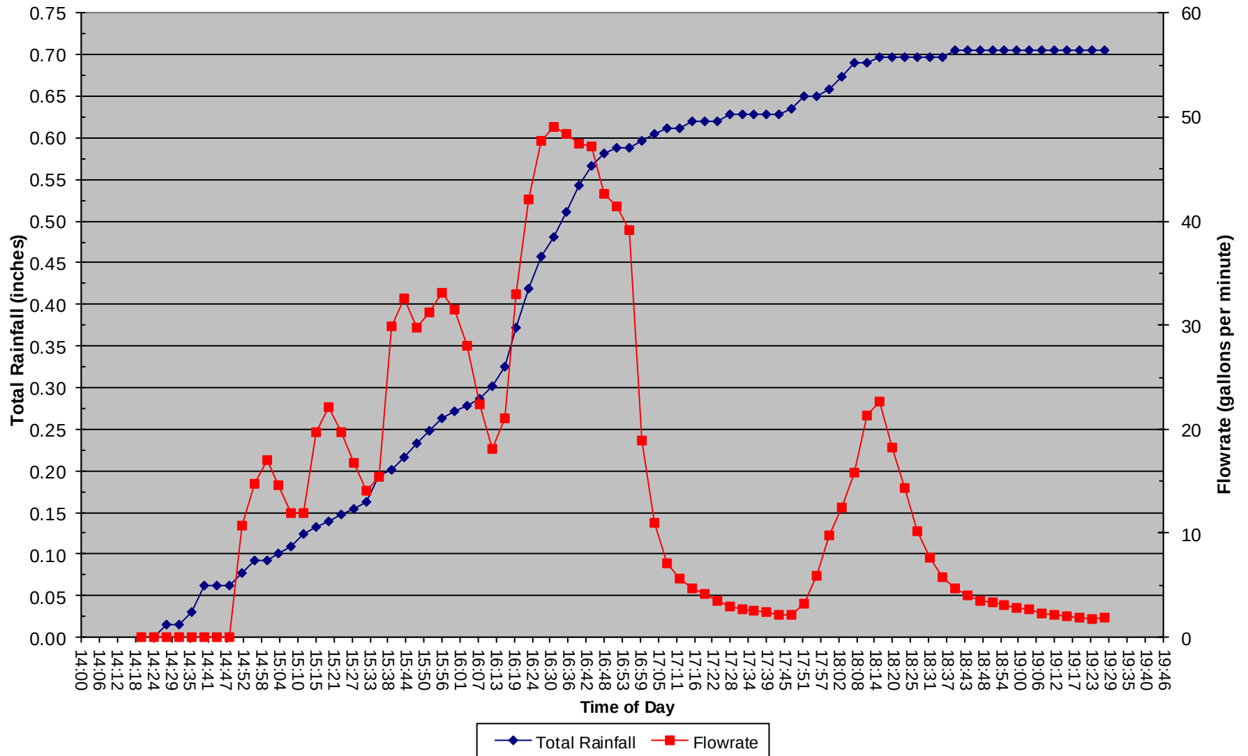
31 Jan 2019 Total Rainfall and Flowrate vs. Time of Day
