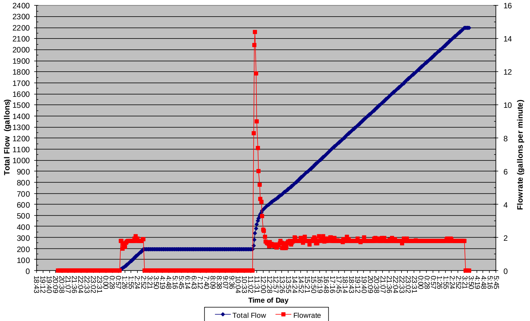
20 Feb 2019 Total Flow and Flowrate vs. Time of Day
