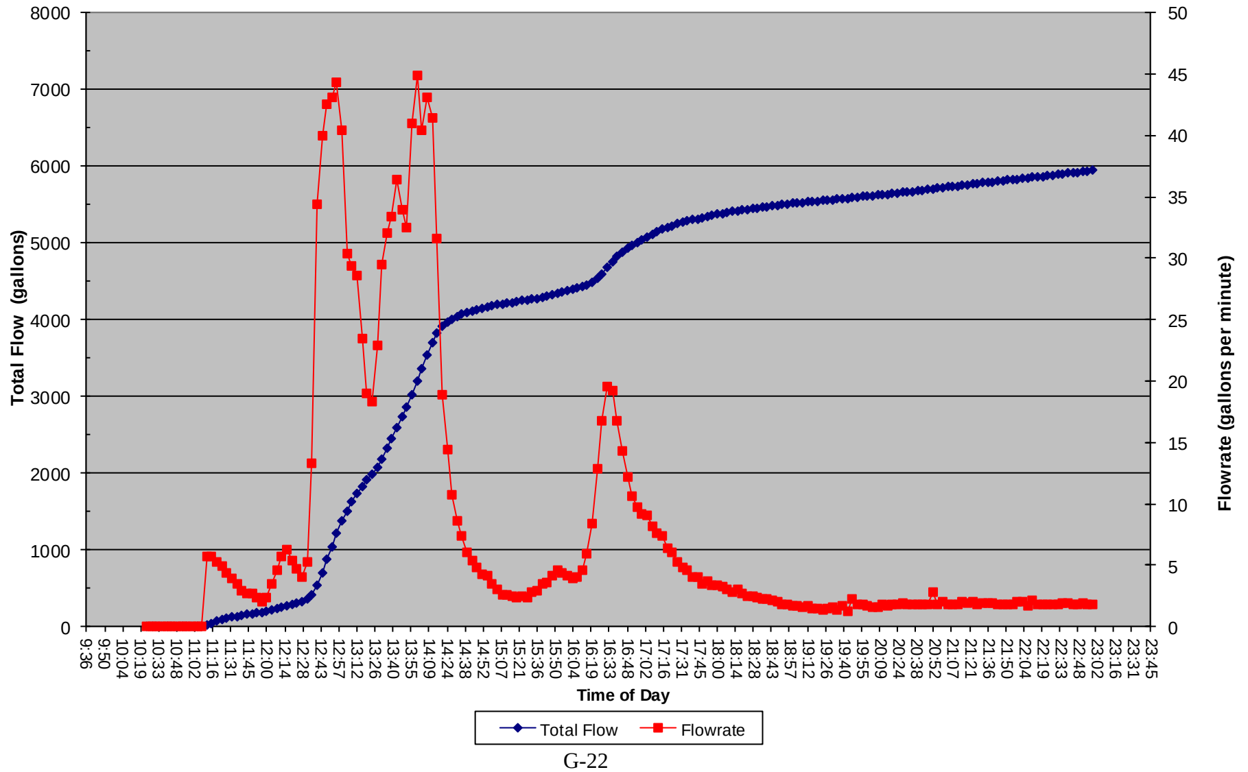
14 Jan 2019 Total Flow and Flowrate vs. Time of Day
