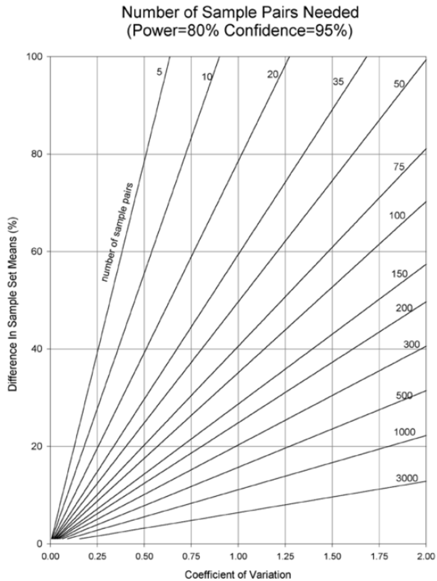
Figure 5-4. Number of Samples Required for 80% Power and 95% Statistical Significance
