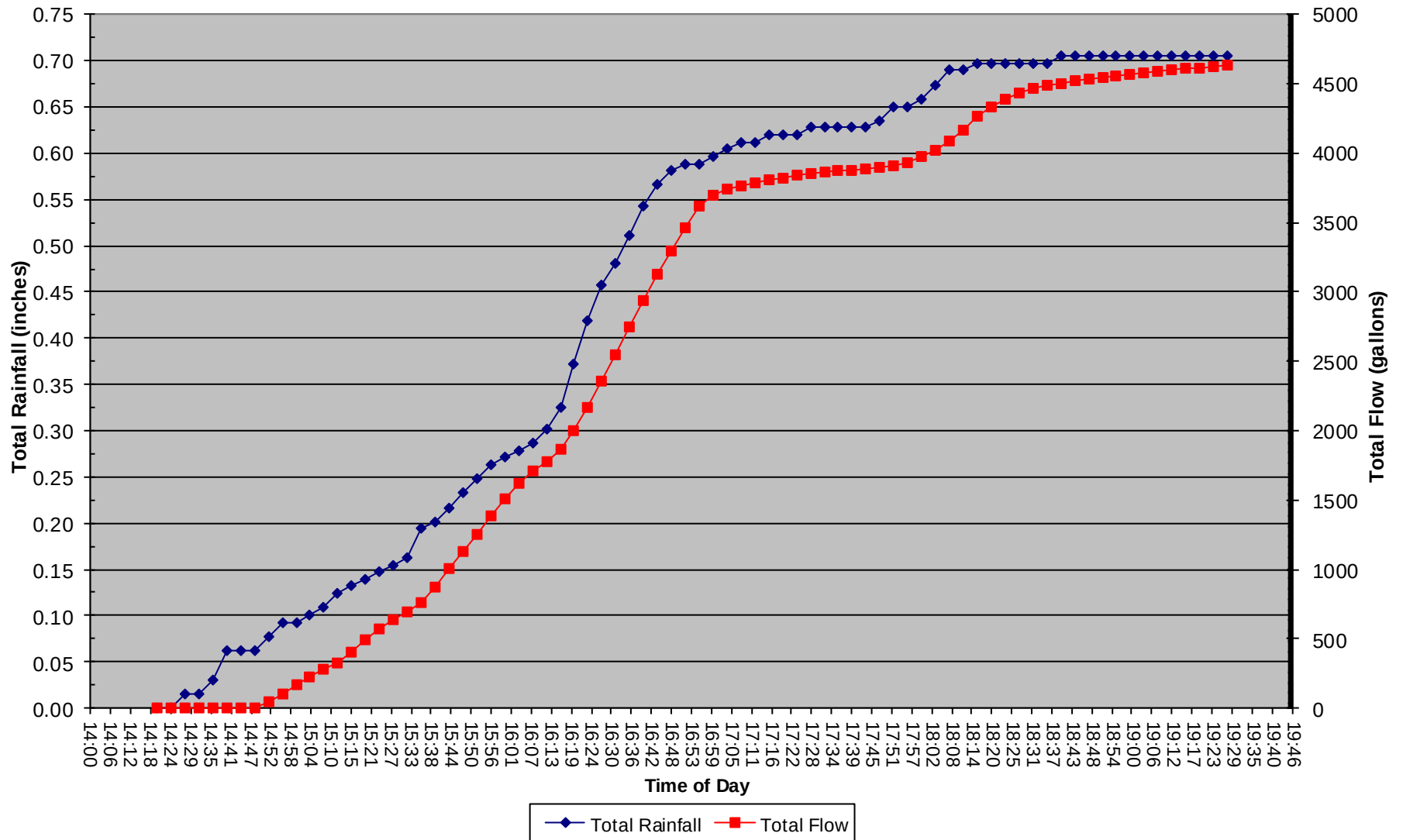
31 Jan 2019 Total Rainfall and Total Flow vs. Time of Day
