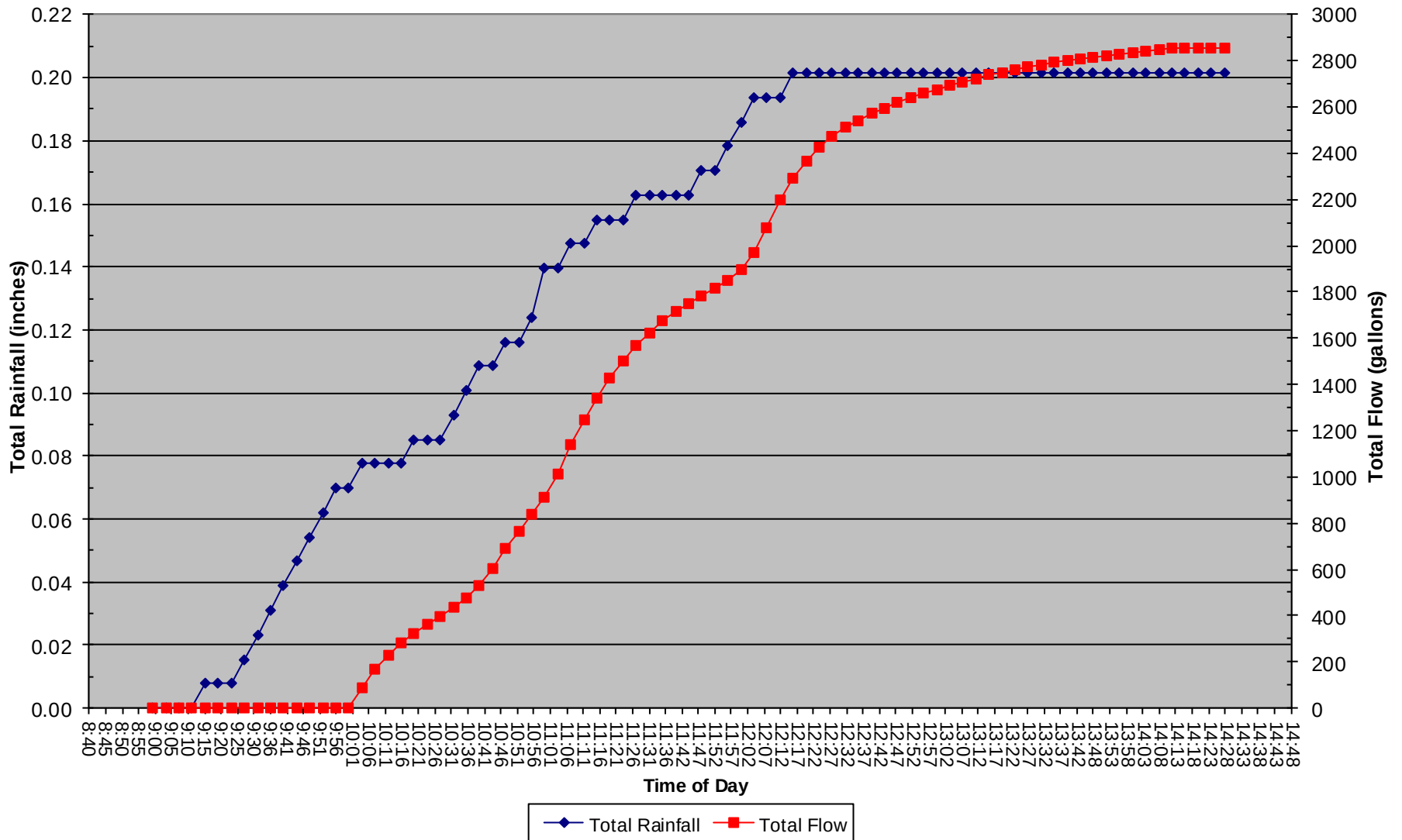
19 May 2019 Total Rainfall and Total Flow vs. Time of Day
