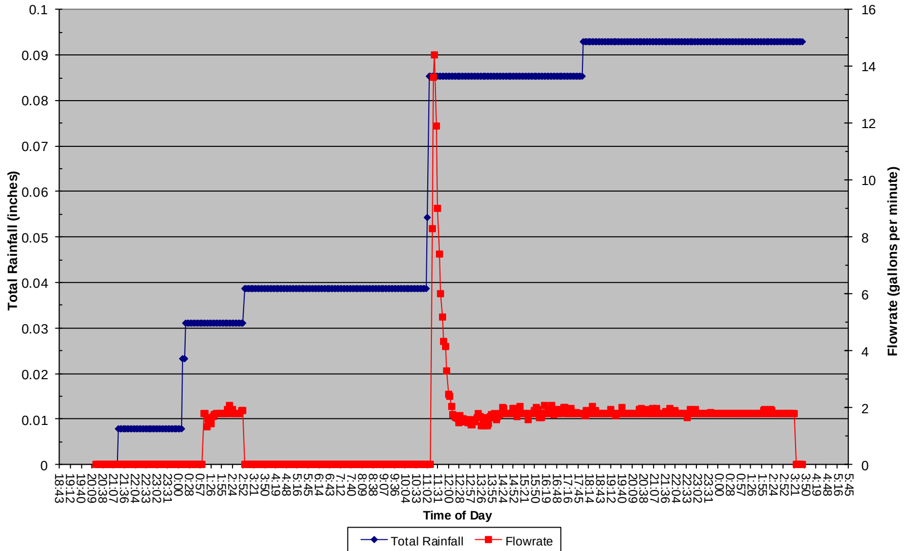
20 Feb 2019 Total Rainfall and Flowrate vs. Time of Day
