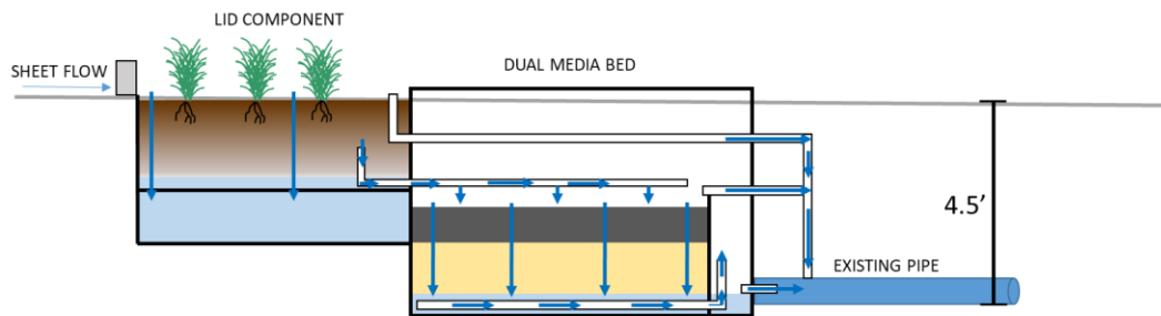
Figure 8-2. Hybrid LID/BMP Elevation Configuration
