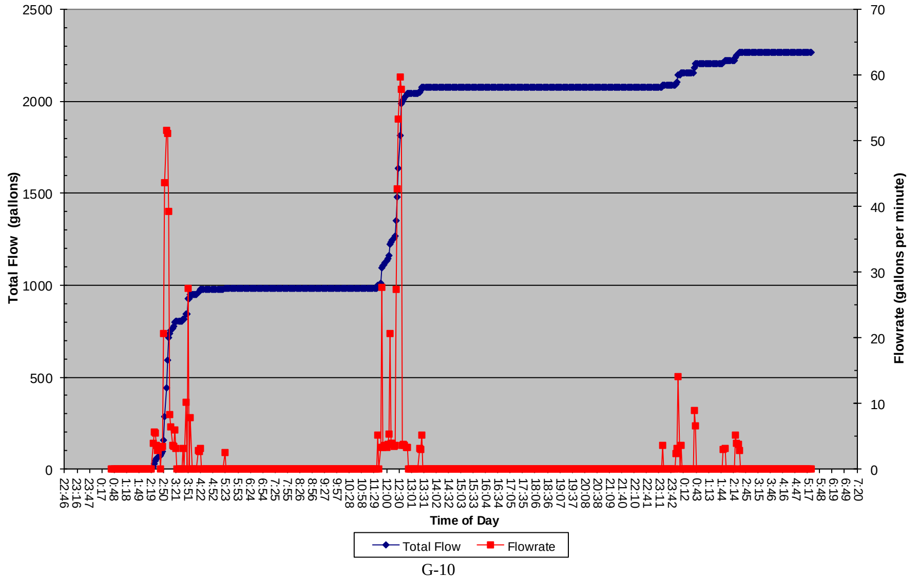
29 Nov 2018 Total Flow and Flowrate vs. Time of Day
