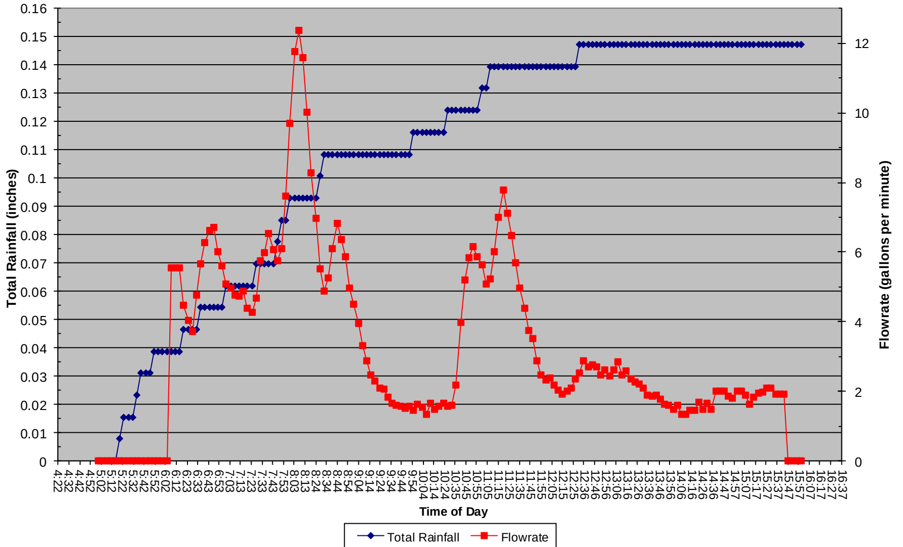
2 Mar 2019 Total Rainfall and Flowrate vs. Time of Day
