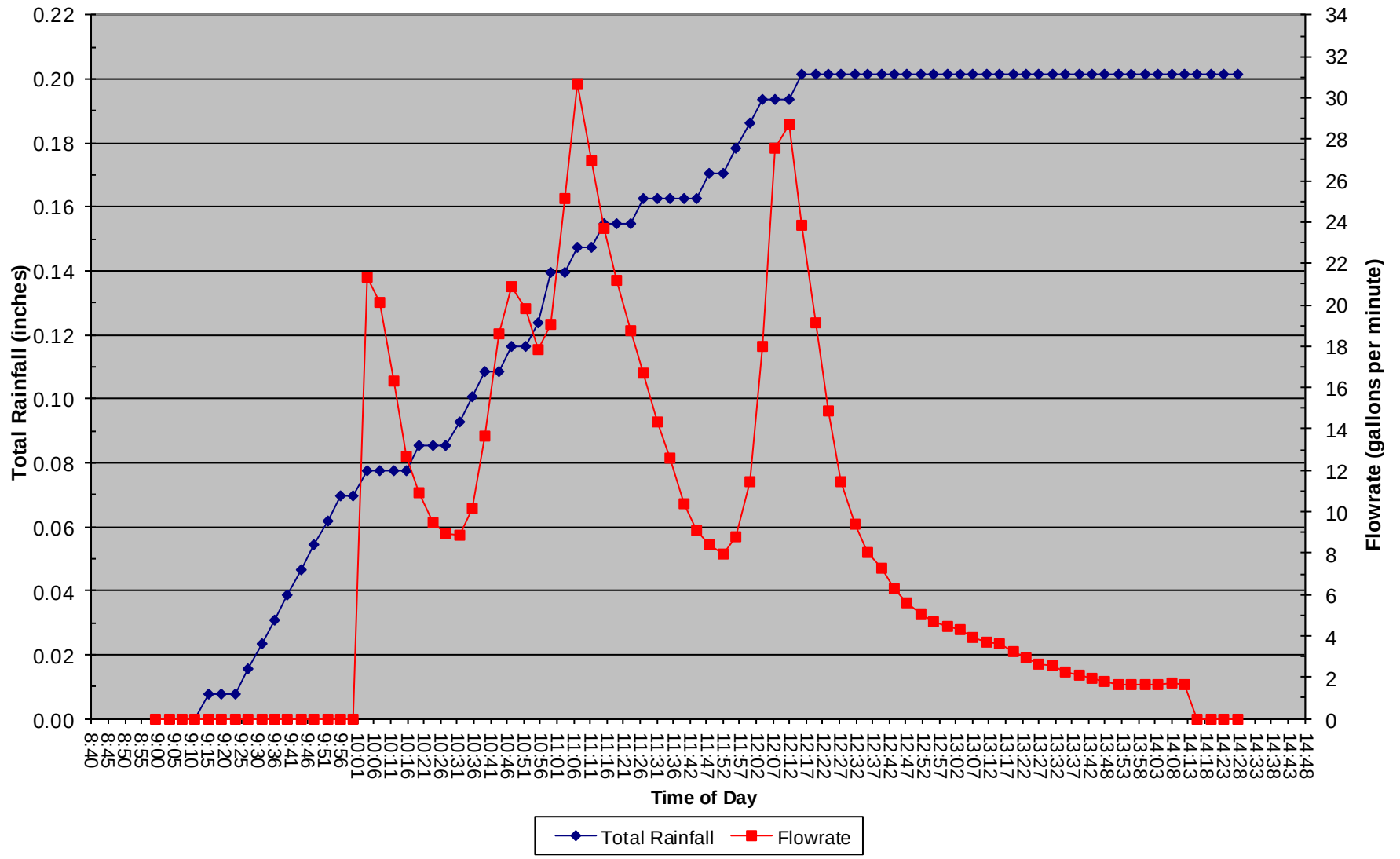
19 May 2019 Total Rainfall and Flowrate vs. Time of Day
