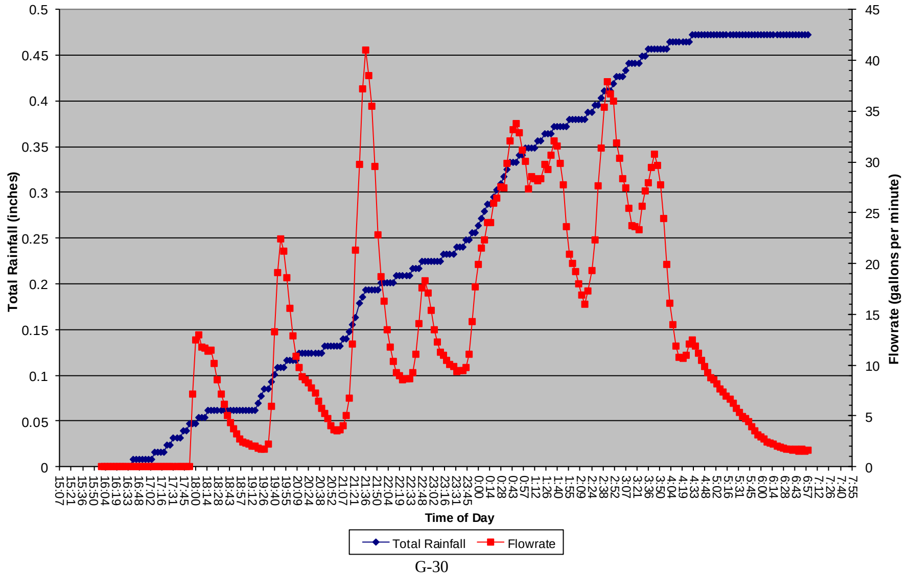
11 Mar 2019 Total Rainfall and Flowrate vs. Time of Day
