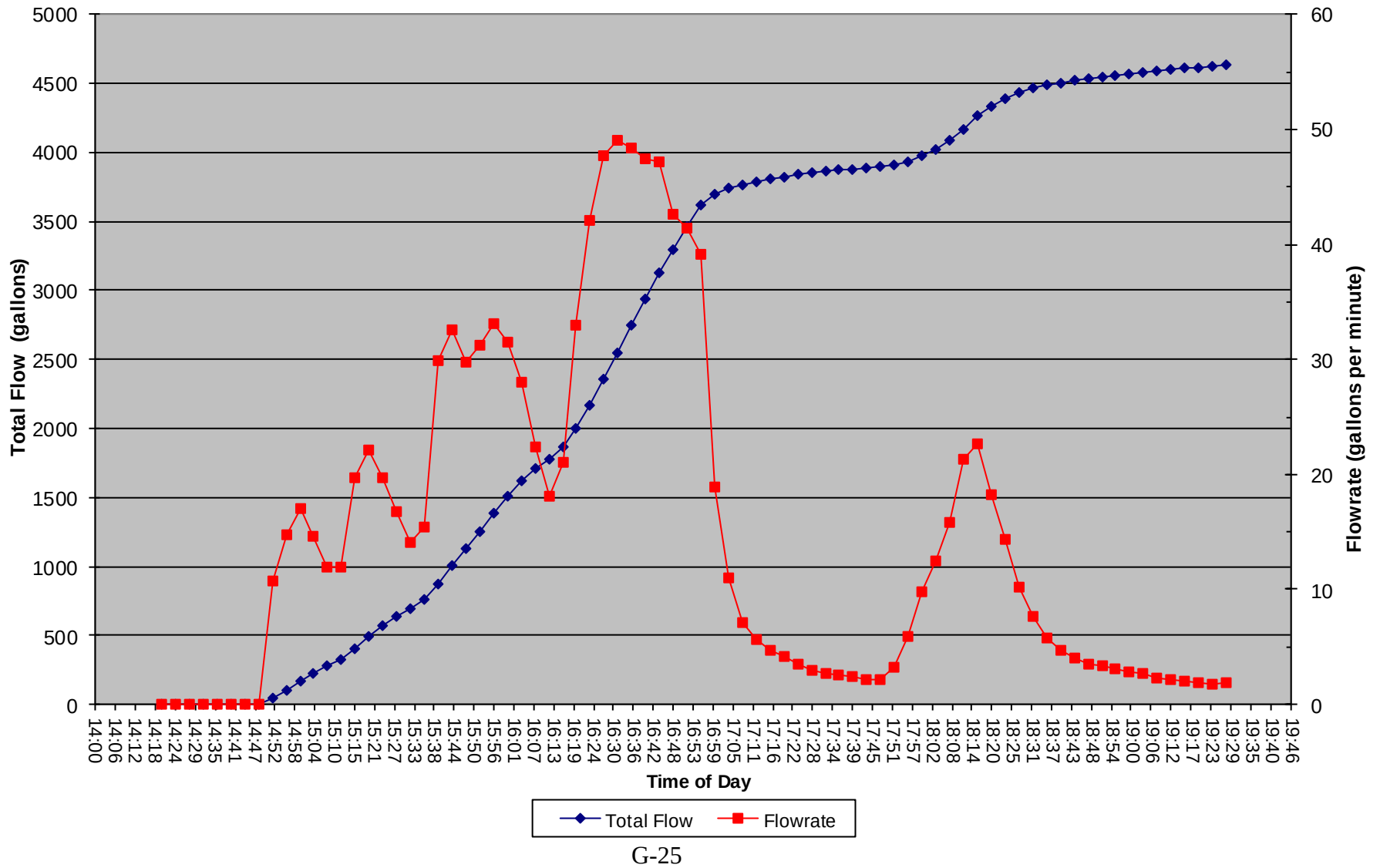
31 Jan 2019 Total Flow and Flowrate vs. Time of Day
