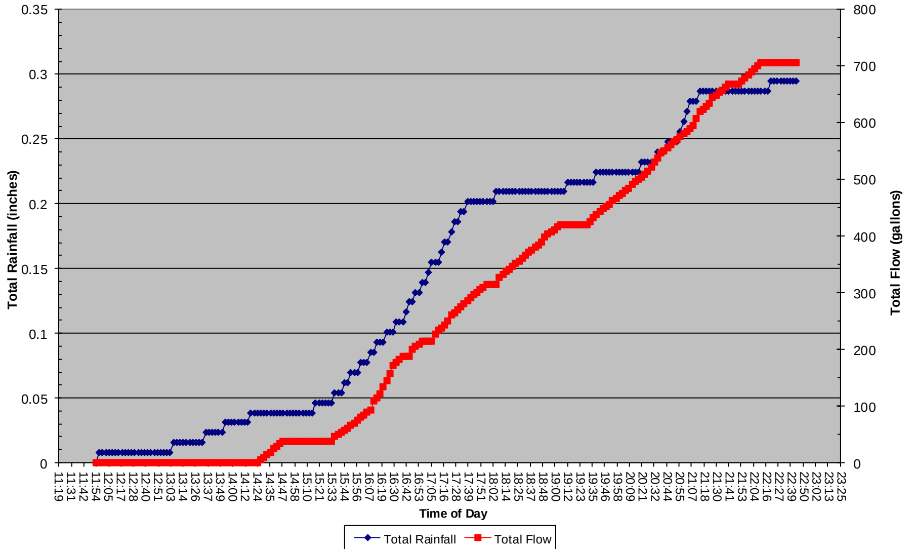
10 Mar 2018 Total Rainfall and Total Flow vs. Time of Day
