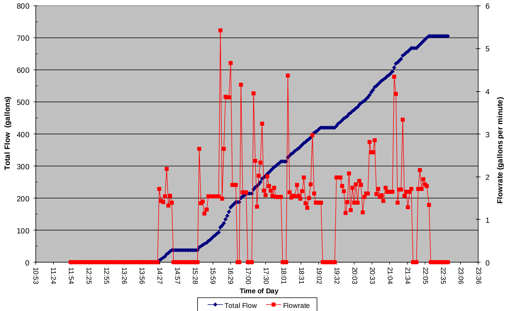
10 Mar 2018 Total Flow and Flowrate vs. Time of Day
