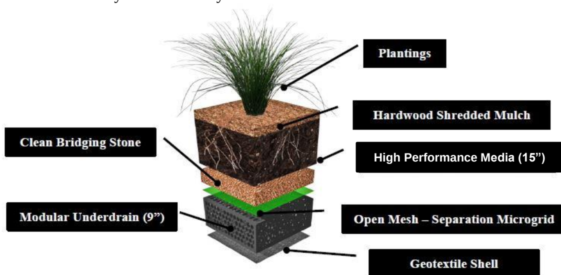
Figure 2-4. FocalPoint Biofilter Conceptual Diagram
