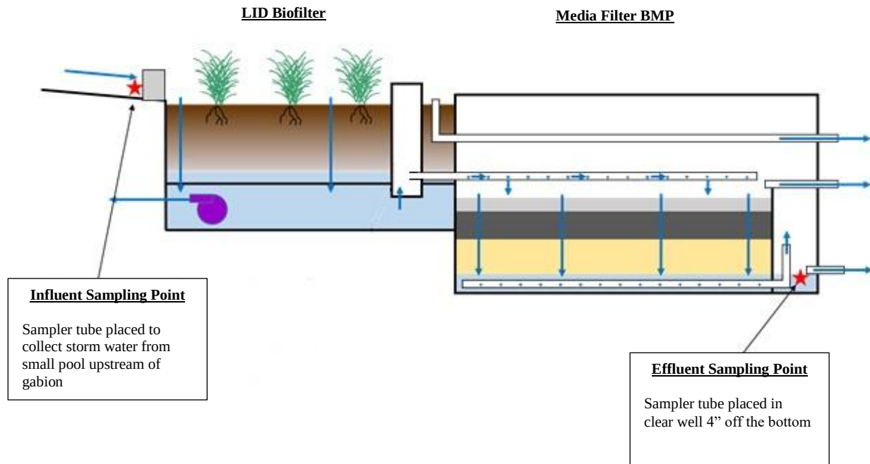
Figure 5-3. Layout of Water Quality Monitoring Equipment
