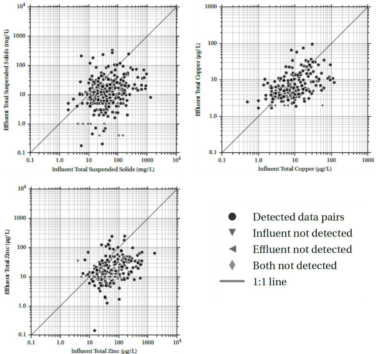
Figure 2-5. Paired Influent and Effluent Monitoring Data from the International Storm Water BMP Database For Bioretention BMPs
