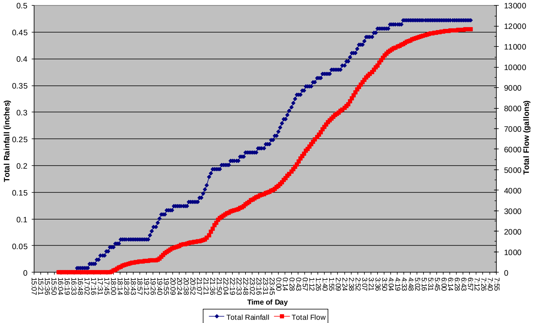
11 Mar 2019 Total Rainfall and Total Flow vs. Time of Day
