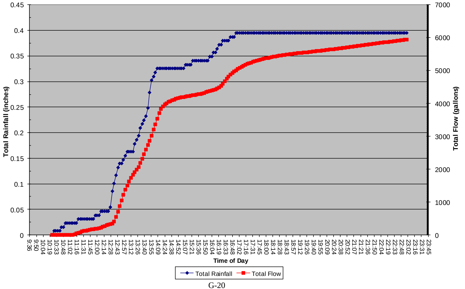
14 Jan 2019 Total Rainfall and Total Flow vs. Time of Day
