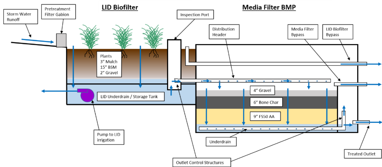
Figure 2-2. Conceptual Cross Section Diagram for Hybrid LID/BMP System
