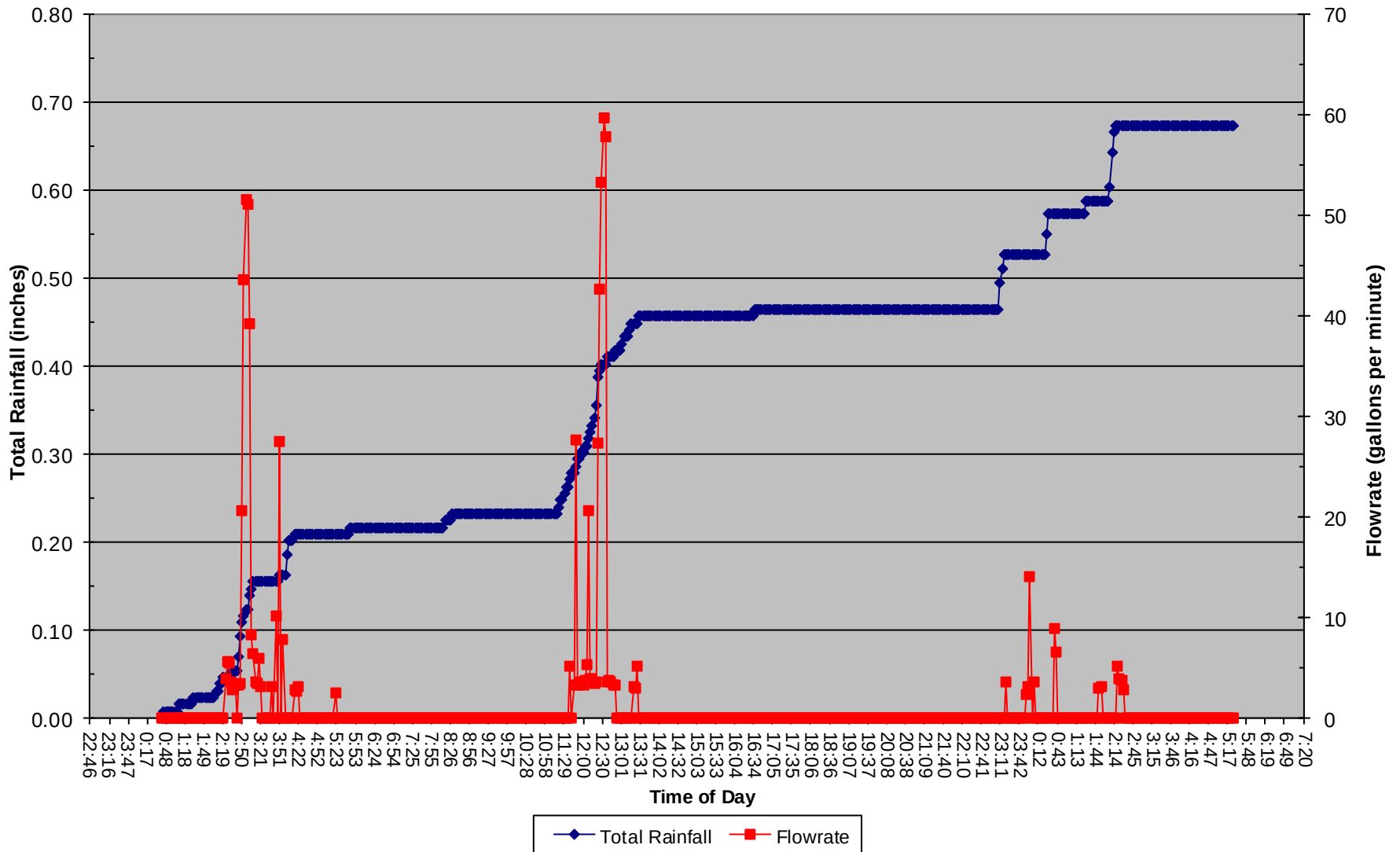
29 Nov 2018 Total Rainfall and Flowrate vs. Time of Day
