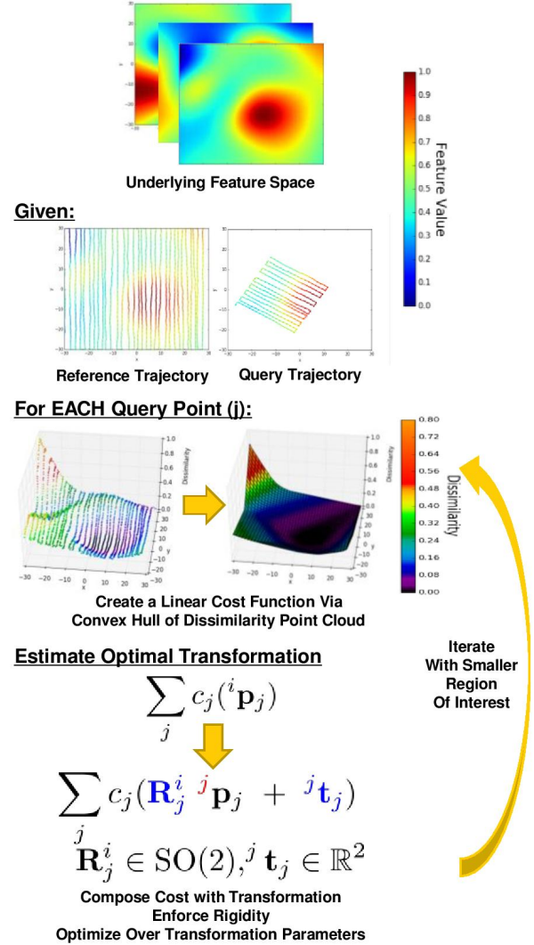
Fig. 1: An overview of the proposed trajectory alignment algorithm. Given sparse observations of an underlying feature space, we formulate a linear optimization problem that seeks to align a query trajectory with a reference trajectory. We do this by iteratively creating a linear cost that minimizes feature distance and optimizing over the transformation that minimizes that cost.
