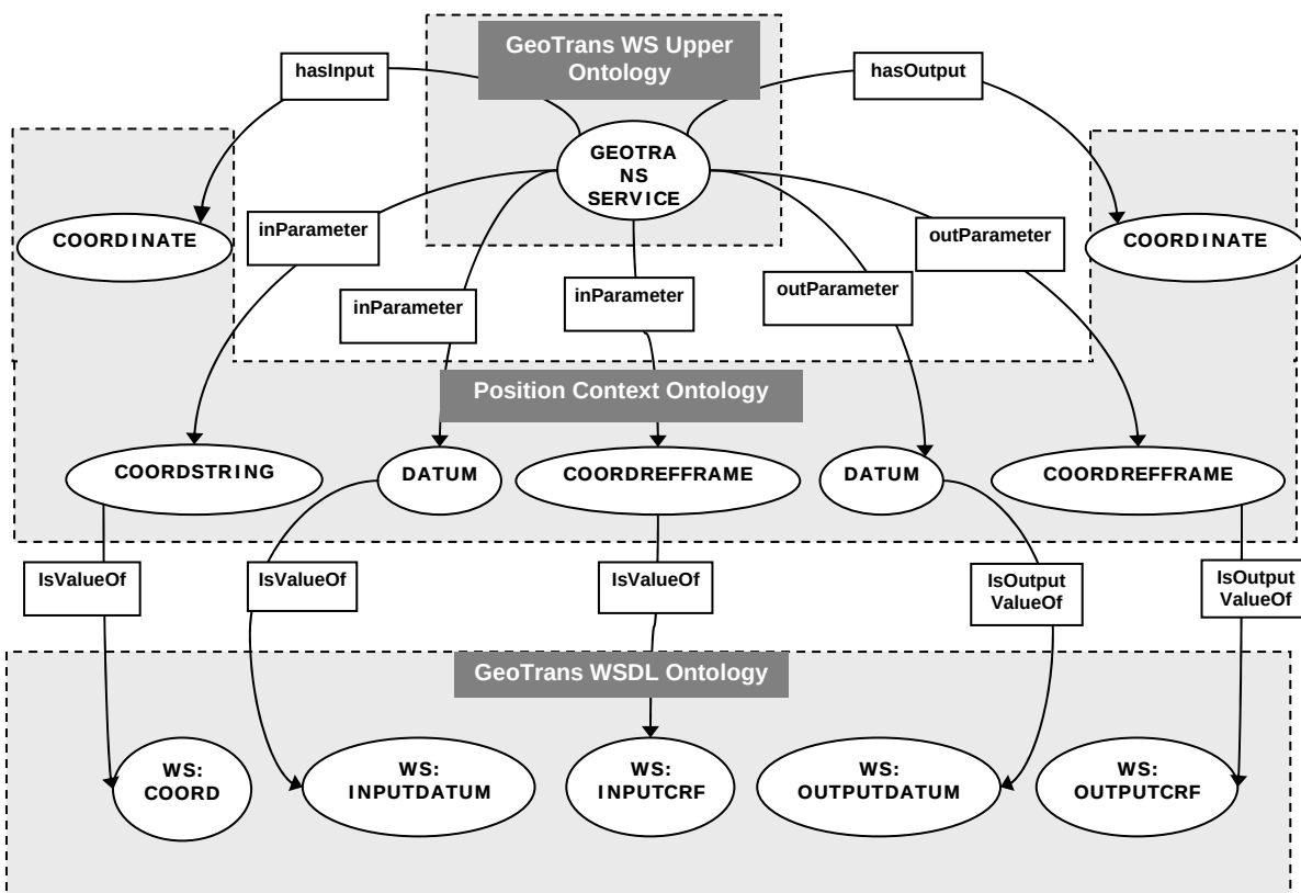
Fig. 7. Geo-Trans WSDL Ontology
