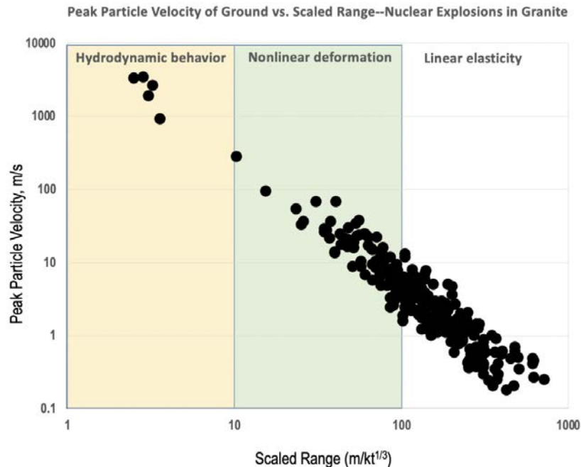
Figure 7. Peak Ground Particle Velocity for Underground Nuclear Explosions in Granite. Data from Perret and Bass (1975) and Xu et al. (2014).
