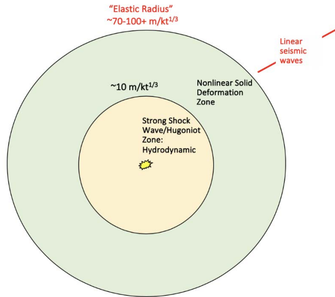
Figure 6. Deformation Regimes in the Vicinity of an Underground Nuclear Explosion
