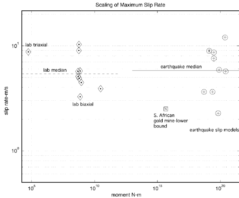
Figure 5. Peak Slip Rates Estimated for Various Earthquakes and Laboratory Stick-Slip Events. Maximum particle velocity is half of slip rate. From McGarr and Fletcher (2007).
