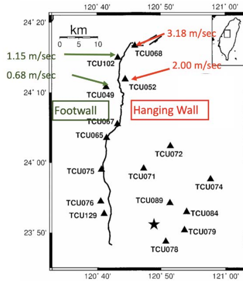
Figure 4. Locations of Instruments That Recorded High Ground Velocities near the Chelungpu Fault in Taiwan during the Chi-Chi Earthquake of 1999. Adapted from Chen et al. (2001).
