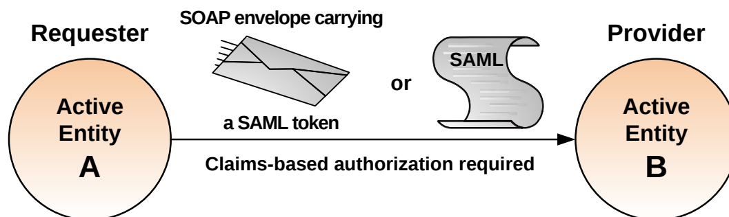
Figure 3. Claims-Based Authorization
