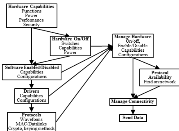
Figure 3 Mobile Ad Hoc Services and Dependencies
