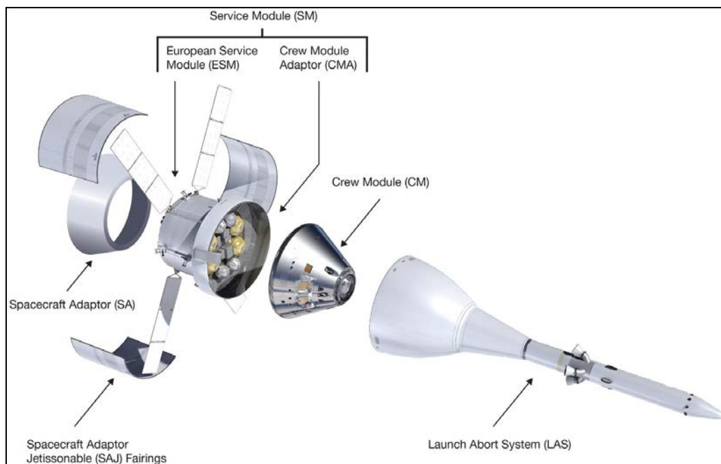
Figure 4. Components of the Orion Multi-Purpose Crew Vehicle
