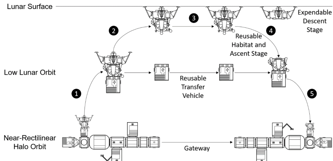
Figure 8. "Bat diagram" of the proposed lunar landing architecture with Gateway
