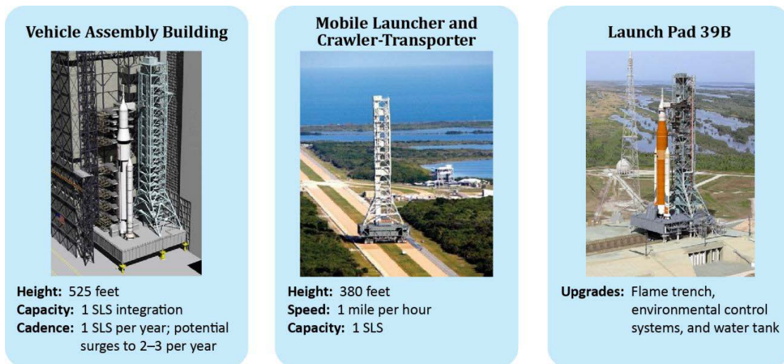
Figure 3. Key Components of EGS
