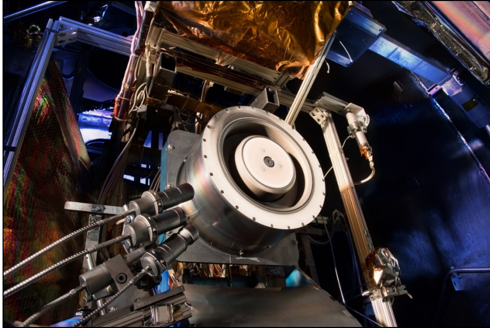
Figure 7. Hall Effect Rocket with Magnetic Shielding (HERMeS) Thruster to Be Used for the SEP system on the Gateway and DST Vehicles
