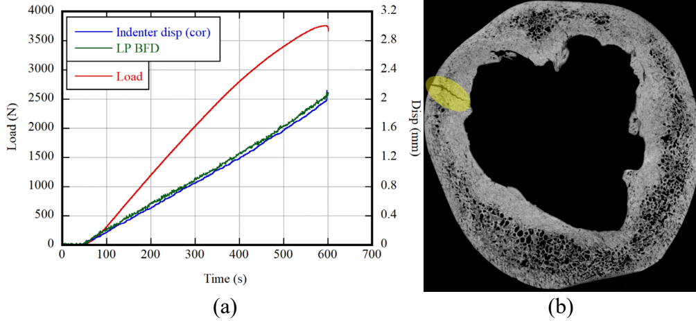
Fig. 17 (a) Load, corrected indenter displacement, and max inner surface BFD vs. time for LR07; (b) posttest micro-CT image with edge fracture highlighted
