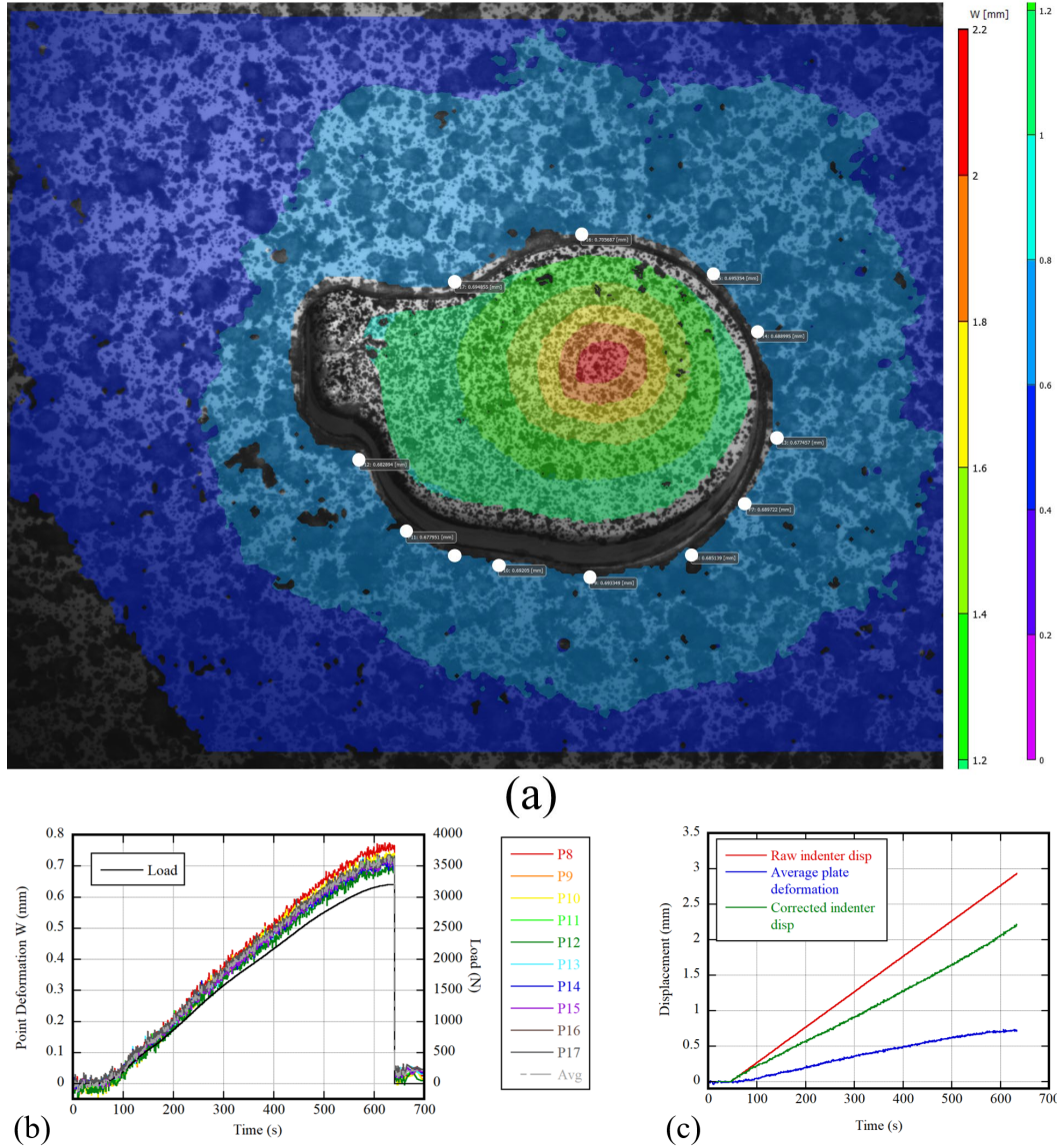
Fig. 7 For LR08 loading cycle 02: (a) backing plate out-of-plane deformation DIC contour with data points used for average plate deformation at time just prior to fracture, (b) variability of backing plate data points based on position around cutout edge, (c) raw and corrected indenter displacement, average plate deformation
