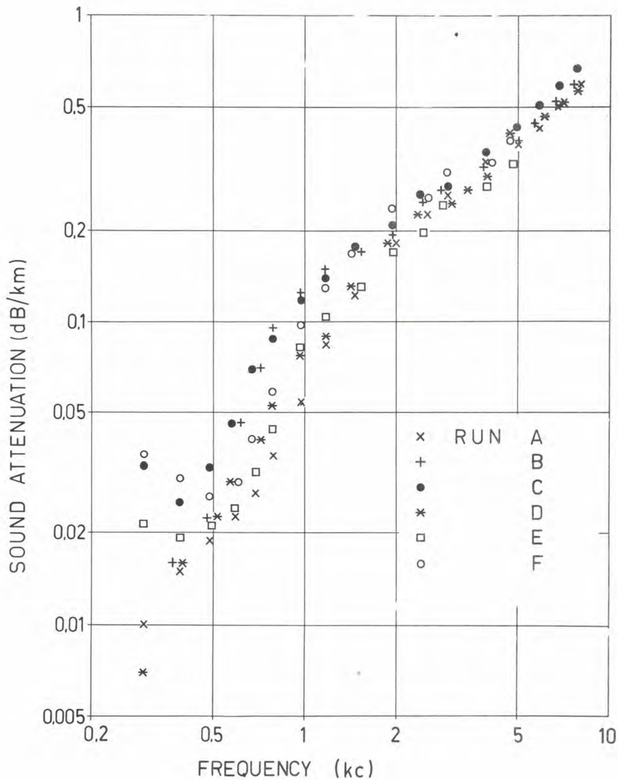
Fig. 9 - SOUND ATTENUATION vs FREQUENCY -- INDIVIDUAL RESULTS OF SIX RUNS.
