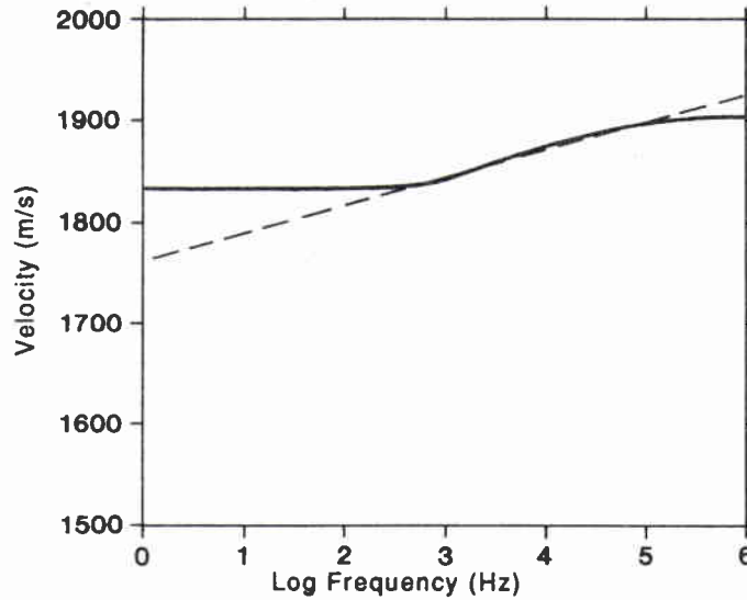
Fig. 4b. Velocity dispersion for the Biot model (solid curve) calculated with the parameters given in Table 1 and for the constant- Q model (broken curve) with Q = 50 .
