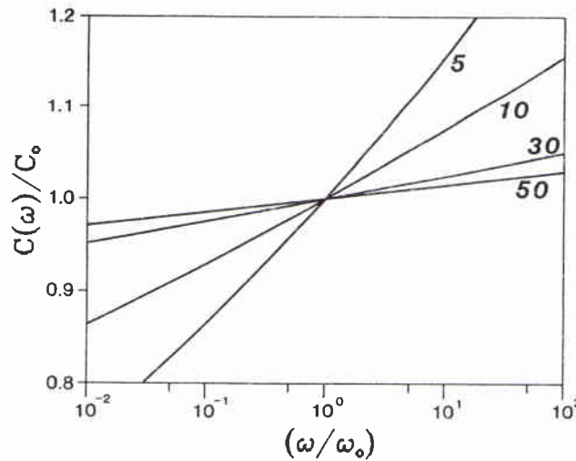
Fig. 1. Velocity dispersion for the constant- Q model for Q = 5, 10, 30, 50 .
