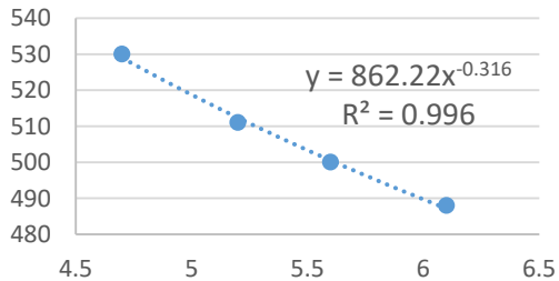
Oil Flow and Max Temp
