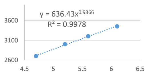
Oil Flow and Gallery1
