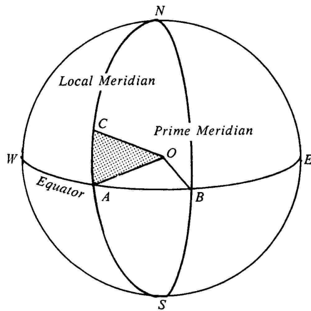
Figure 1 -- In this representation of the Earth, the North and South poles are at N and S, the equator is denoted by the arc WABE and the center of the Earth is at point O. Arc NCAS is the Local Meridian of the point C on the surface of the Earth; arc NBS is the Prime Meridian. Arc AC is the latitude of point C and is equal to the angle between the lines OC and OA. Arc BA is the longitude of point C and equal to the angle between the lines OB and OA.
